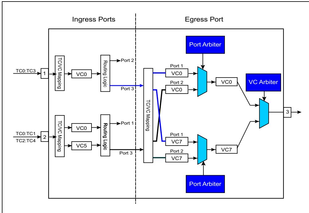
Figure 7-16: Port Arbitration Buffering
