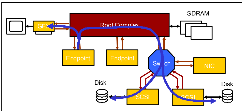
Figure 20-1: Multicast System Example
