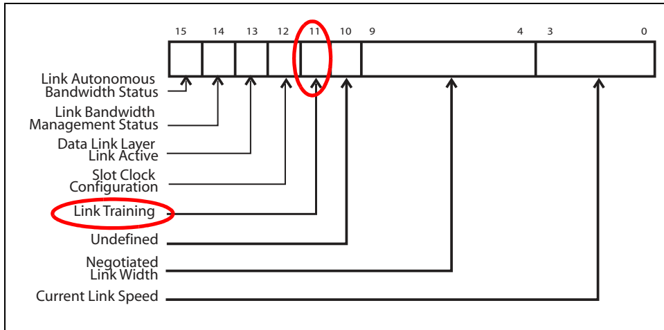
Figure 15-20: Link Training Status in the Link Status Register
