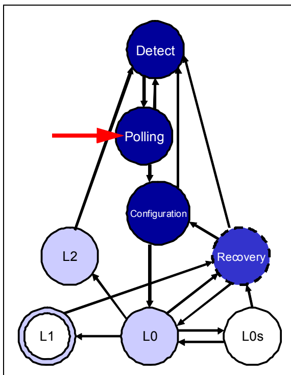
Figure 14-45: LTSSM Overview
