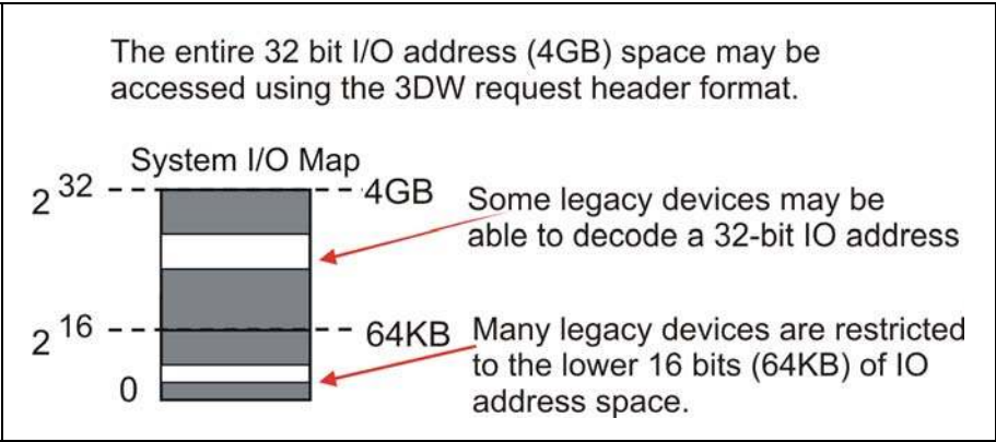
Figure 5-6: System IO Map
