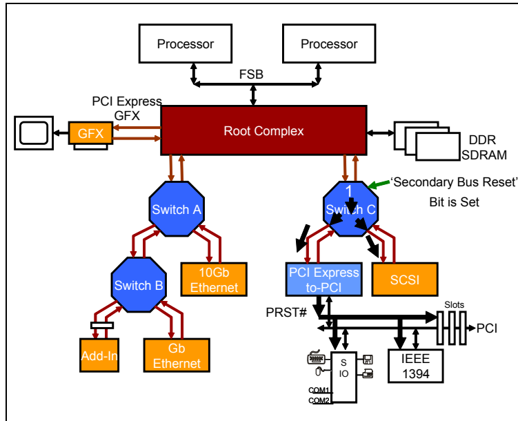
Figure 18-4: Switch Generates Hot Reset on All Downstream Ports
