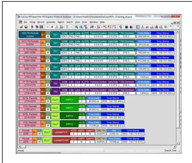
Figure A-9: “Compact View” Collapses Related Packets for Easy Viewing of Link Training
