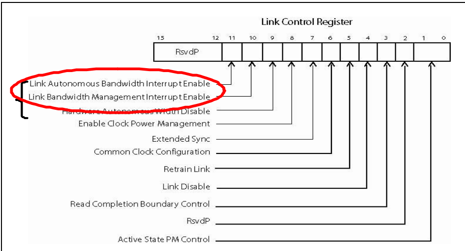
Figure 14-54: Bandwidth Change Notification Bits
