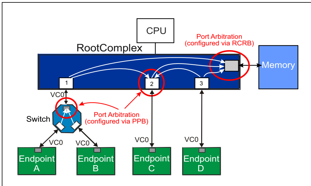
Figure 7-14: Port Arbitration Concept
