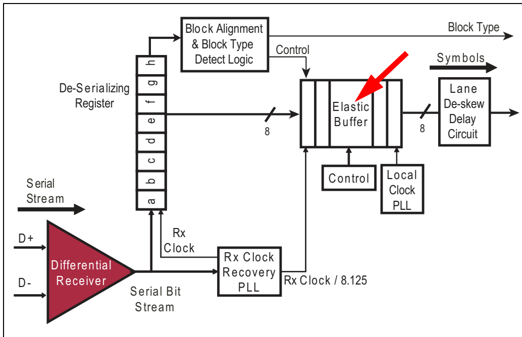
Figure 12-21: Gen3 Elastic Buffer Logic
