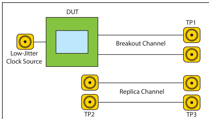
Figure 13-10: Test Circuit Measurement Channels
