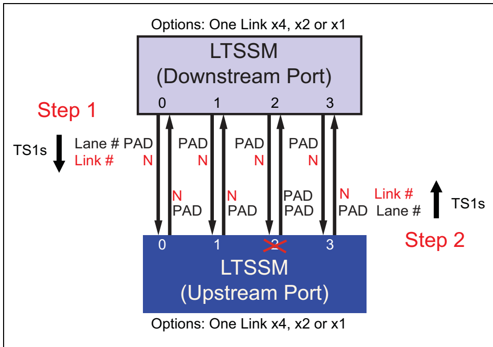
Figure 14-21: Example 3 - Steps 1 and 2
