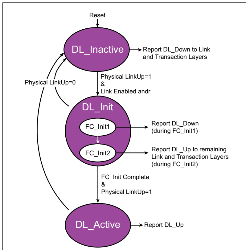
Figure 6-4: The Data Link Control & Management State Machine
