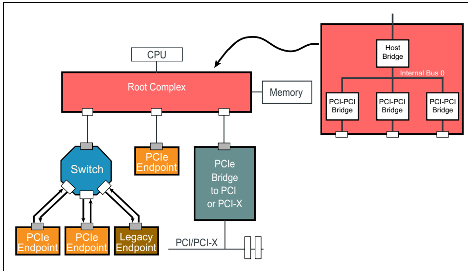
Figure 2-8: Topology Example
