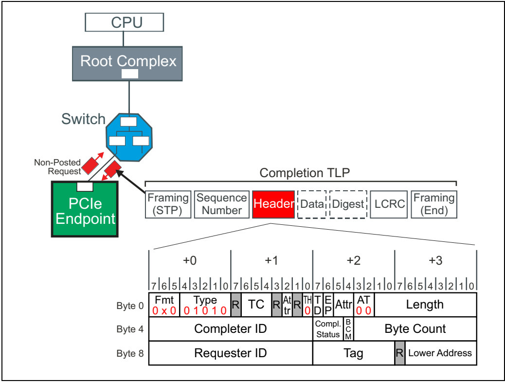
Figure 5-10: 3DW Completion Header Format
