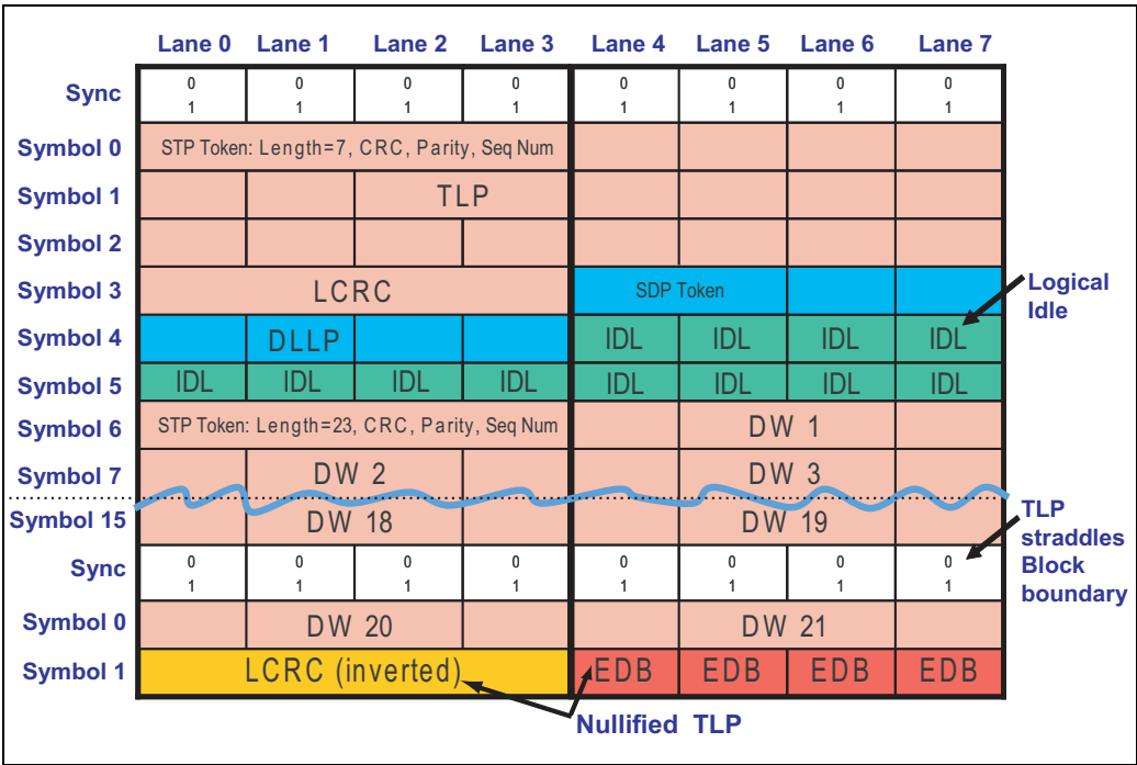
Figure 12-13: Gen3 x8 Nullified Packet
