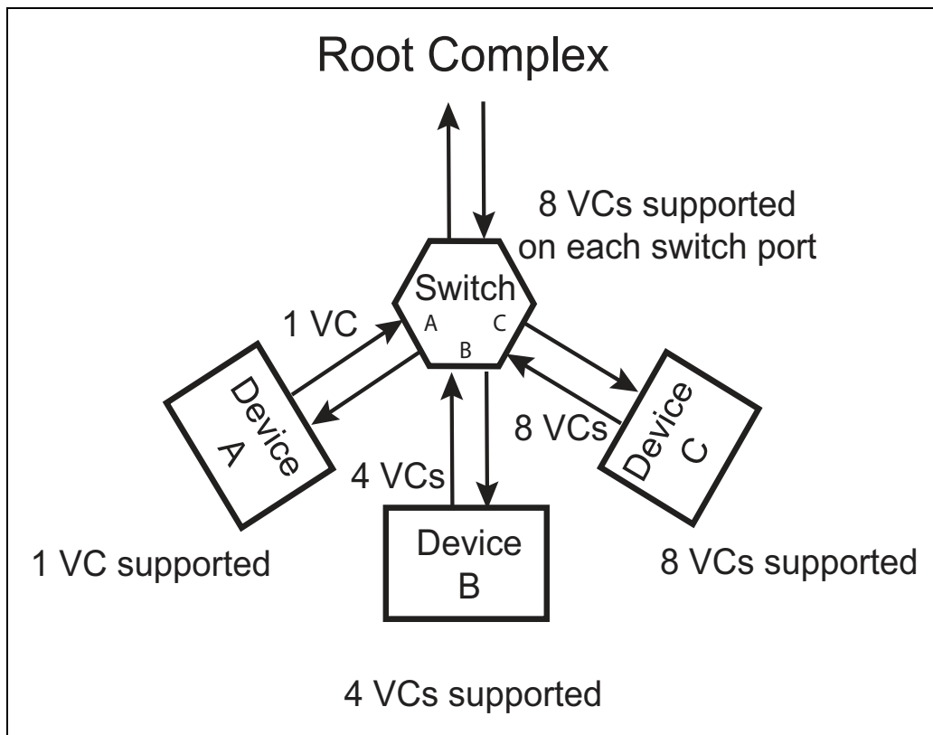
Figure 7-4: Multiple VCs Supported by a Device
