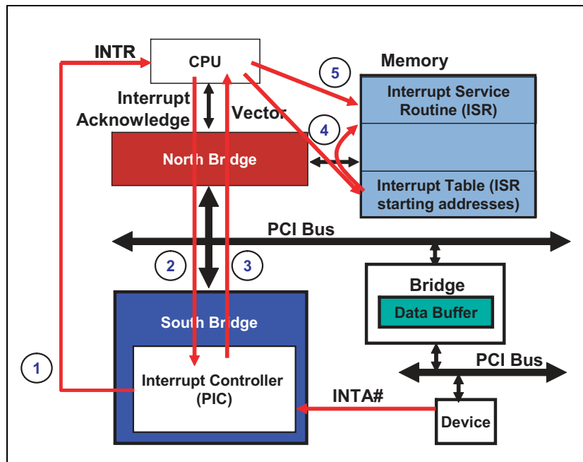
Figure 17-3: Legacy Interrupt Example
