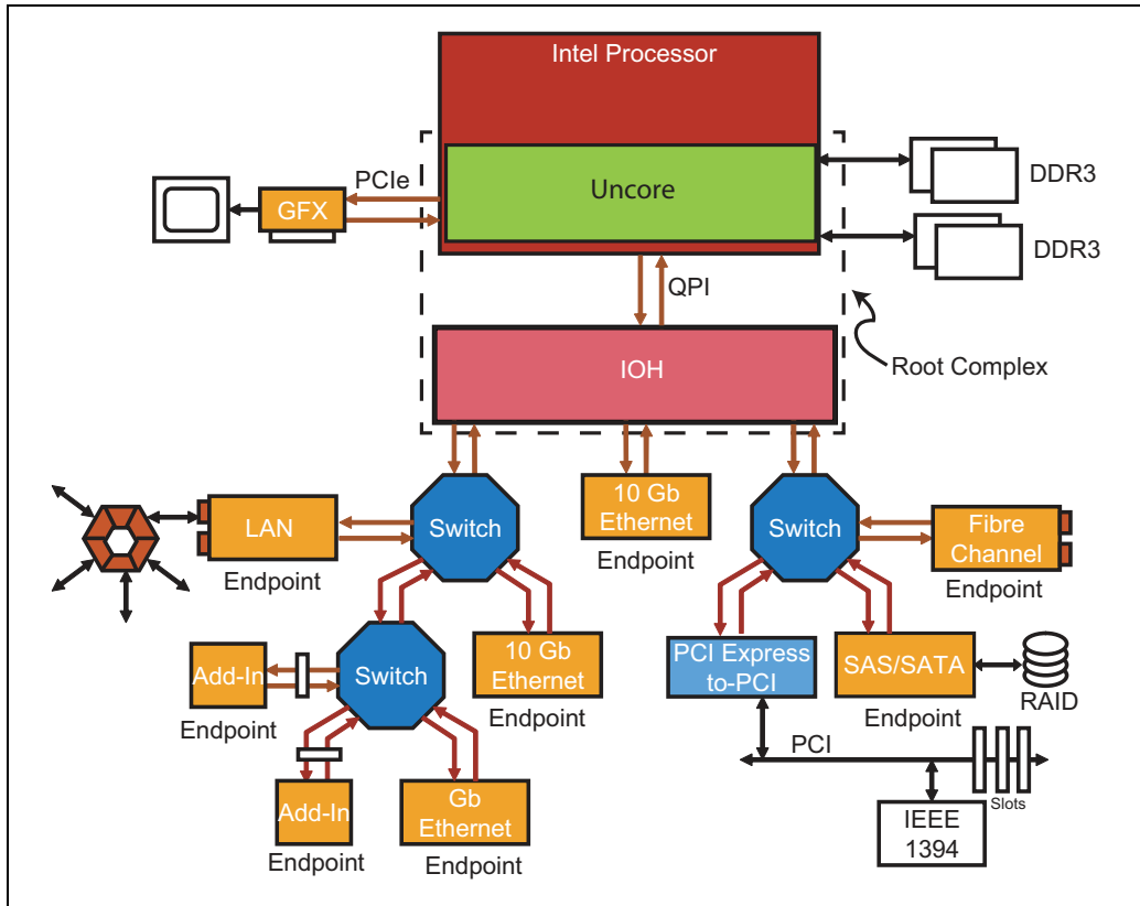
Figure 2-11: Server PCIe System
