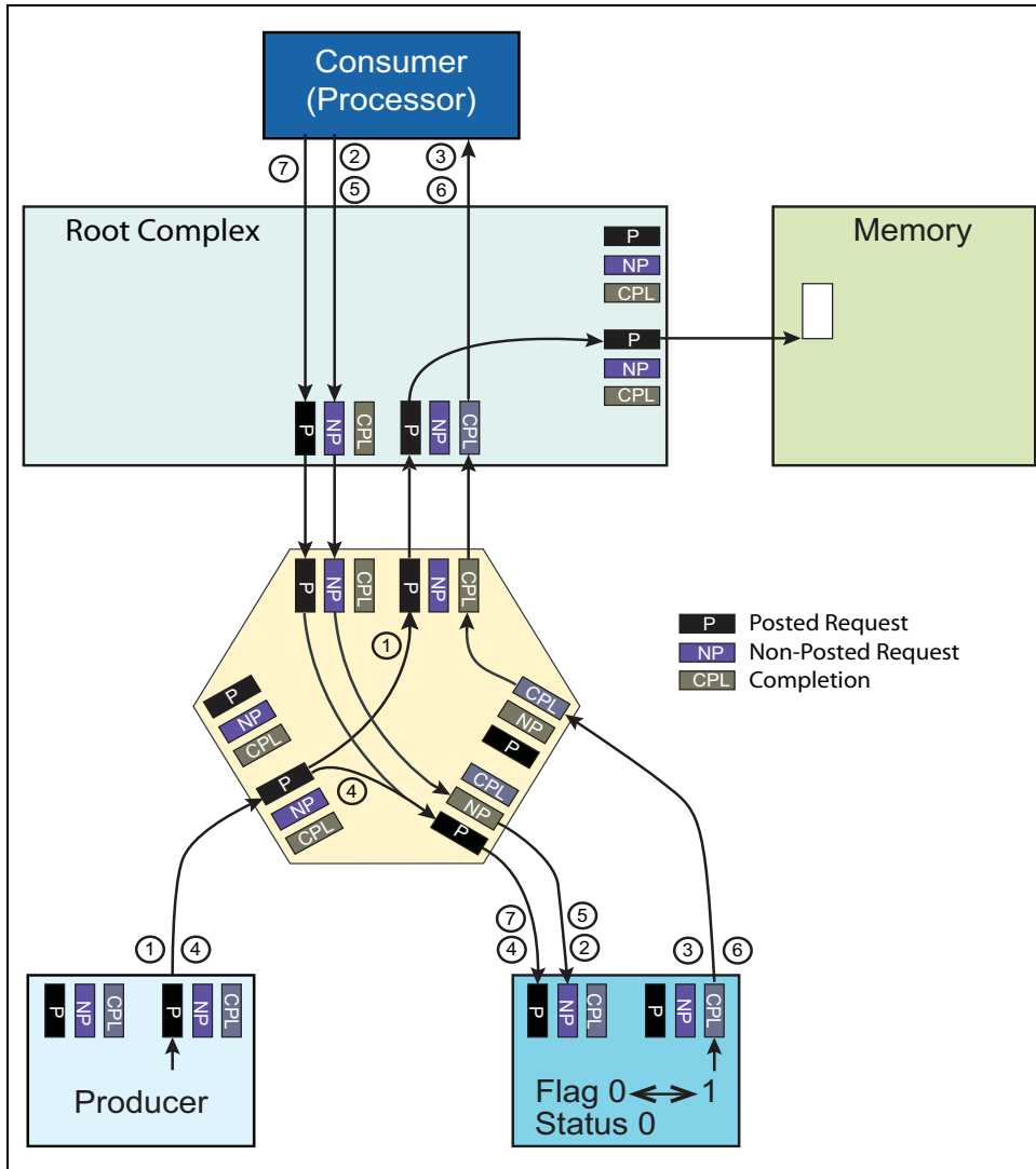
Figure 8-2: Producer/Consumer Sequence Example — Part 1
