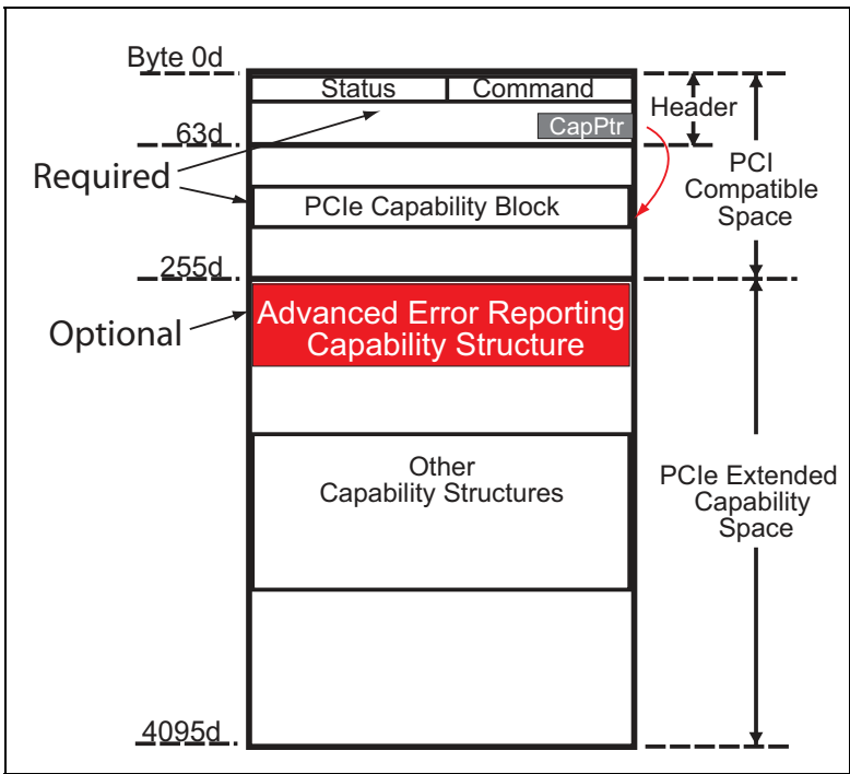
Figure 15-4: Location of Error-Related Configuration Registers
