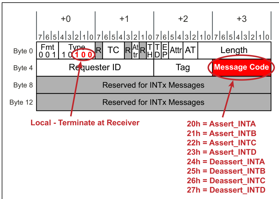
Figure 17-10: INTx Message Format and Type
