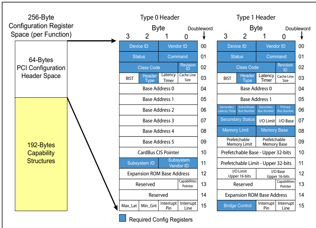
Figure 3-2: PCI Compatible Configuration Register Space
