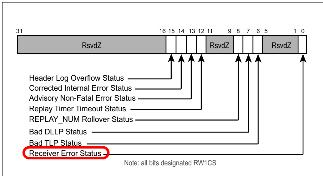
Figure 12-9: AER Correctable Error Register
