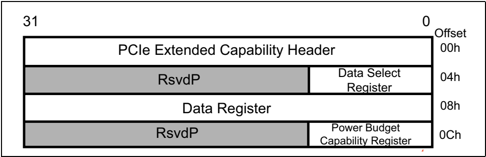
Figure 19-12: Power Budget Capability Registers
