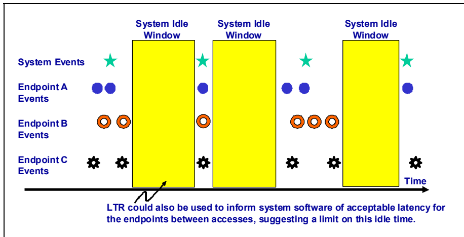
Figure 16-32: Improved System Idle Time
