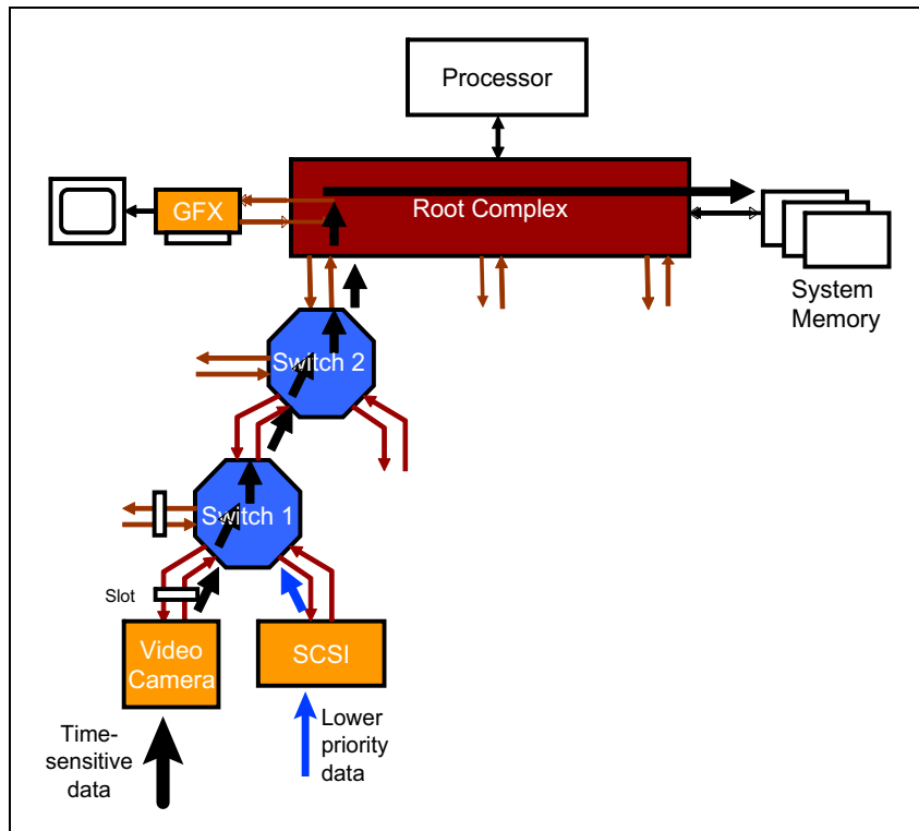
Figure 7-24: Example Isochronous System
