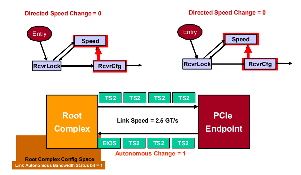
Figure 14-51: Speed Change - Part 3
