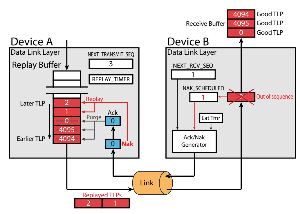
Figure 10-13: Handling Lost TLPs
