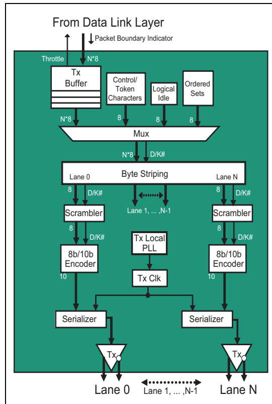
Figure 11-5: Physical Layer Transmit Logic Details (Gen1 and Gen2 Only)
