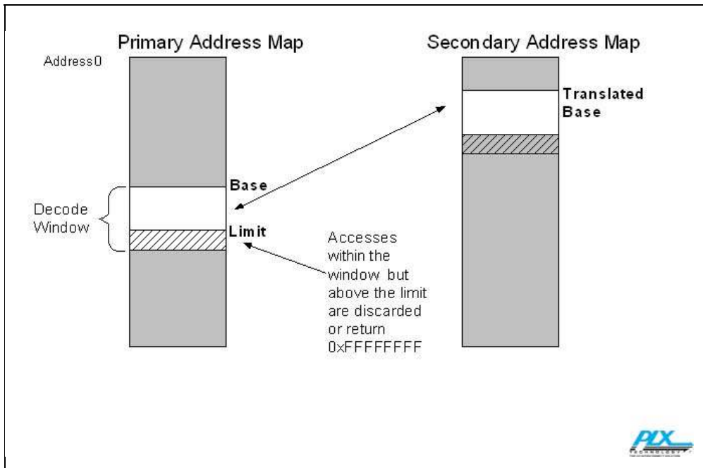
Figure 0-10: Use of Limit Register
