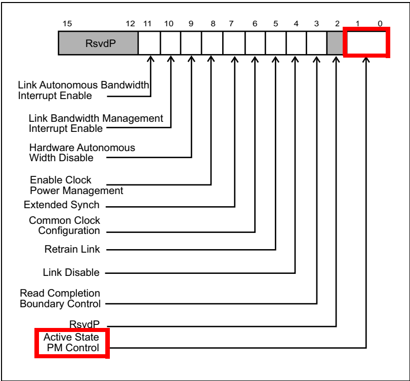
Figure 16-15: Active State PM Control Field
