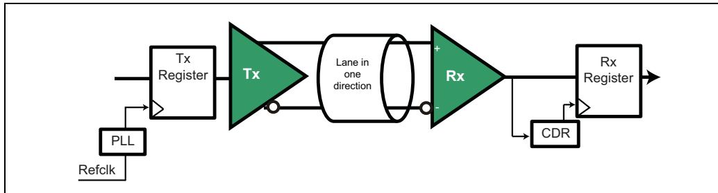
Figure 13-8: Data Clocked Rx Architecture
