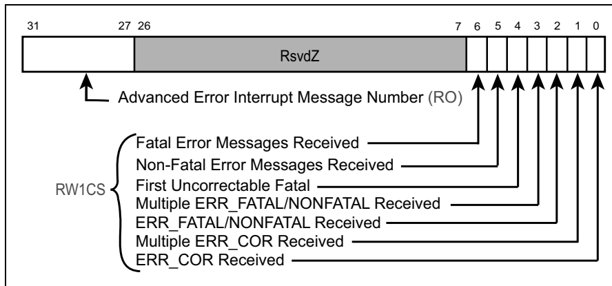
Figure 15-28: Root Error Status Register
