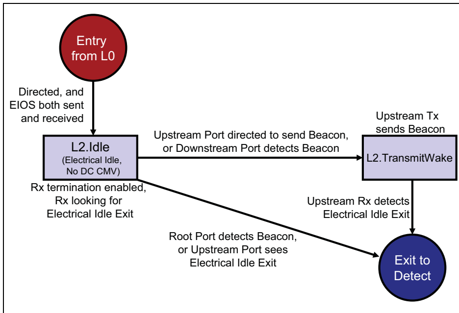
Figure 14-43: L2 State Machine
