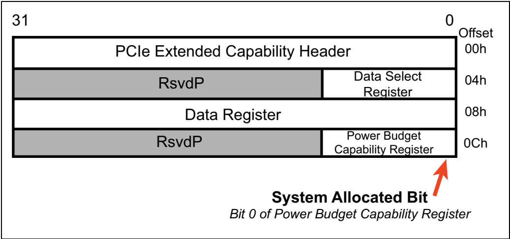
Figure 19-9: Power Budget Registers
