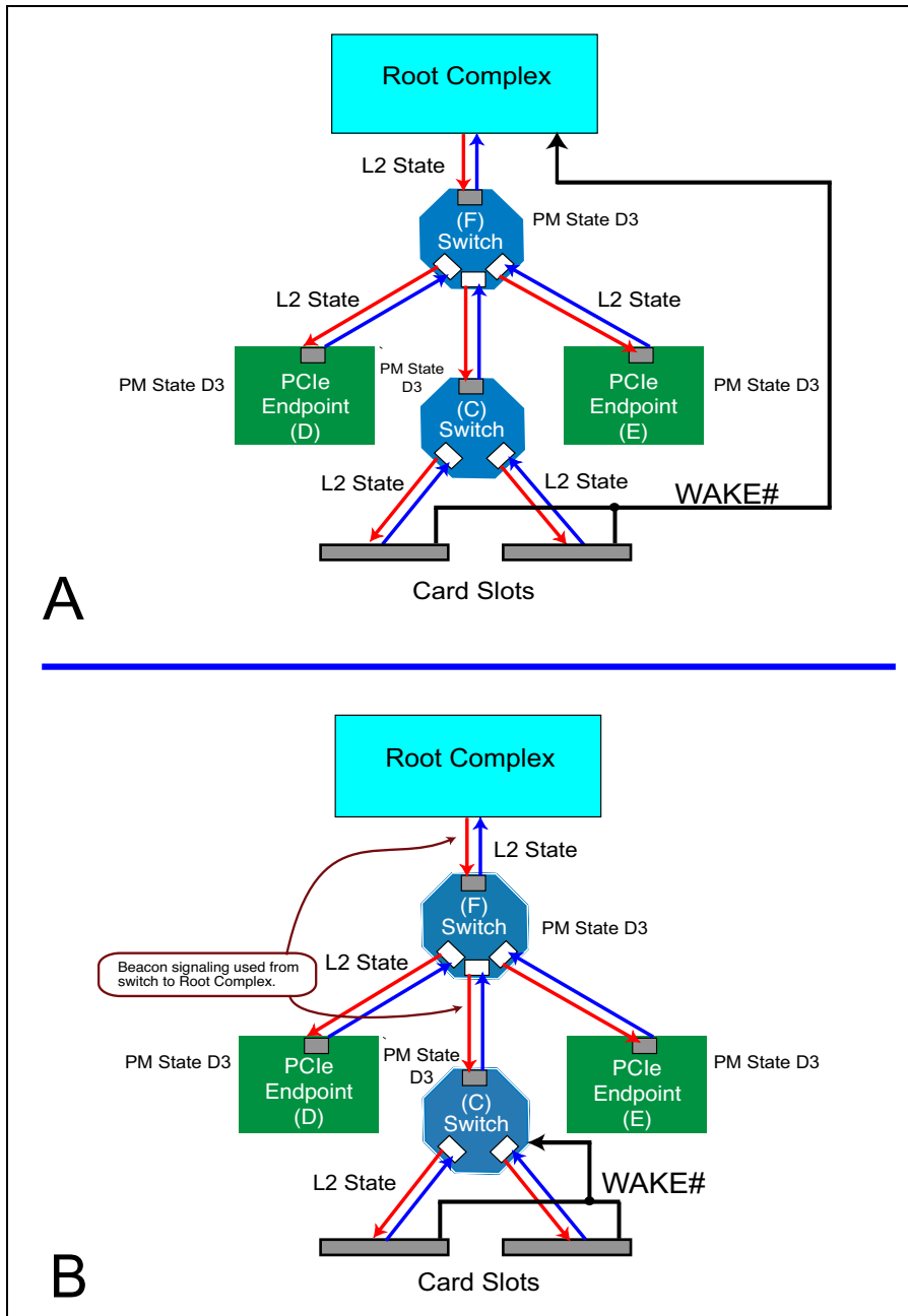
Figure 16-29: WAKE# Signal Implementations
