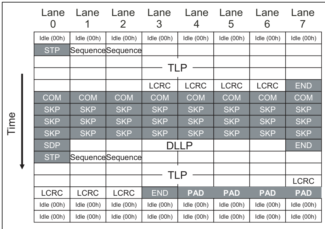
Figure 11-13: x8 Packet Format
