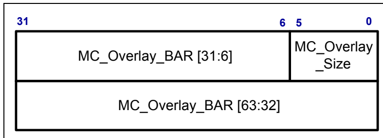
Figure 20-8: Multicast Overlay BAR
