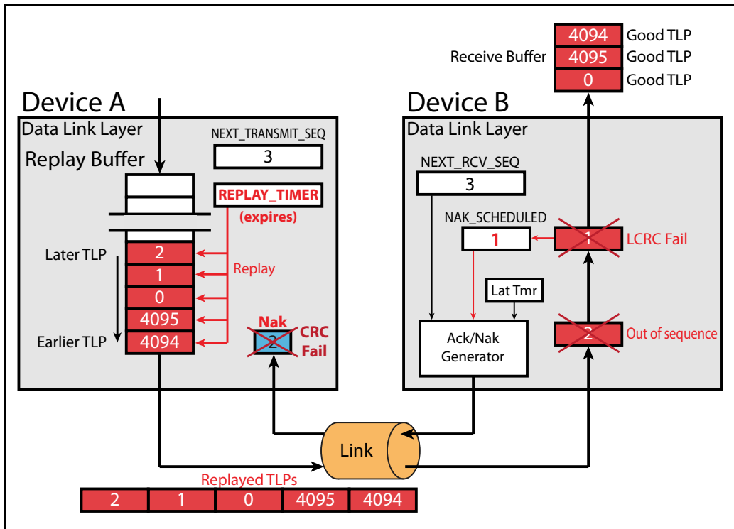
Figure 10-15: Handling Bad Nak
