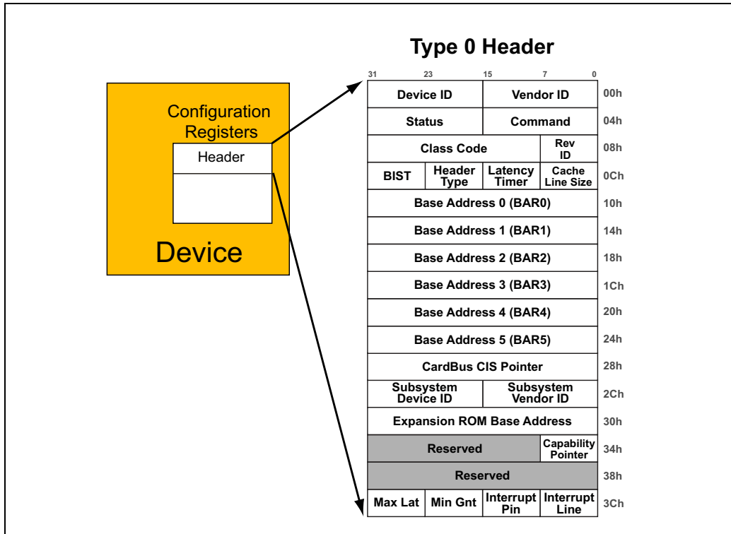
Figure 1-13: PCI Configuration Header Type 0 (not a Bridge)
