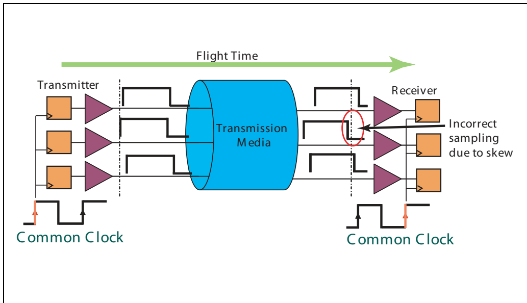
Figure 1-18: Inherent Problems in a Parallel Design
