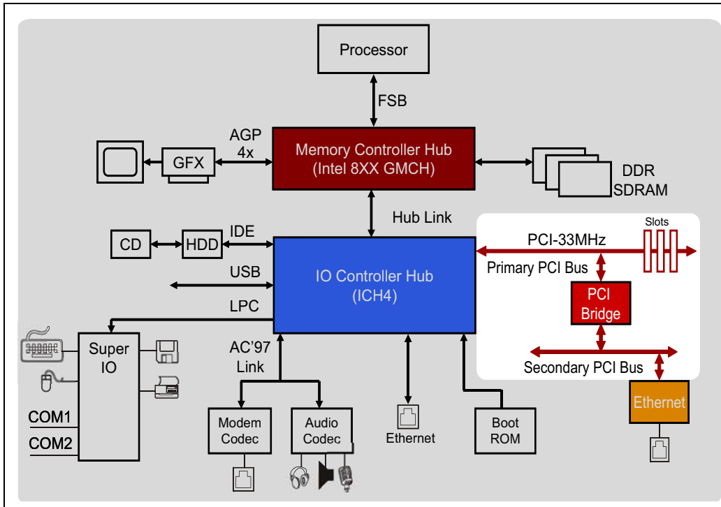
Figure 1-5: 33 MHz PCI System, Including a PCI-to-PCI Bridge
