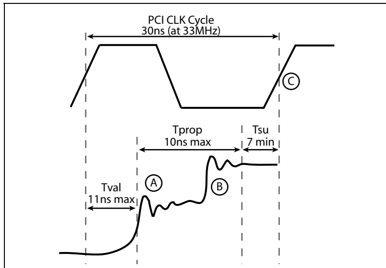
Figure 1-4: PCI Reflected-Wave Signaling
