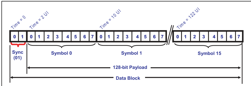
Figure 12-3: Sync Header Data Block Example
