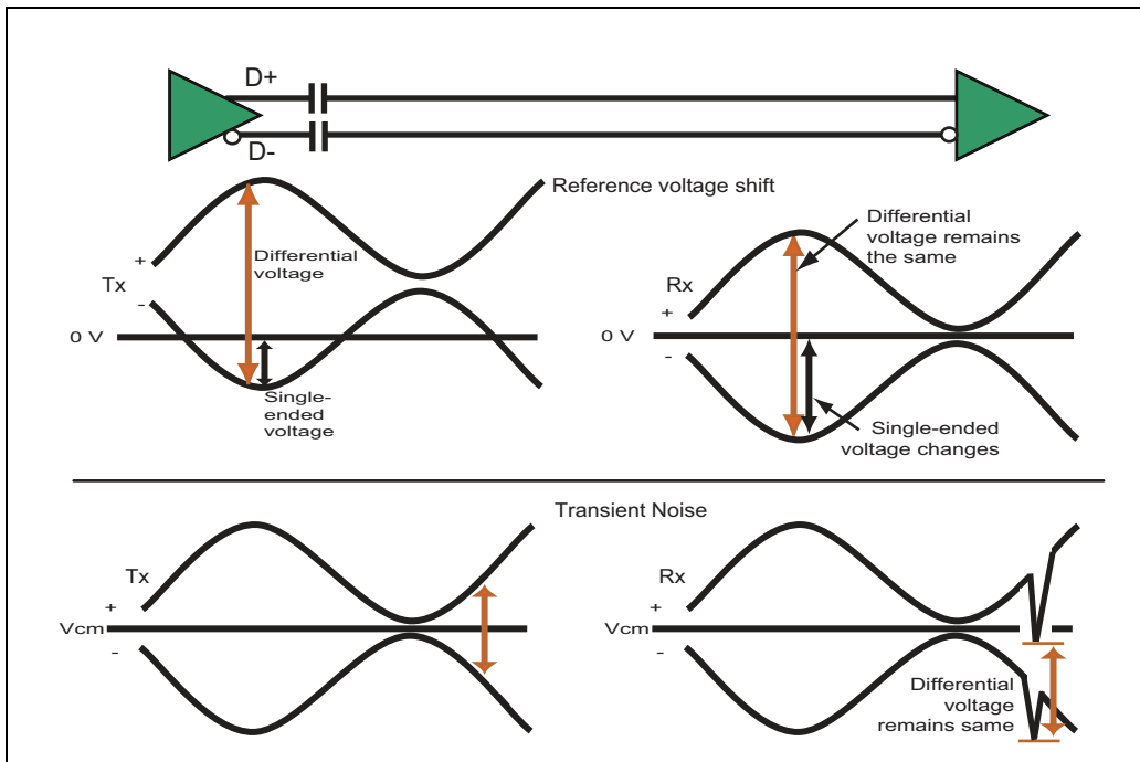
Figure 13-3: Differential Common-Mode Noise Rejection
