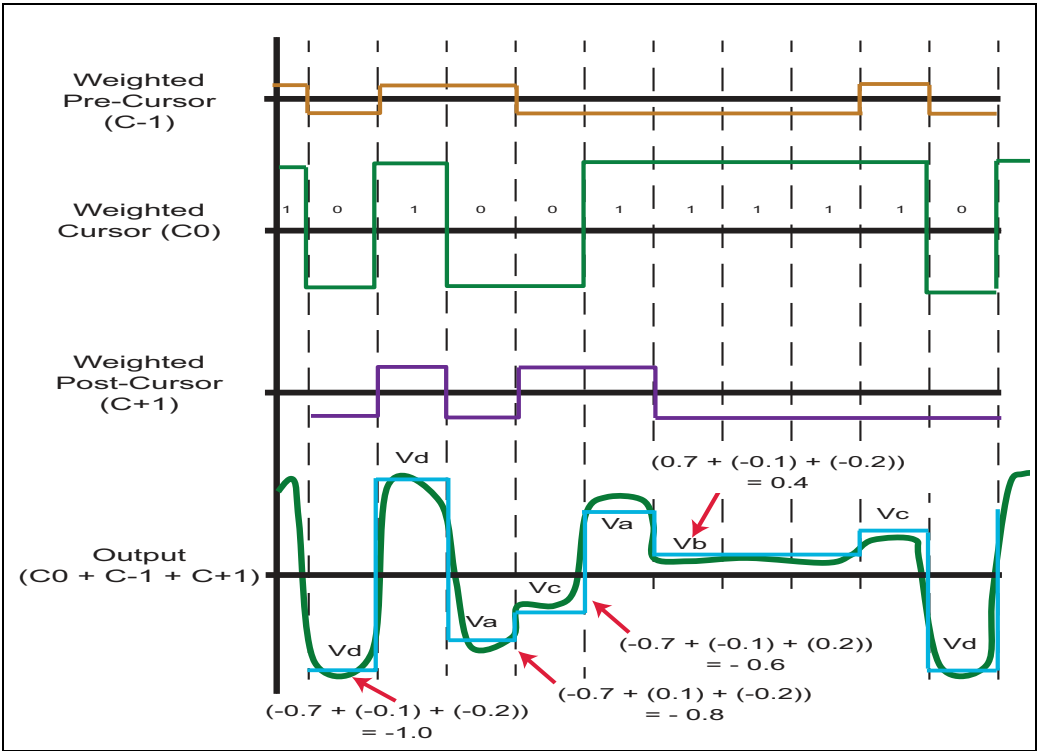
Figure 13-24: Tx 3-Tap Equalizer Output
