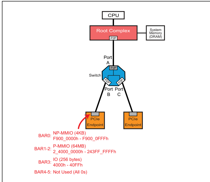
Figure 4-7: Example Topology for Setting Up Base and Limit Values
