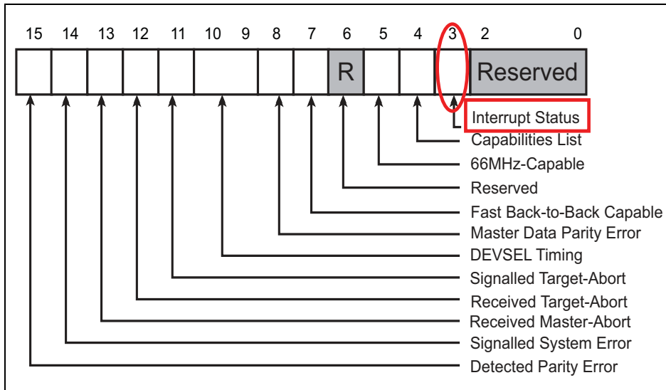
Figure 17-8: Configuration Status Register — Interrupt Status Field
