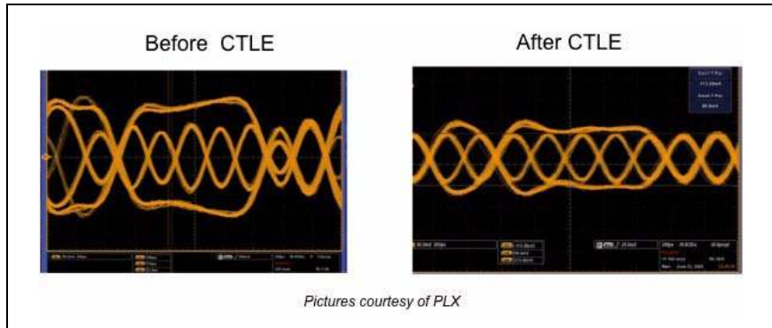
Figure 13-31: Effect of Rx Continuous-Time Linear Equalizer (CTLE) on Received Signal
