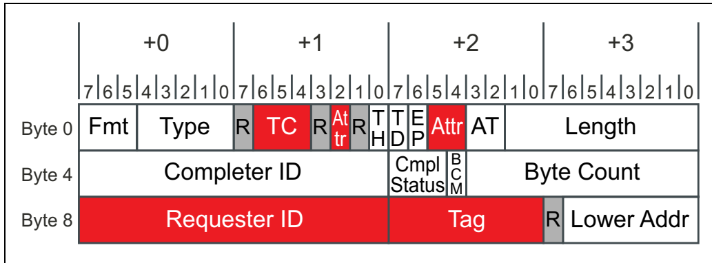
Figure 5-5: Transaction Descriptor Fields
