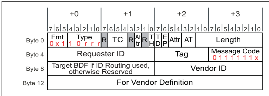
Figure 5-12: Vendor-Defined Message Header
