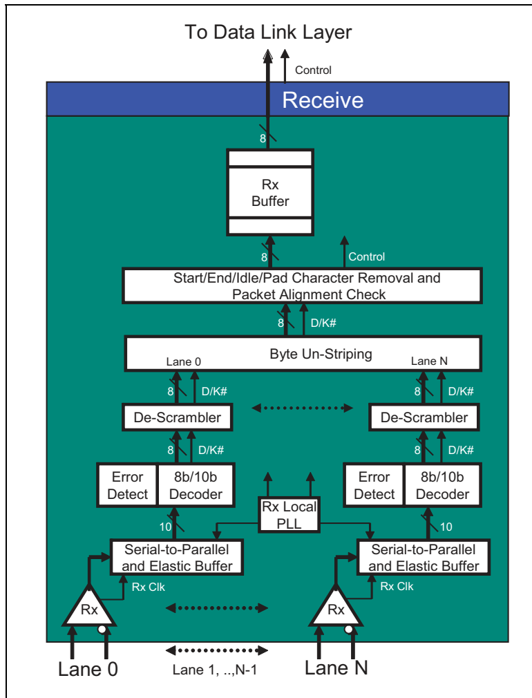
Figure 11-21: Physical Layer Receive Logic Details (Gen1 and Gen2 Only)
