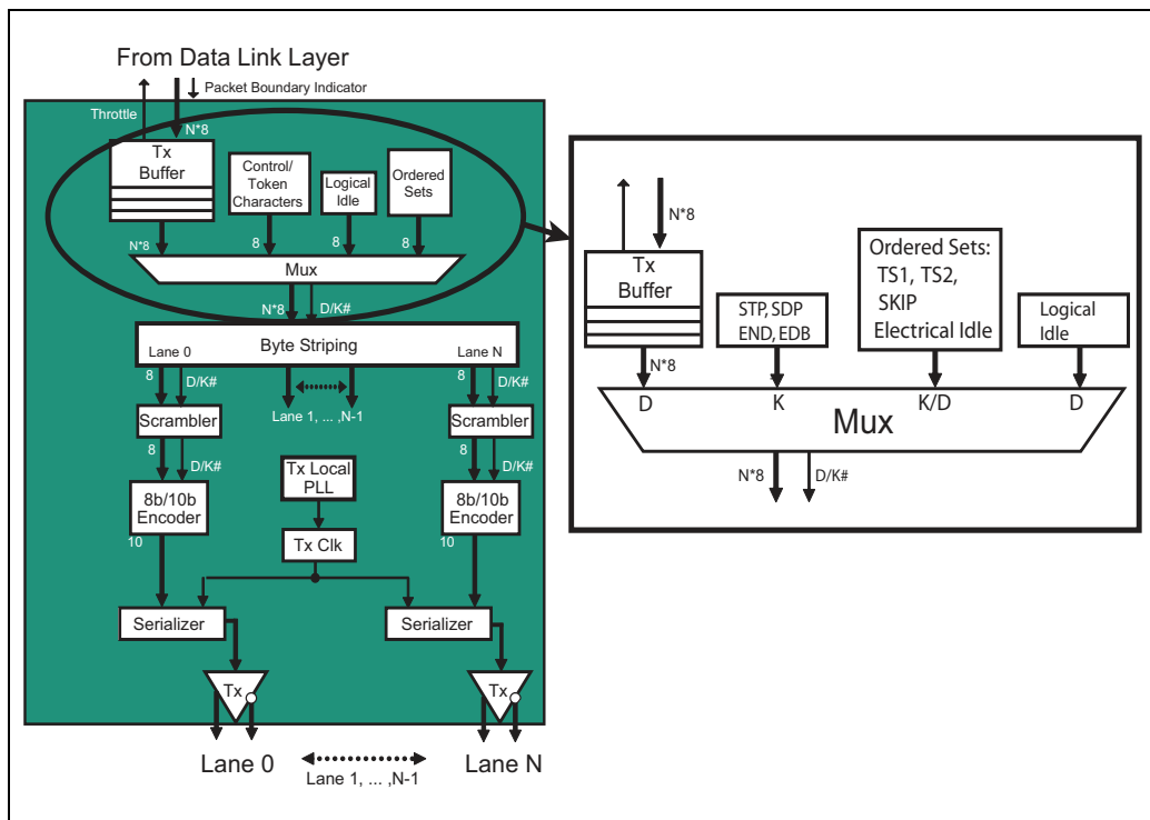
Figure 11-6: Transmit Logic Multiplexer
