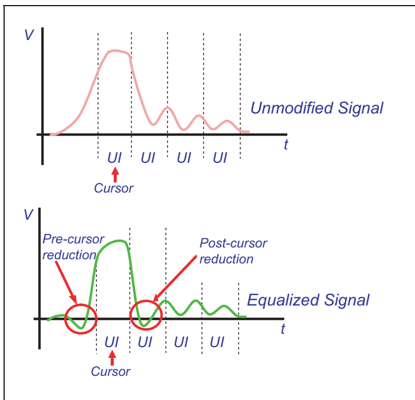
Figure 13-22: Tx 3-Tap Equalizer Shaping of an Output Pulse
