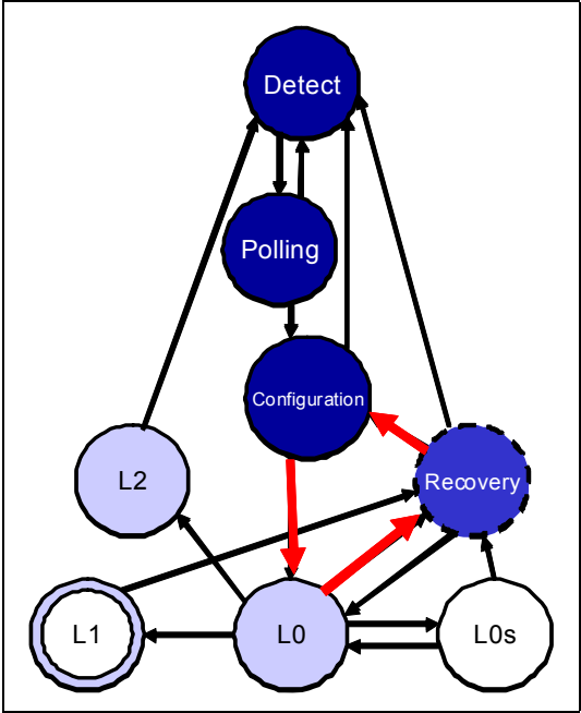
Figure 14-60: Link Width Change LTSSM Sequence
