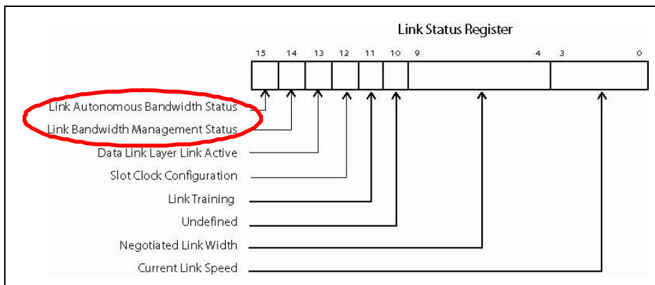
Figure 14-52: Bandwidth Change Status Bits
