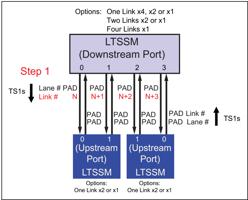
Figure 14-18: Example 2 - Step 1
