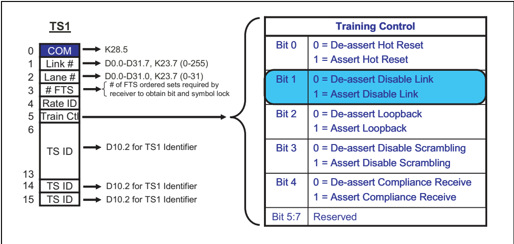
Figure 18-7: TS1 Ordered-Set Showing Disable Link Bit
