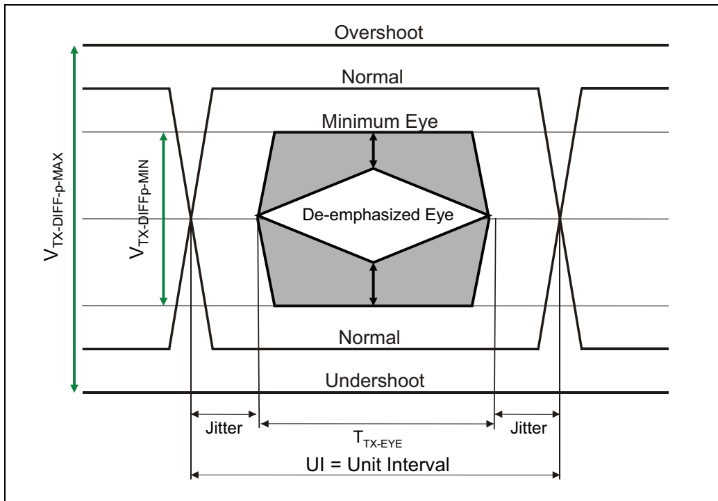
Figure 13-26: Transmitter Eye Diagram
