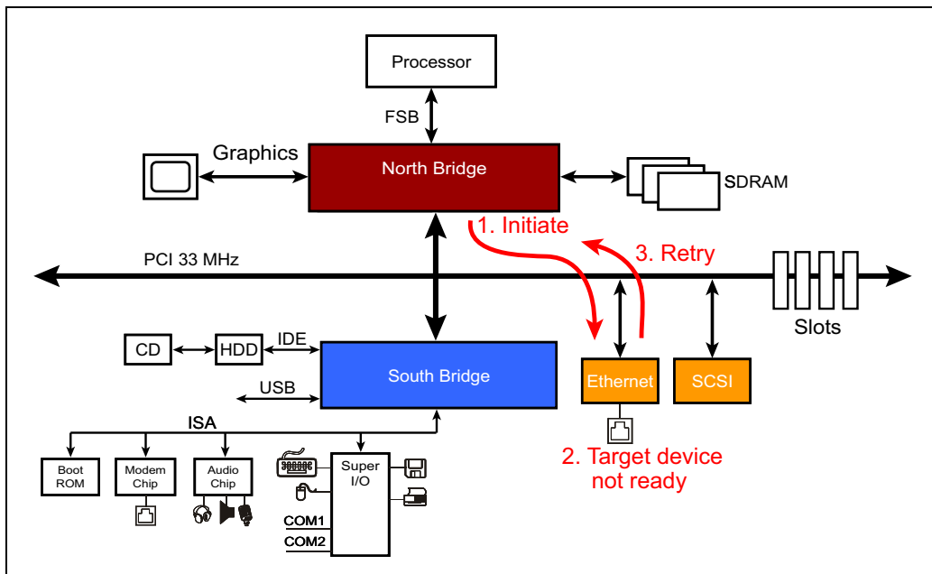
Figure 1-7: PCI Transaction Retry Mechanism
