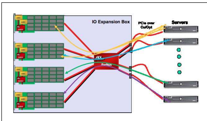
Figure 0-6: Server Failover in 1 + N Failover Scheme
