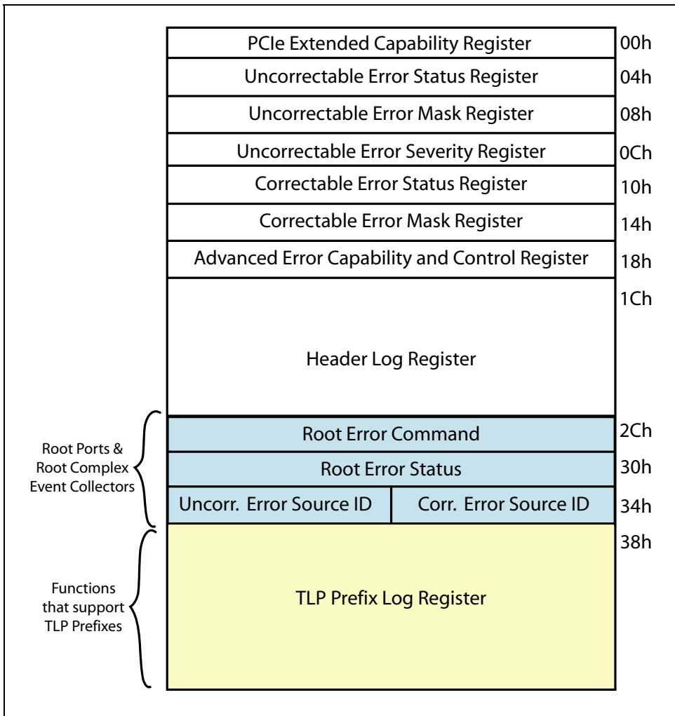
Figure 15-21: Advanced Error Capability Structure
