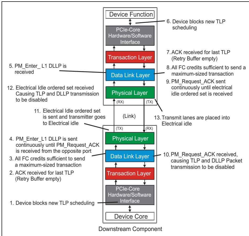
Figure 16-24: Procedure Used to Transition a Link from the L0 to L1 State
