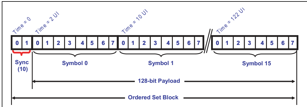
Figure 12-14: Gen3 x1 Ordered Set Construction
