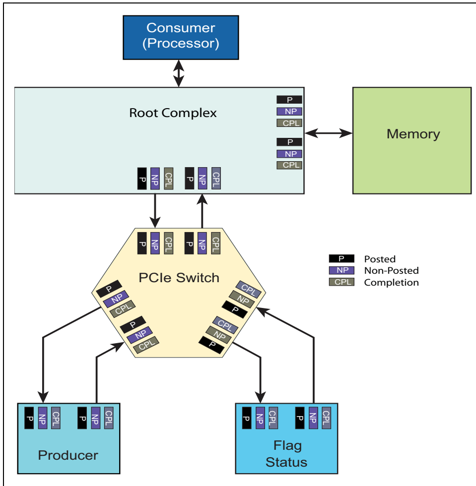
Figure 8-1: Example Producer/Consumer Topology
