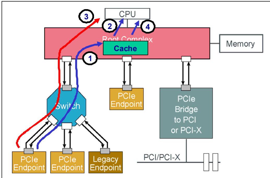
Figure 20-12: TPH Example with System Cache
