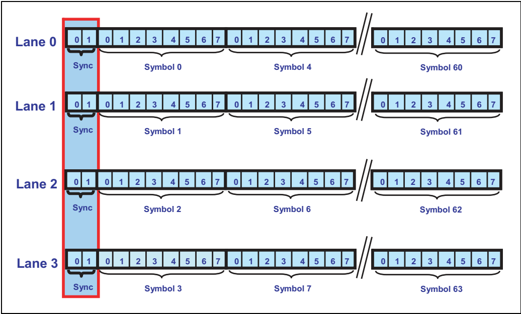
Figure 12-11: Gen3 Byte Striping x4
