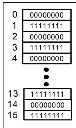
Figure 12-4: Gen3 Mode EIEOS Symbol Pattern
