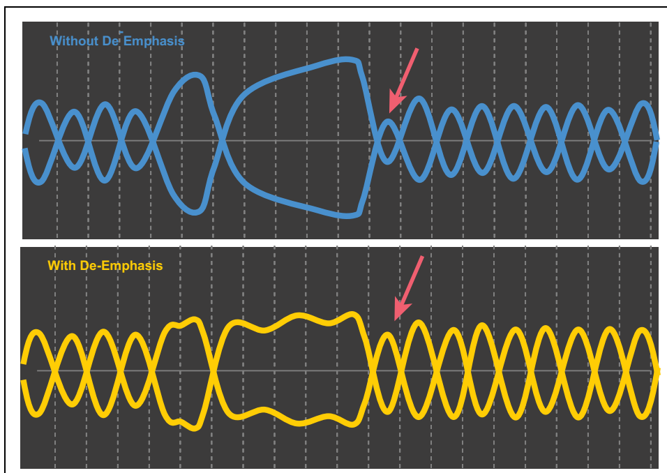
Figure 13-18: Benefit of De-emphasis at Receiver Shown With Differential Signals
