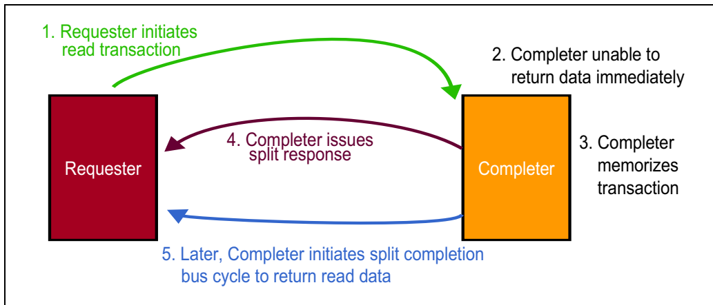
Figure 1-17: PCI-X Split Transaction Protocol
