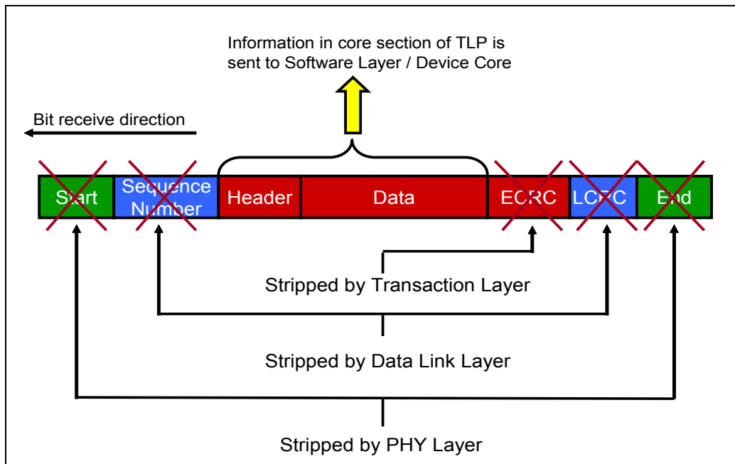
Figure 2-17: TLP Disassembly
