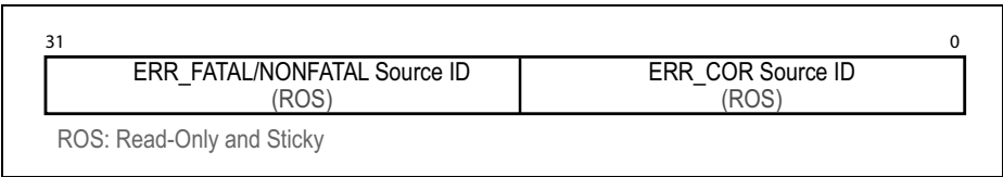
Figure 15-29: Advanced Source ID Register
