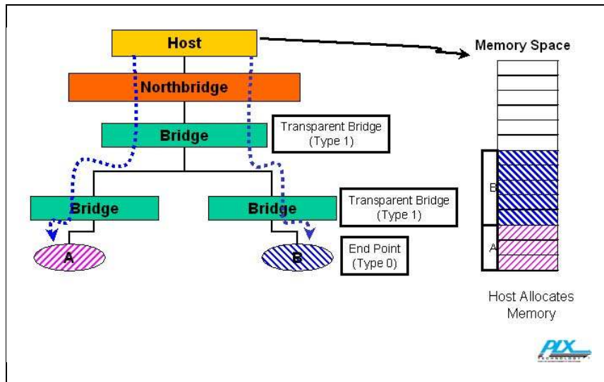
Figure 0-1: Enumeration Using Transparent Bridges
