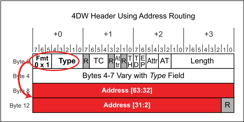
Figure 4-19: 4DW TLP Header - Address Routing Fields
