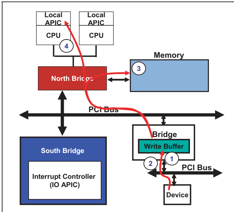
Figure 17-22: MSI Delivery
