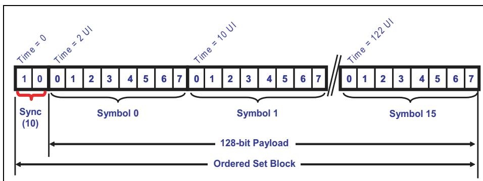
Figure 12-5: Gen3 x1 Ordered Set Block Example
