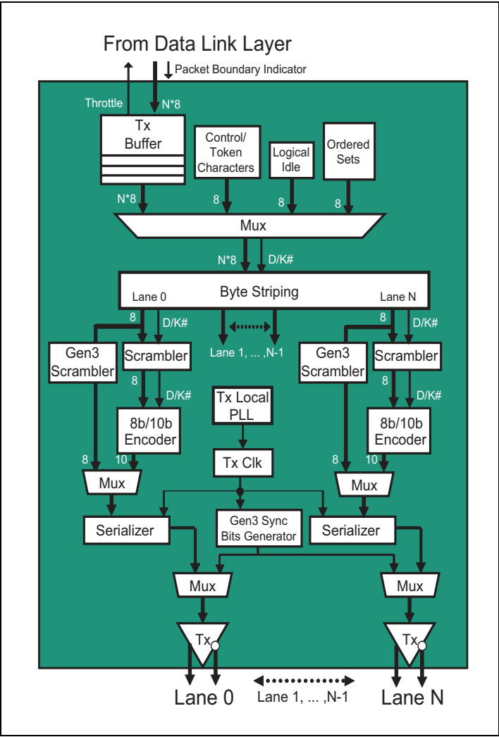
Figure 12-10: Gen3 Physical Layer Transmitter Details
