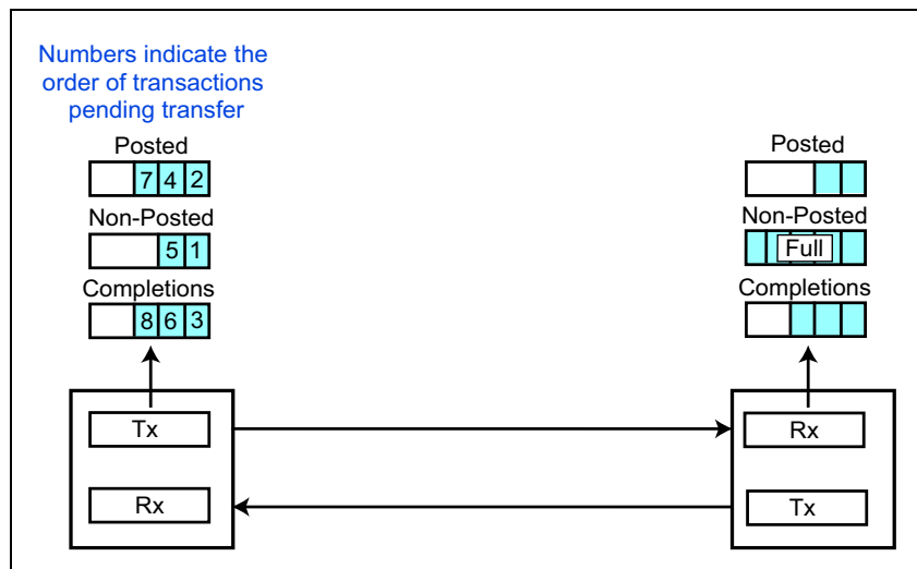
Figure 8-6: Strongly Ordered Example Results in Temporary Stall
