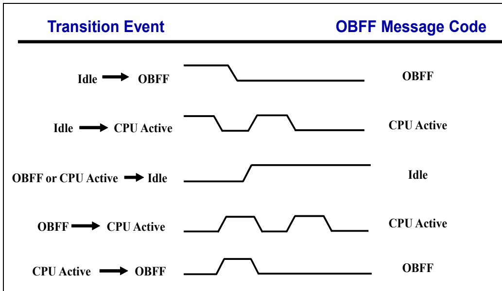
Figure 16-34: WAKE# Pin OBFF Signaling
