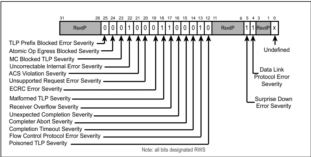
Figure 15-26: Advanced Uncorrectable Error Severity Register
