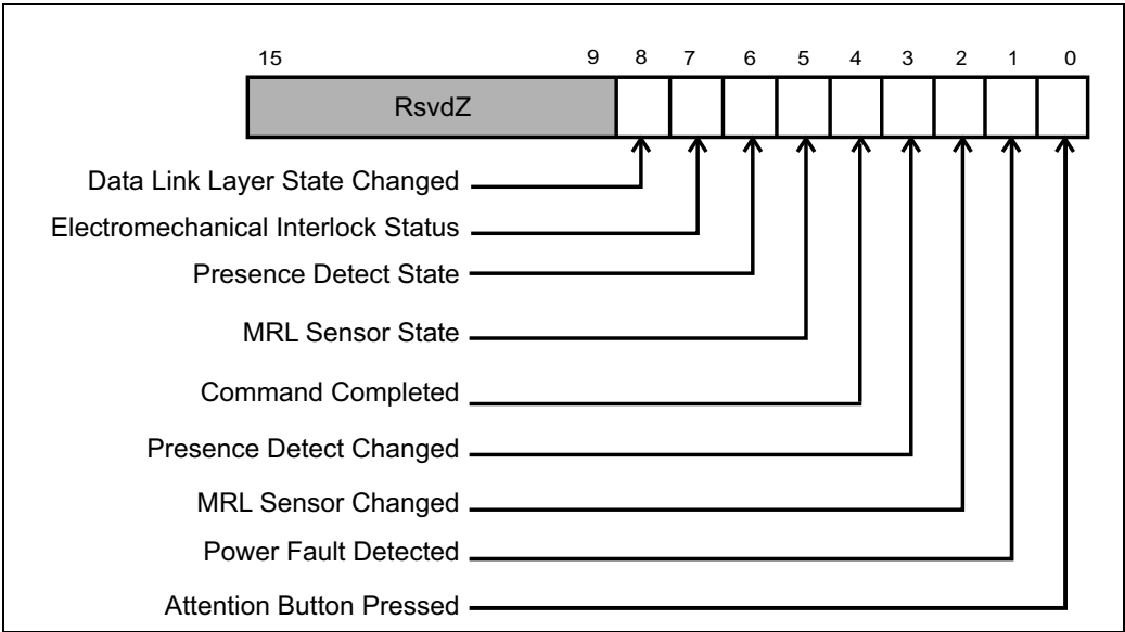
Figure 19-7: Slot Status Register
