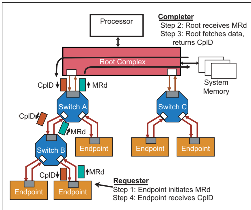
Figure 2-18: Non-Posted Read Example
