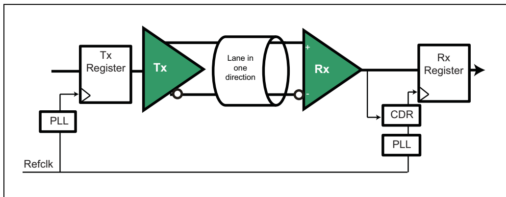
Figure 13-7: Shared Refclk Architecture
