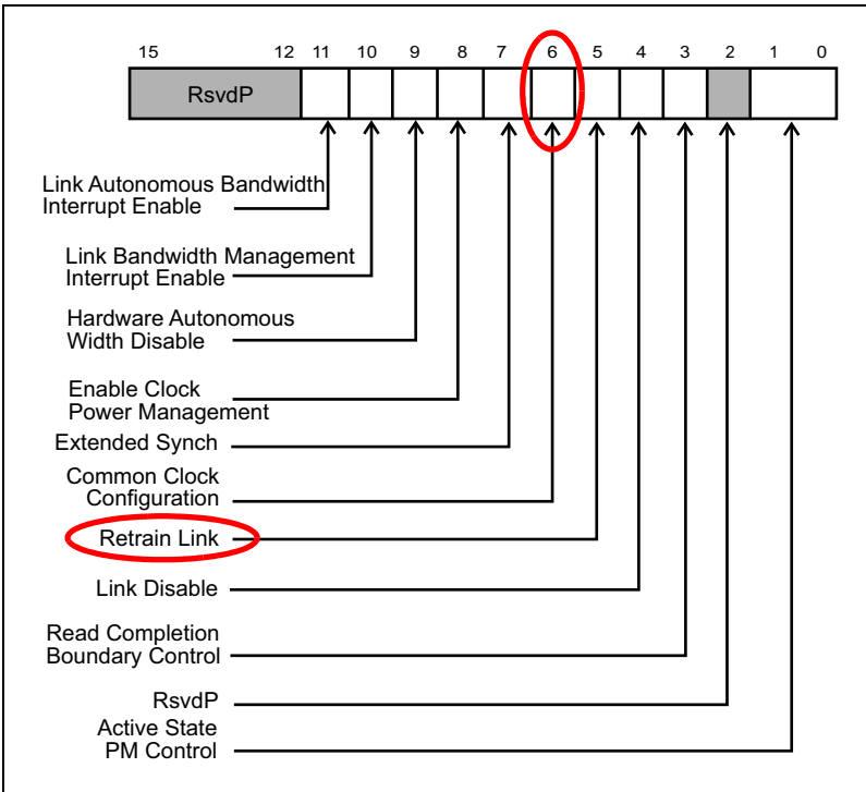
Figure 15-19: Link Control Register - Force Link Retraining
