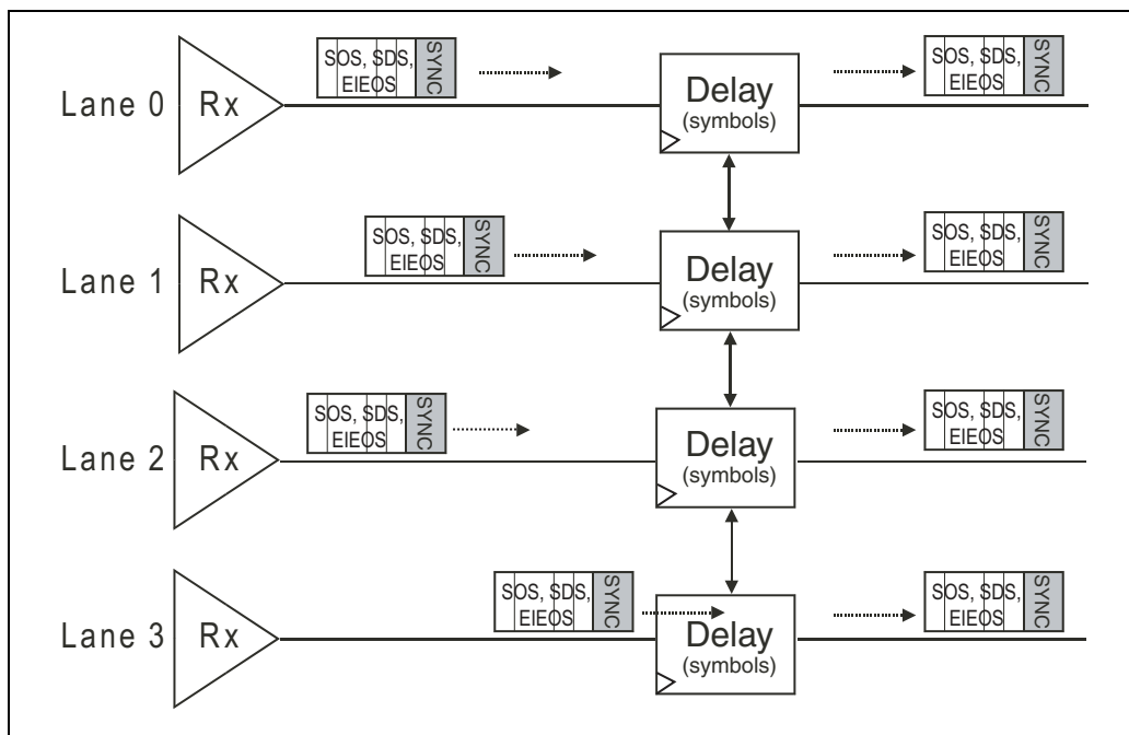
Figure 12-22: Receiver Link De-Skew Logic
