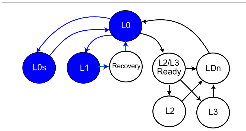
Figure 16-13: ASPM Link State Transitions
