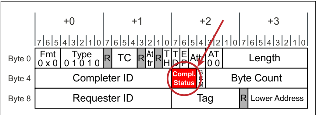
Figure 15-7: Completion Status Field within the Completion Header
