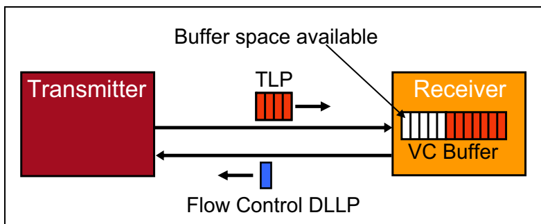
Figure 2-23: Flow Control Basics
