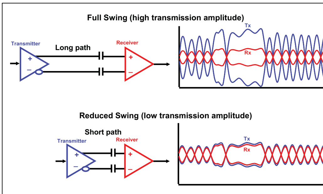
Figure 13-20: Reduced-Swing Option for 5.0 GT/s with No De-emphasis
