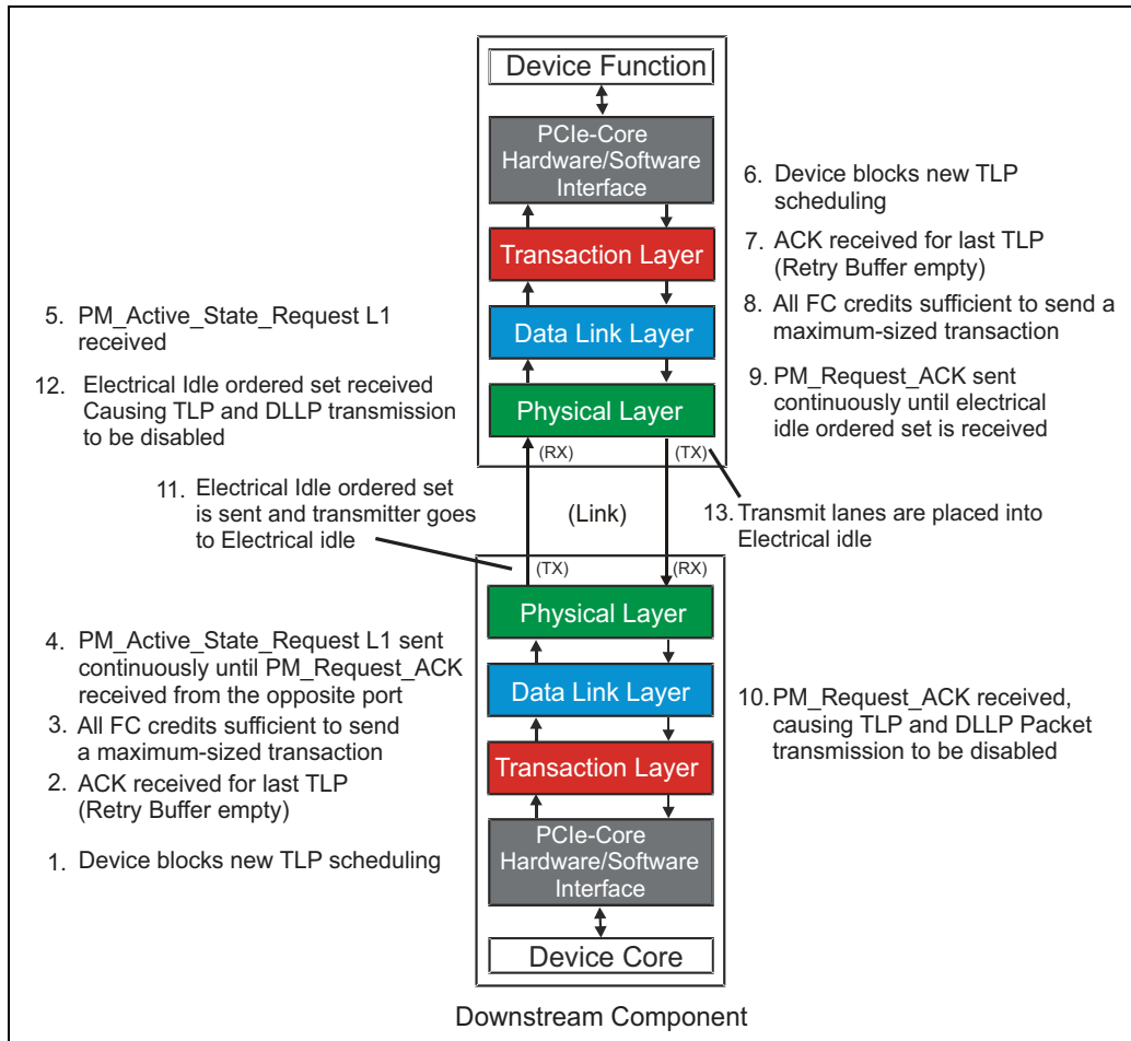
Figure 16-17: Negotiation Sequence Required to Enter L1 Active State PM
