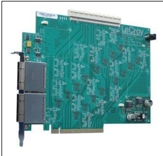
Figure A-2: LeCroy PCI Express Slot Interposer x16
