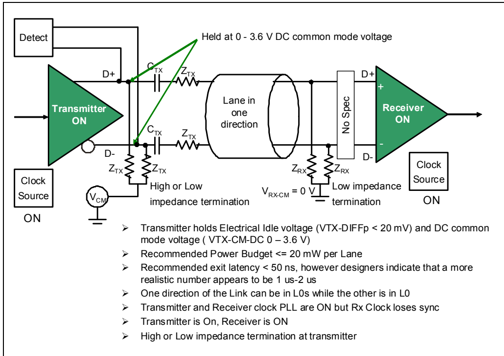
Figure 13-36: L0s Low Power Link State
