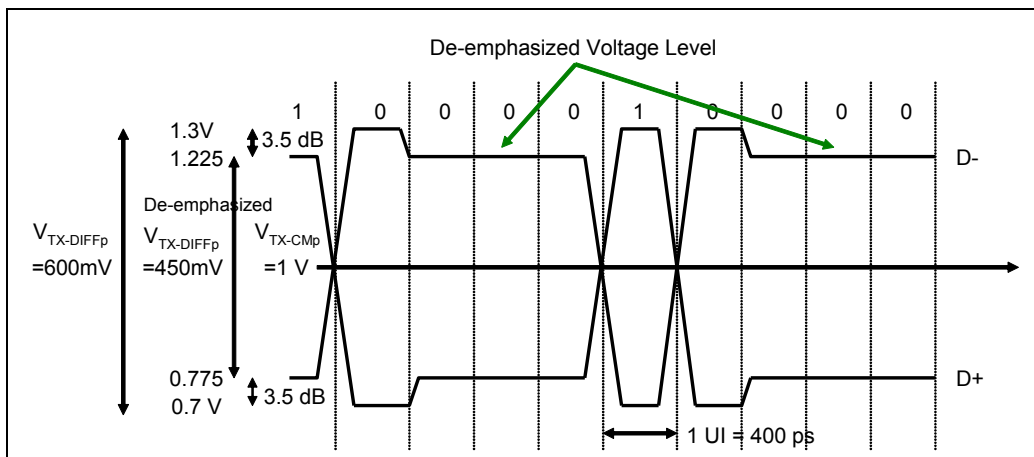
Figure 13-16: Transmission with De-emphasis
