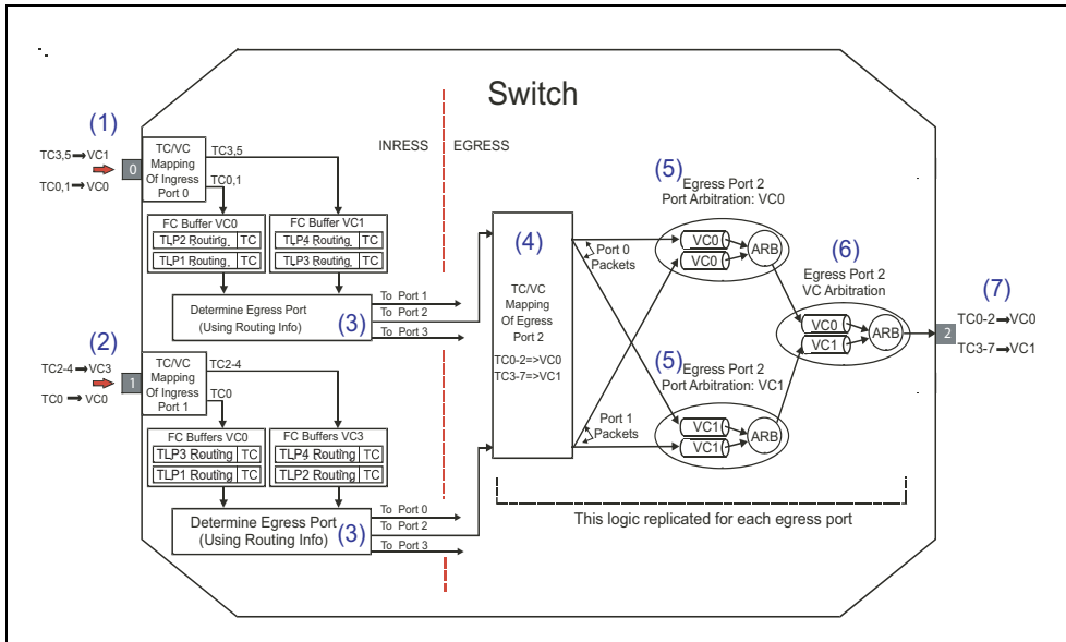
Figure 7-20: Arbitration Examples in a Switch
