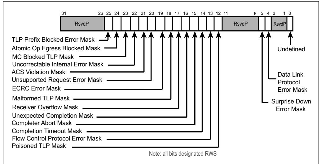
Figure 15-27: Advanced Uncorrectable Error Mask Register
