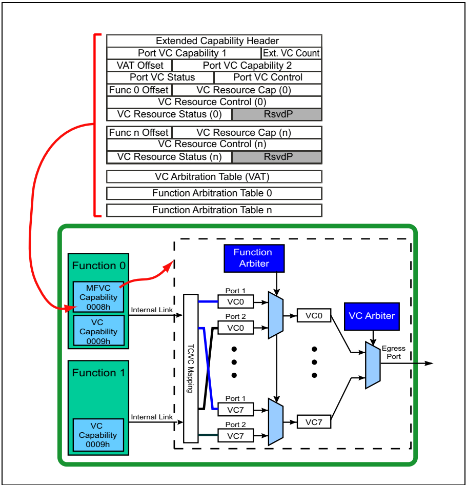
Figure 7-22: QoS Support in Multi-Function Arbitration
