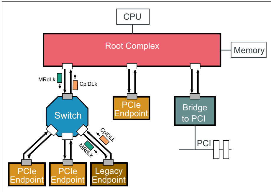
Figure 2-19: Non-Posted Locked Read Transaction Protocol
