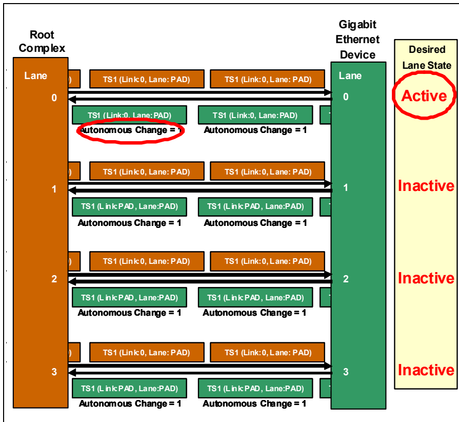
Figure 14-64: Marking Active Lanes
