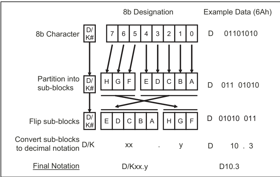
Figure 11-16: 8b/10b Nomenclature
