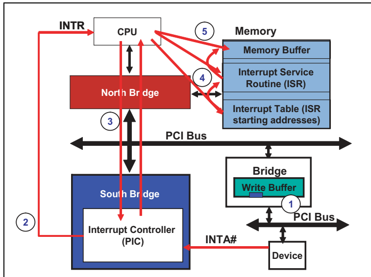
Figure 17-21: Memory Synchronization Problem
