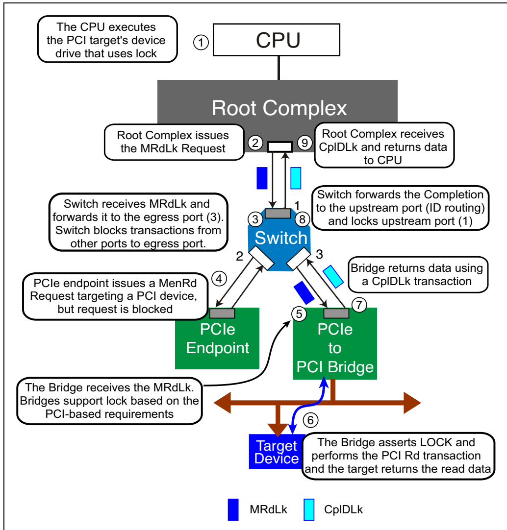
Figure D-1: Lock Sequence Begins with Memory Read Lock Request
