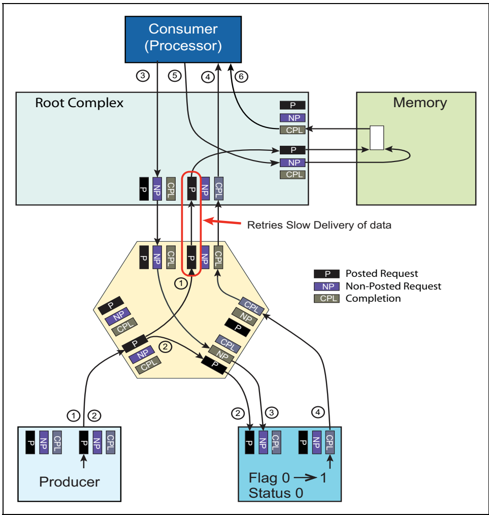
Figure 8-4: Producer/Consumer Sequence with Error
