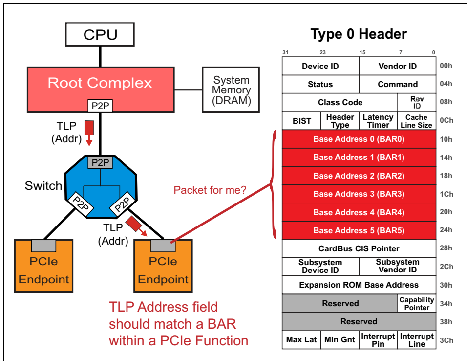
Figure 4-20: Endpoint Checks Incoming TLP Address
