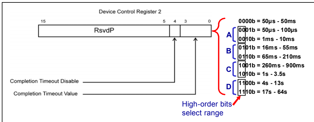
Figure 15-8: Device Control Register 2
