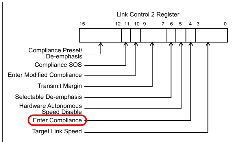
Figure 14-12: Link Control 2 Register’s “Enter Compliance” Bit
