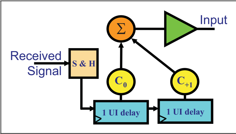
Figure 13-29: Rx Discrete-Time Linear Equalizer (DLE)
