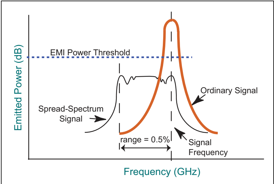
Figure 13-4: SSC Motivation
