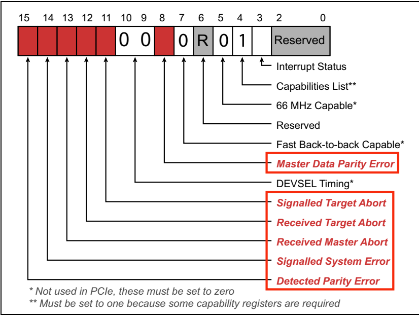
Figure 15-14: Status Register in Configuration Header
