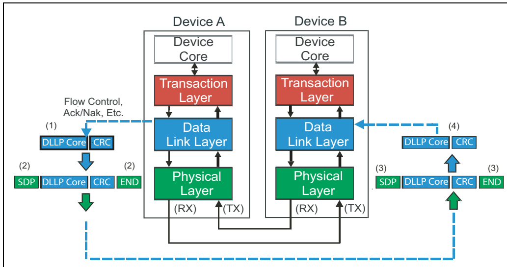
Figure 2-24: DLLP Origin and Destination
