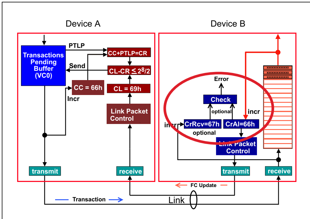
Figure 6-14: Buffer Overflow Error Check
