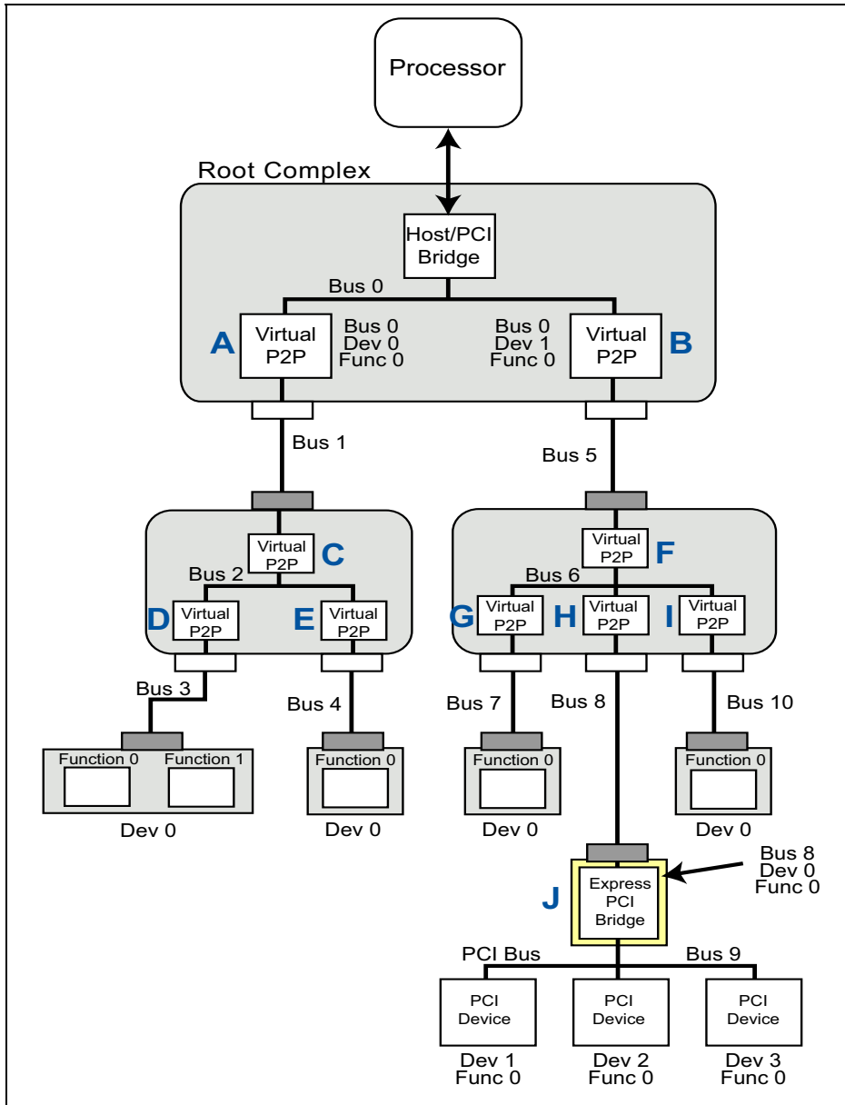
Figure 3-13: Single-Root System
