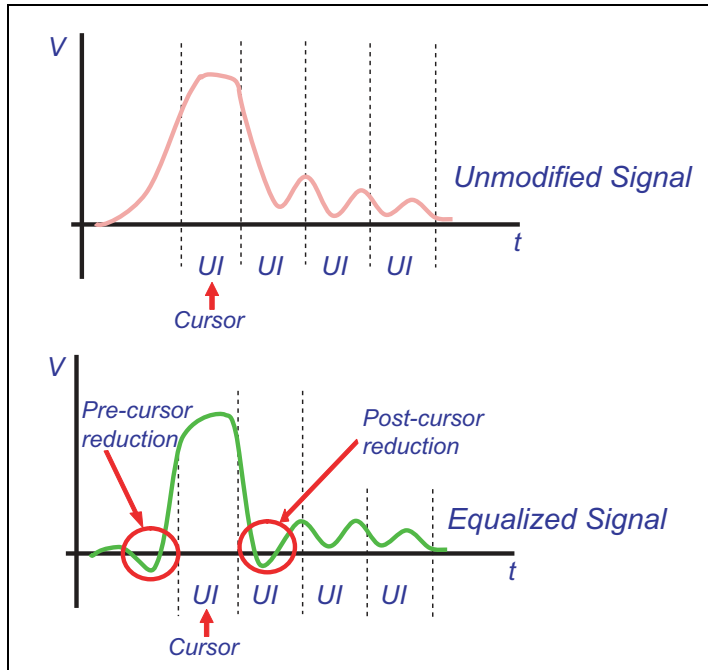
Figure 14-34: Equalization Process: Adjustments During Phase 2
