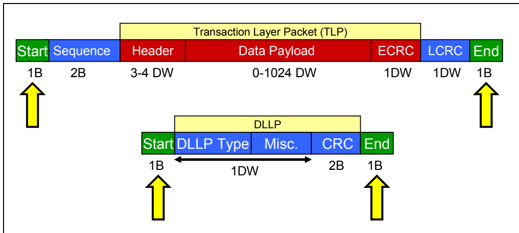
Figure 2-28: TLP and DLLP Structure at the Physical Layer
