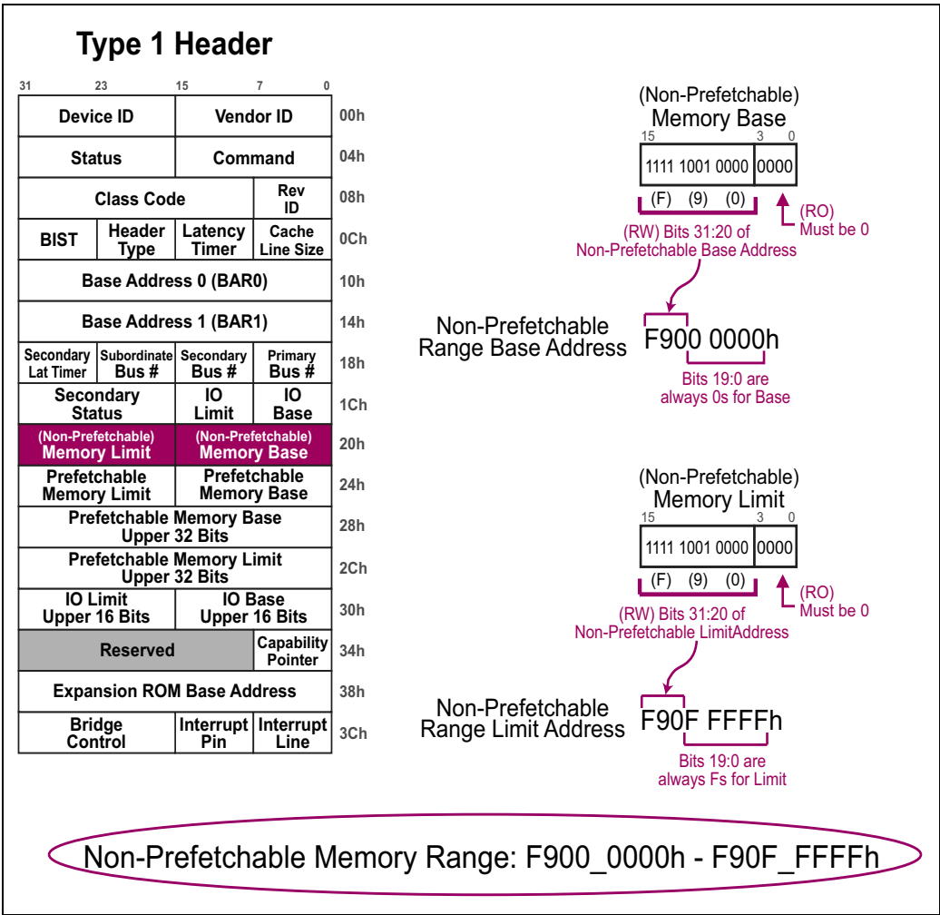
Figure 4-9: Example Non-Prefetchable Memory Base/Limit Register Values
