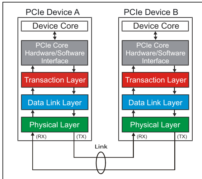
Figure 2-12: PCI Express Device Layers
