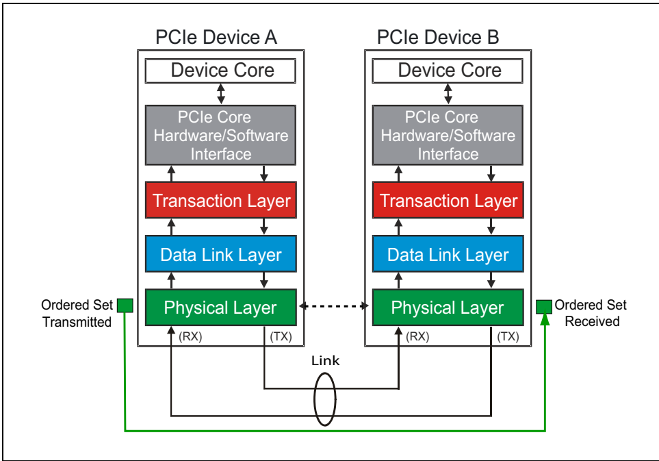
Figure 2-30: Ordered Sets Origin and Destination
