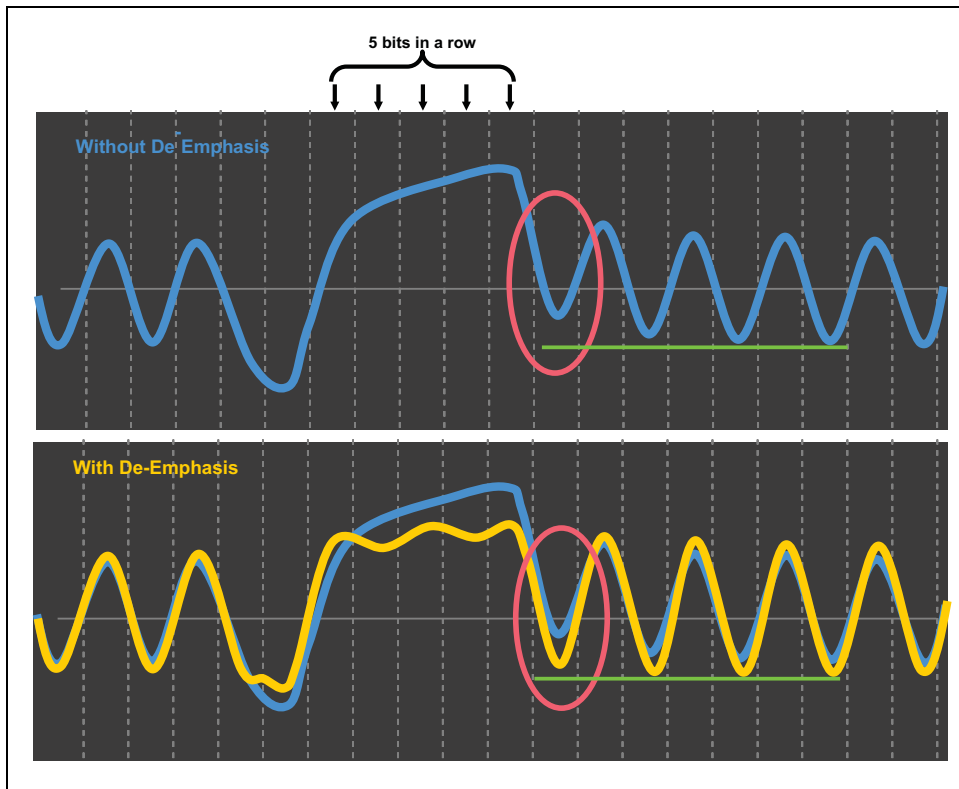
Figure 13-17: Benefit of De-emphasis at the Receiver
