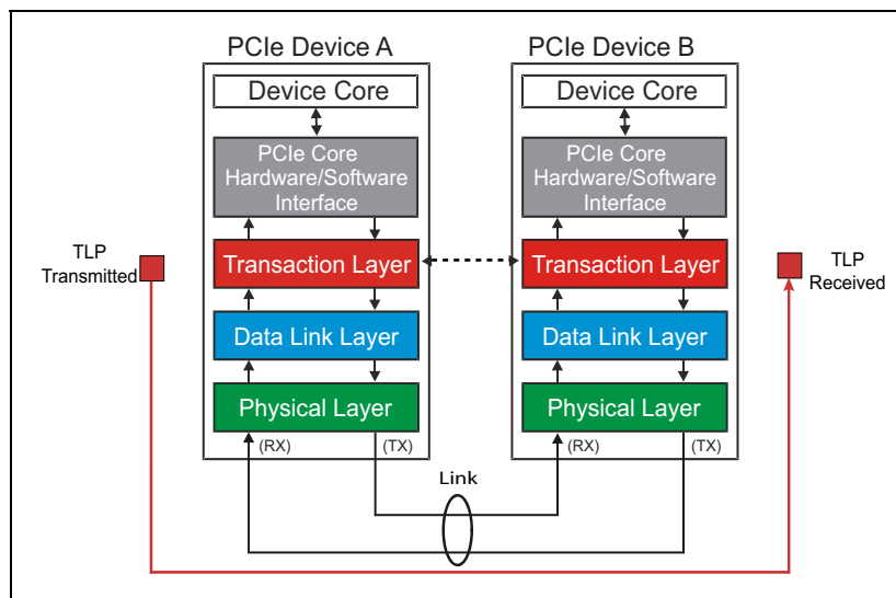
Figure 2-15: TLP Origin and Destination
