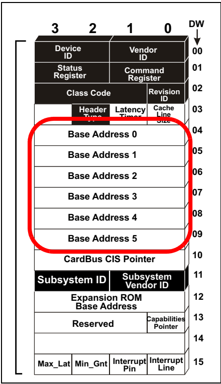
Figure 20-23: BARs in a Type0 Configuration Header
