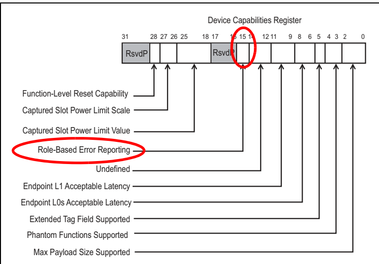
Figure 15-10: Device Capabilities Register
