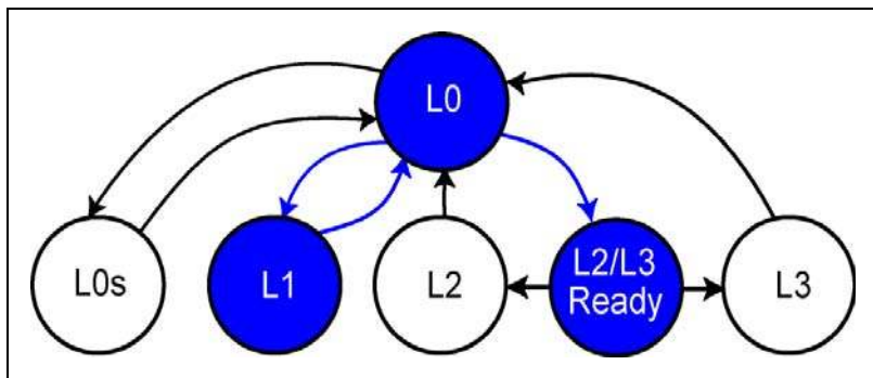
Figure 16-25: Link States Transitions Associated with Preparing Devices for Removal of the Reference Clock and Power
