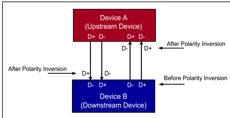
Figure 14-3: Polarity Inversion Example (Support Required)
