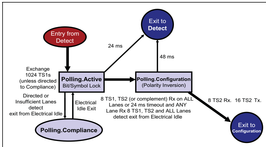
Figure 14-9: Polling State Machine
