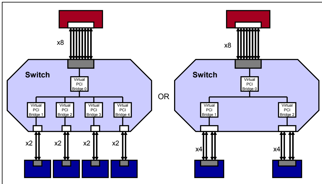
Figure 14-14: Combining Lanes to Form Wider Links (Link Merging)
