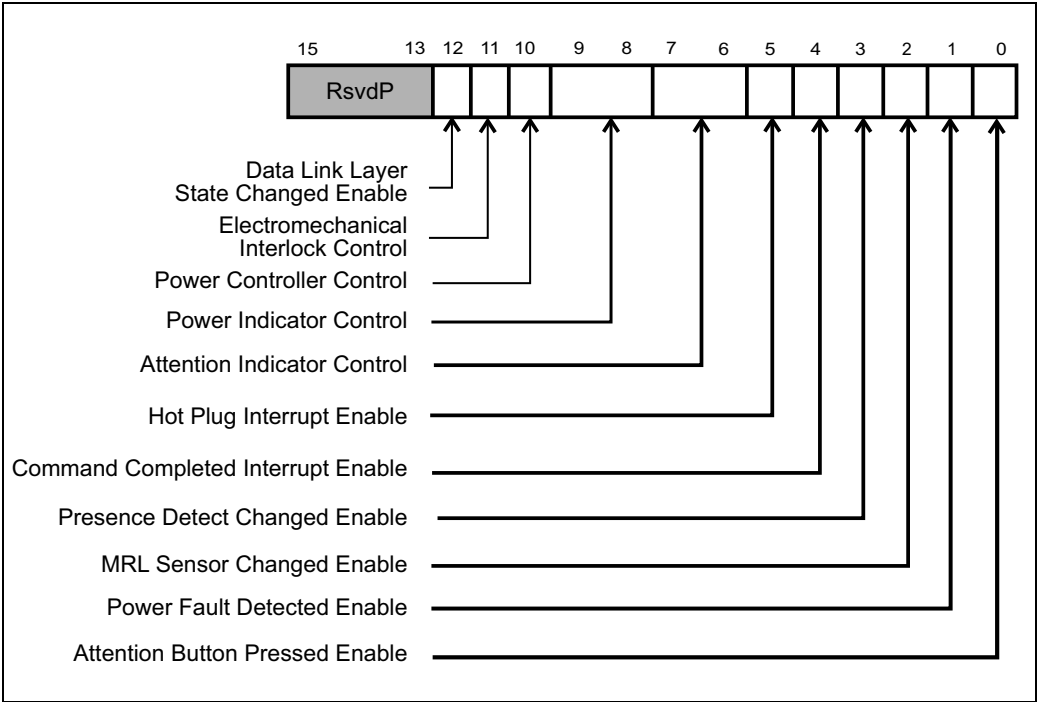
Figure 19-6: Slot Control Register
