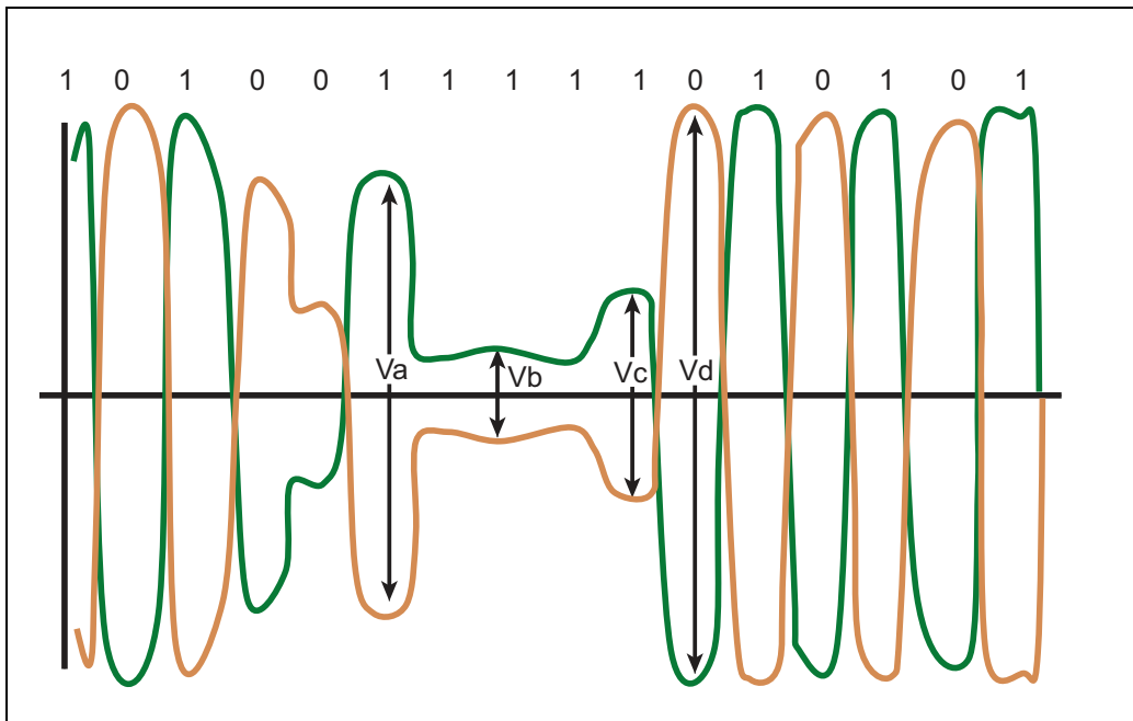
Figure 13-23: 8.0 GT/s Tx Voltage Levels
