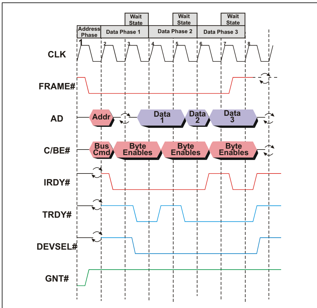
Figure 1-3: Simple PCI Bus Transfer
