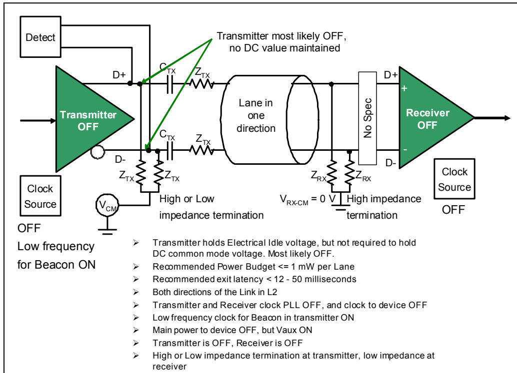
Figure 13-38: L2 Low Power Link State
