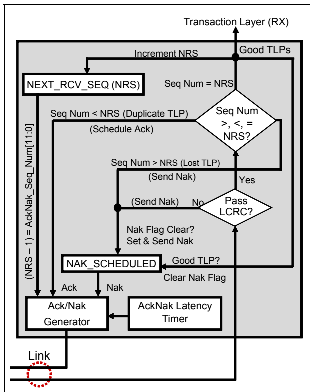
Figure 10-5: Receiver Elements Associated with the Ack/Nak Protocol
