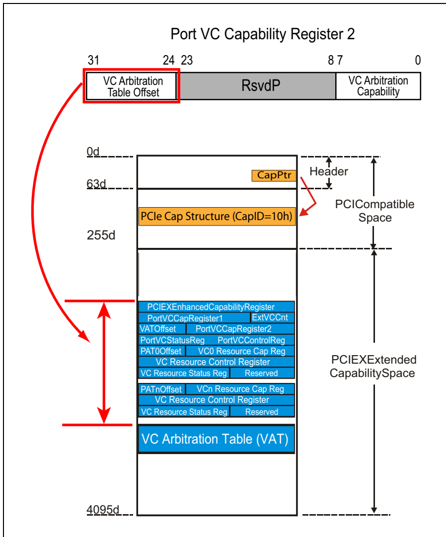
Figure 7-12: VC Arbitration Table Offset and Load VC Arbitration Table Fields
