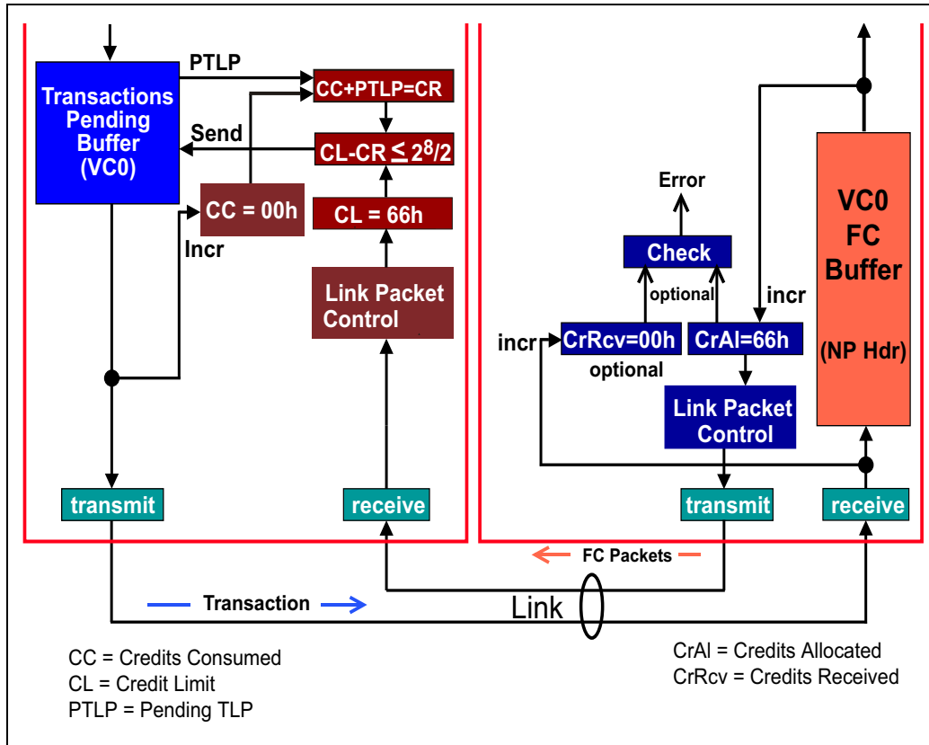
Figure 6-10: Flow Control Elements Following Initialization
