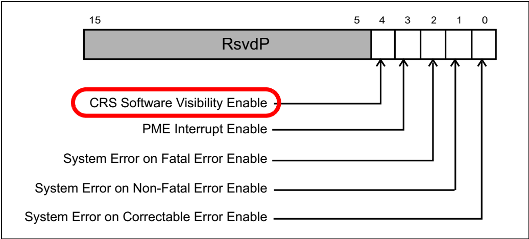
Figure 3-11: Root Control Register in PCIe Capability Block
