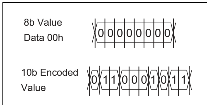
Figure 11-15: Example of 8-bit Character 00h Encoding
