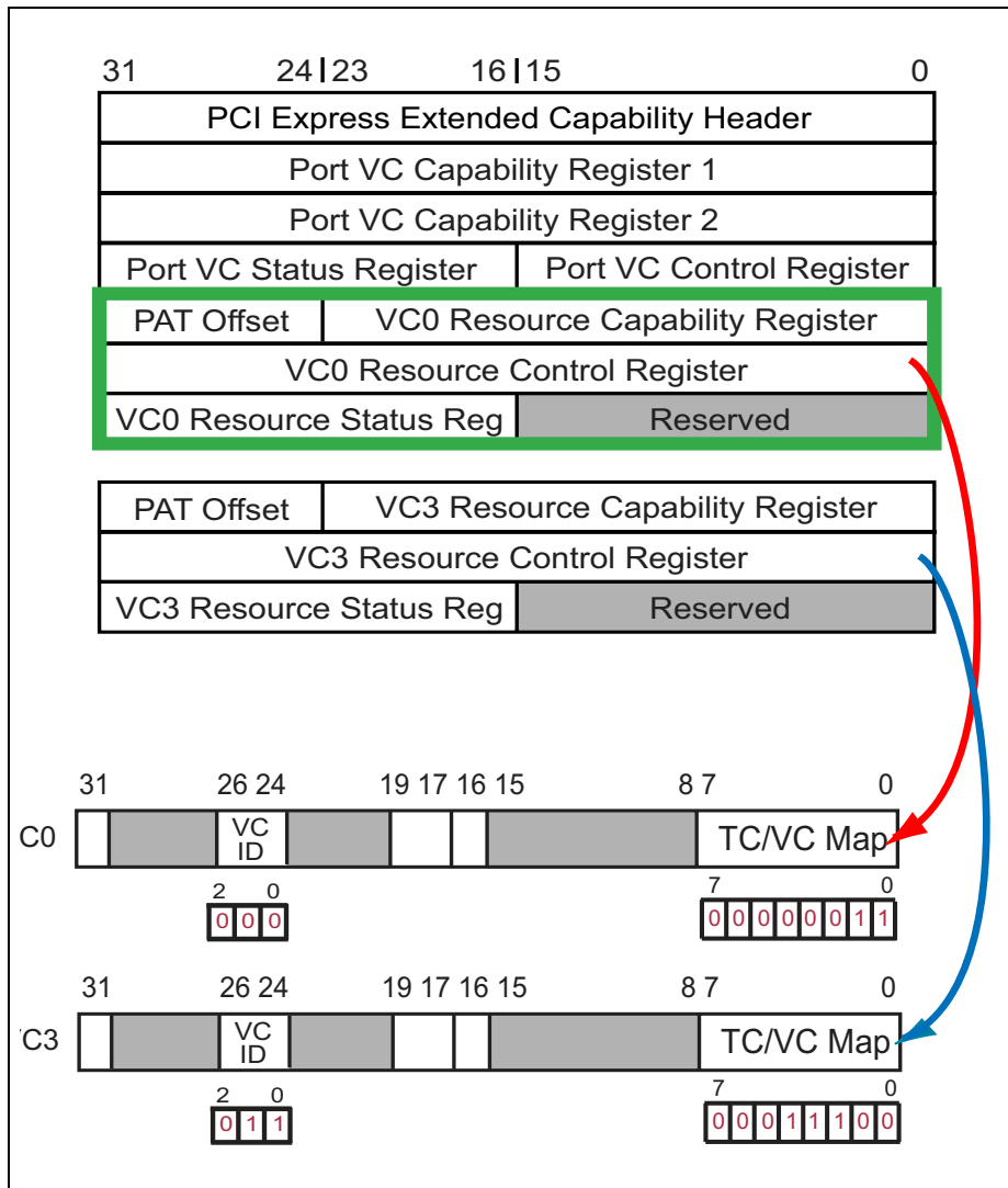
Figure 7-3: TC to VC Mapping Example
