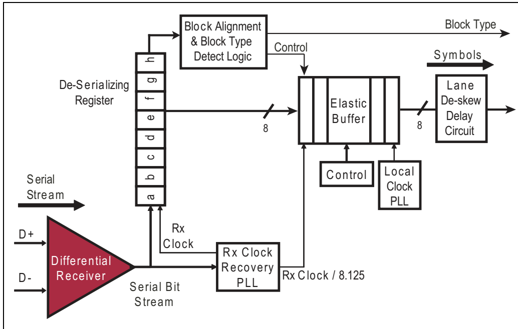
Figure 12-19: Gen3 CDR Logic
