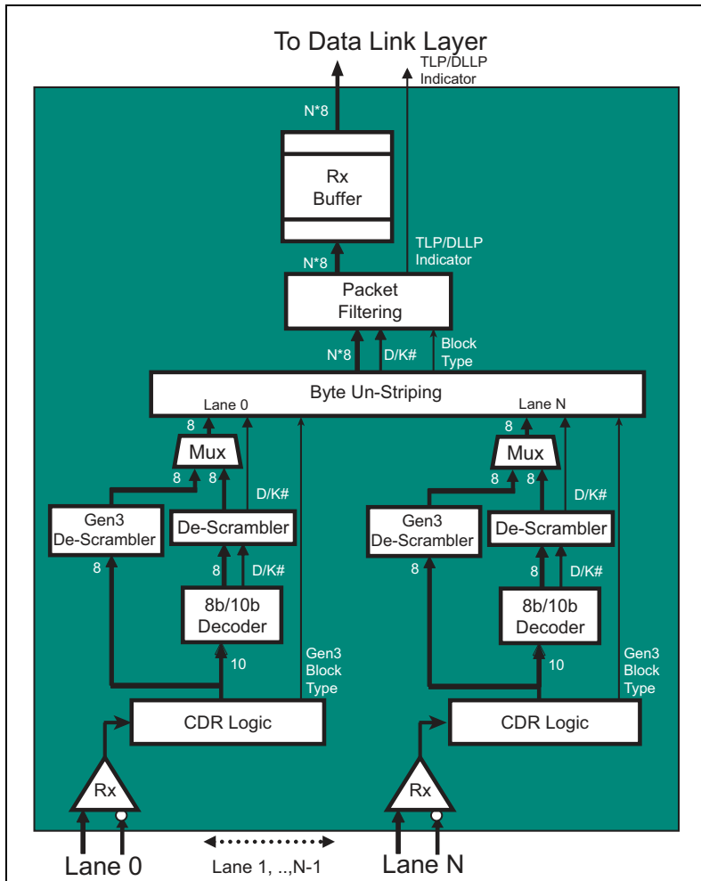
Figure 12-23: Physical Layer Receive Logic Details
