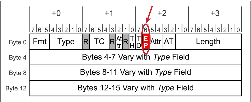
Figure 15-6: The Error/Poisoned Bit in a Completion Header
