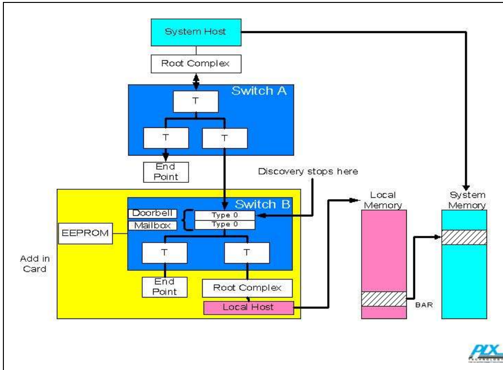
Figure 0-4: Intelligent Adapters in PCI and PCI Express Systems
