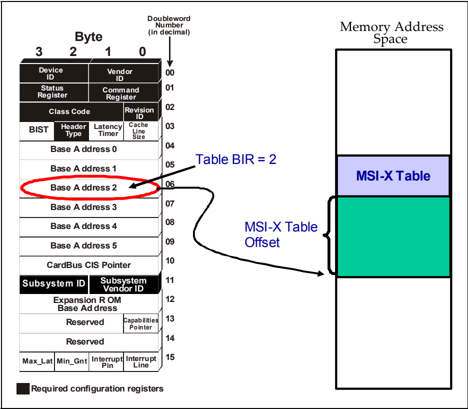
Figure 17-18: Location of MSI-X Table
