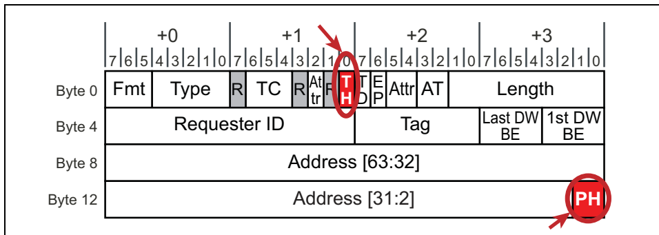
Figure 20-15: TPH Header Bits
