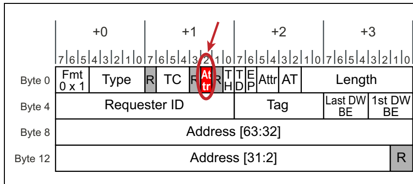
Figure 8-8: IDO Attribute in 64-bit Header
