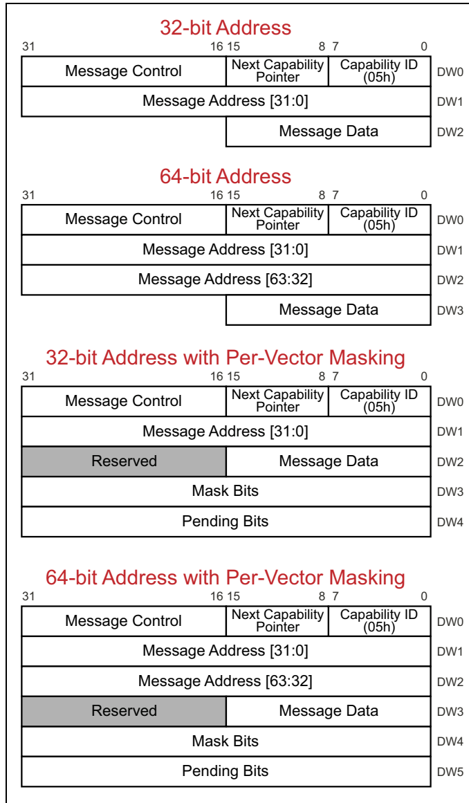
Figure 17-13: MSI Capability Structure Variations
