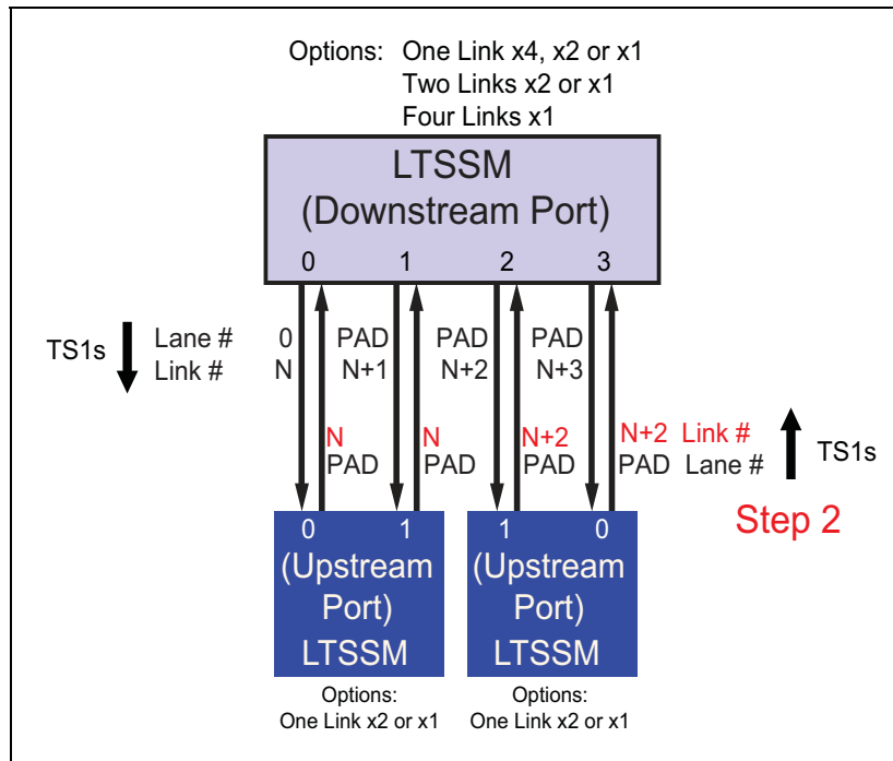
Figure 14-19: Example 2 - Step 2
