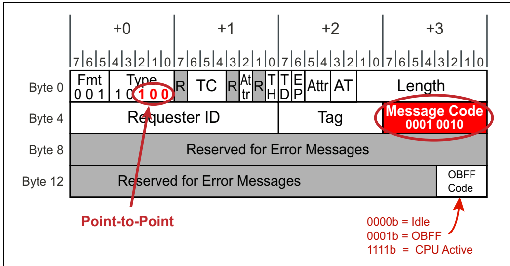
Figure 16-35: OBFF Message Contents
