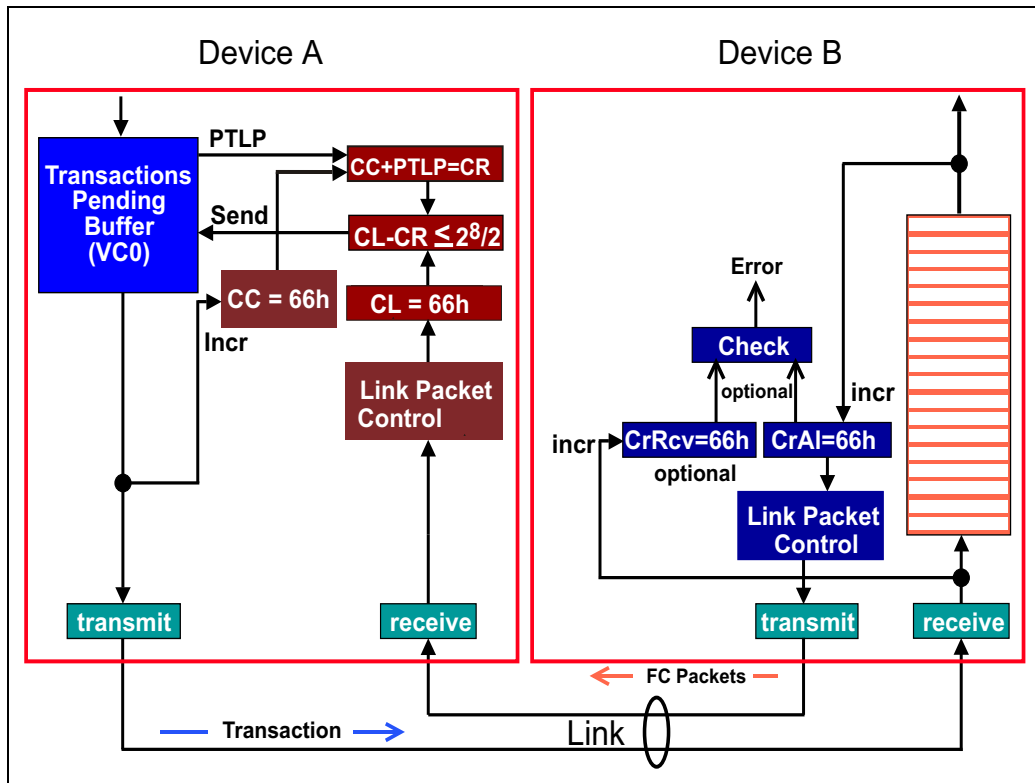
Figure 6-12: Flow Control Elements with Flow Control Buffer Filled
