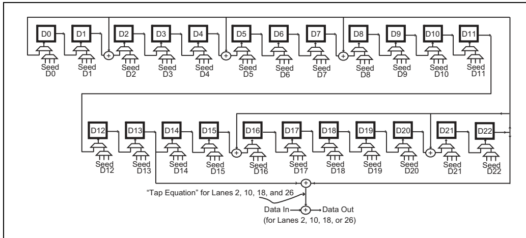
Figure 12-17: Gen3 Single-LFSR Scrambler
