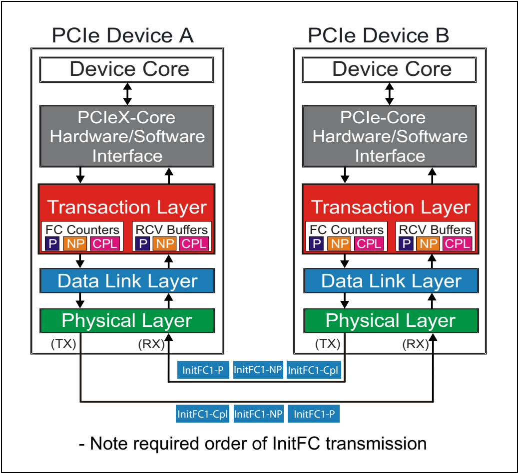
Figure 6-6: Devices Send InitFC1 in the DL_Init State
