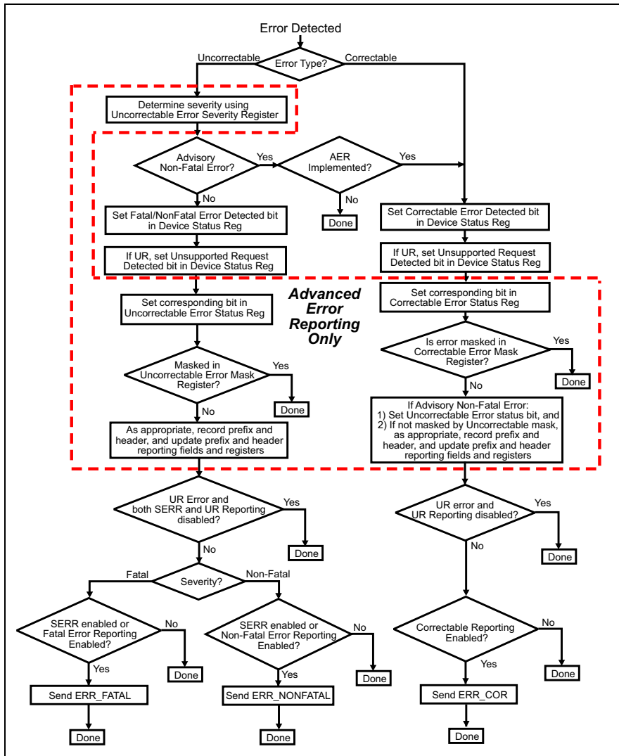
Figure 15-31: Flow Chart of Error Handling Within a Function
