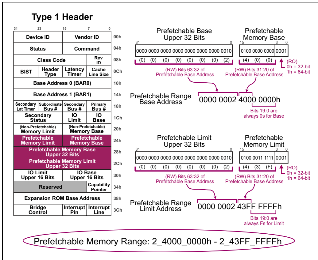
Figure 4-8: Example Prefetchable Memory Base/Limit Register Values
