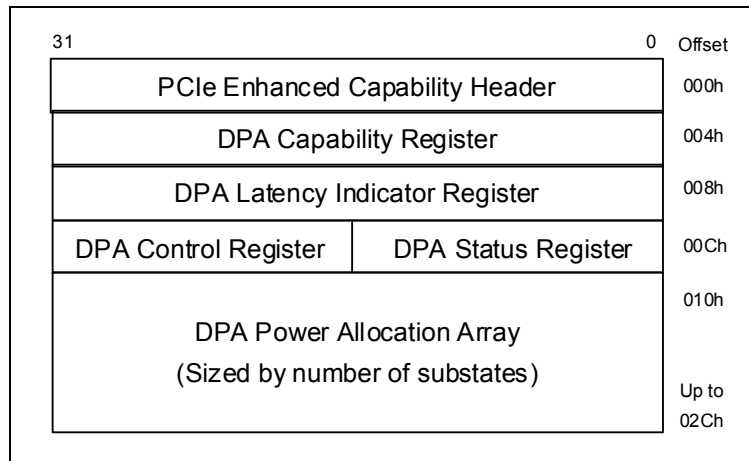
Figure 16-3: Dynamic Power Allocation Registers
