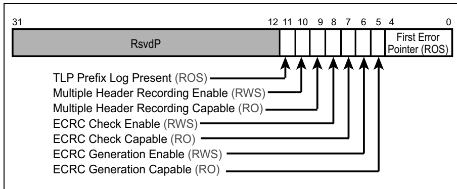
Figure 15-22: The Advanced Error Capability and Control Register
