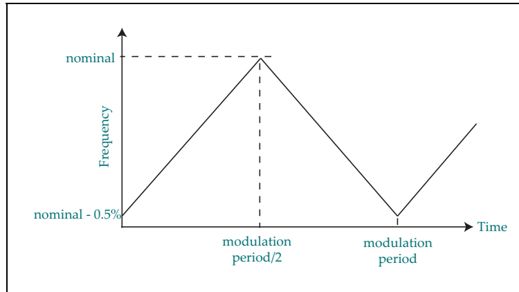
Figure 13-6: SSC Modulation Example
