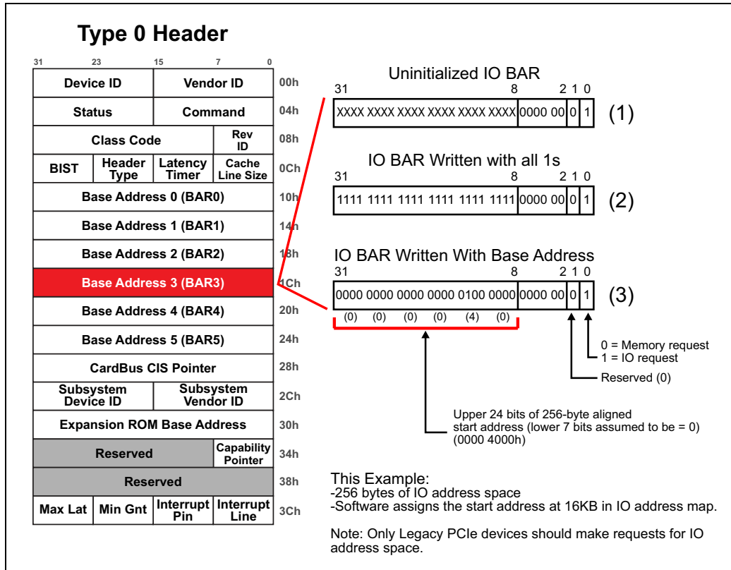
Figure 4-6: IO BAR Set Up
