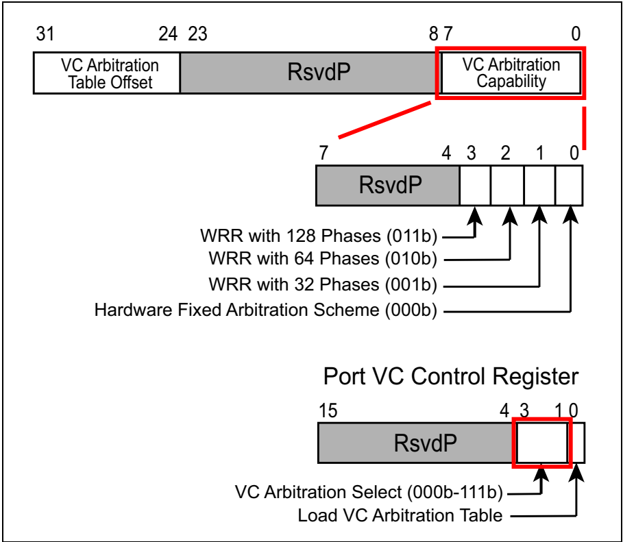
Figure 7-9: VC Arbitration Capabilities
