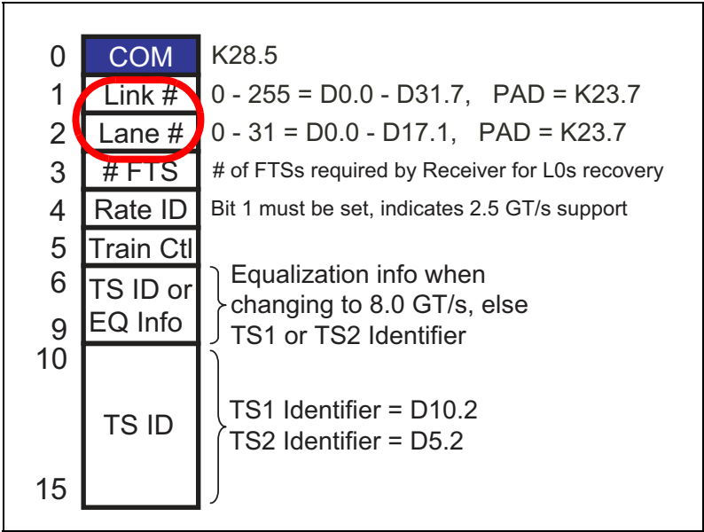
Figure 14-13: Link and Lane Number Encoding in TS1/TS2
