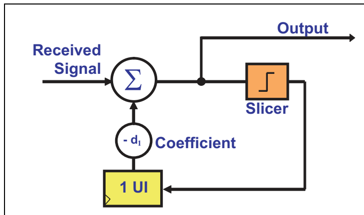
Figure 13-32: Rx 1-Tap DFE
