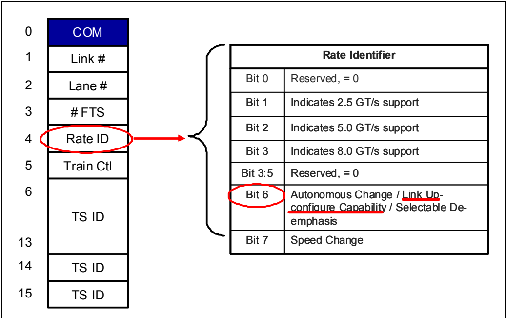
Figure 14-58: TS2 Contents
