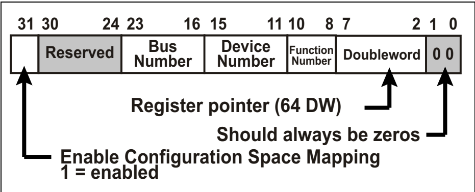
Figure 3-4: Configuration Address Port at 0CF8h
