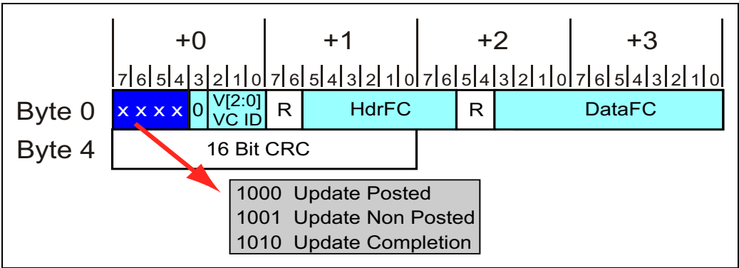
Figure 6-9: Types and Format of Flow Control DLLPs
