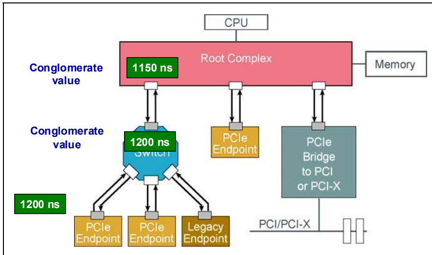
Figure 16-41: LTR Example
