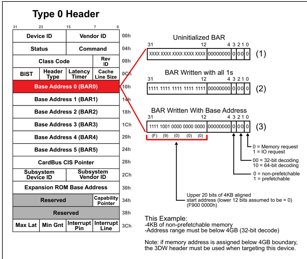
Figure 4-4: 32-Bit Non-Prefetchable Memory BAR Set Up
