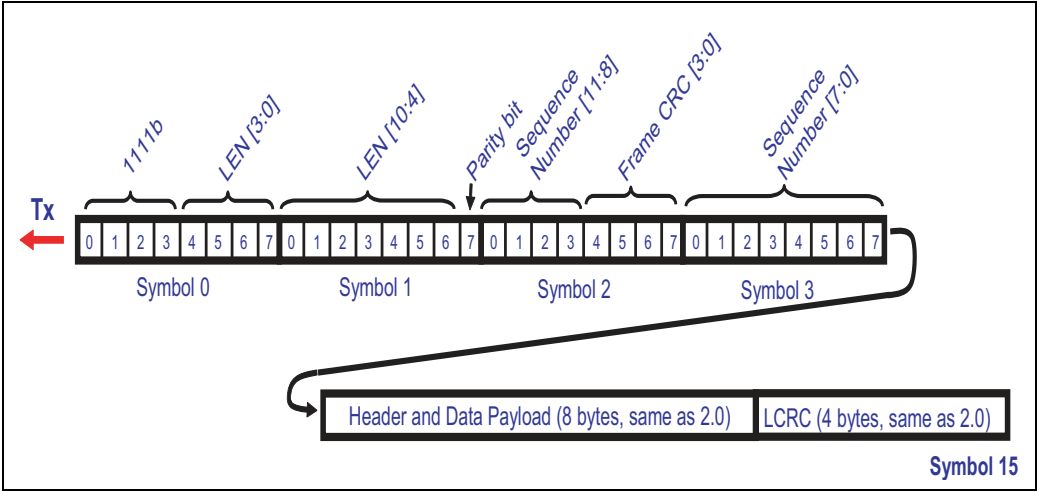
Figure 12-7: Gen3 x1 Frame Construction Example
