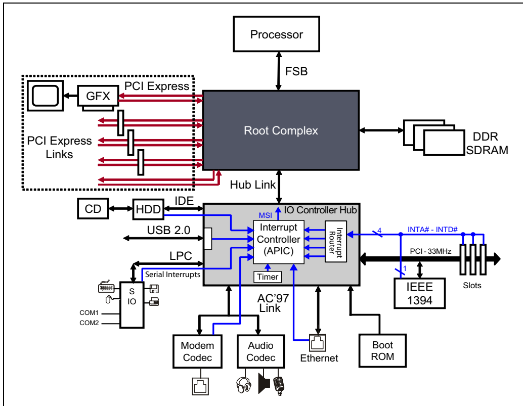
Figure 17-23: PCI Express System with PCI-Based IO Controller Hub
