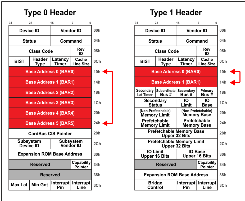
Figure 4-2: BARs in Configuration Space
