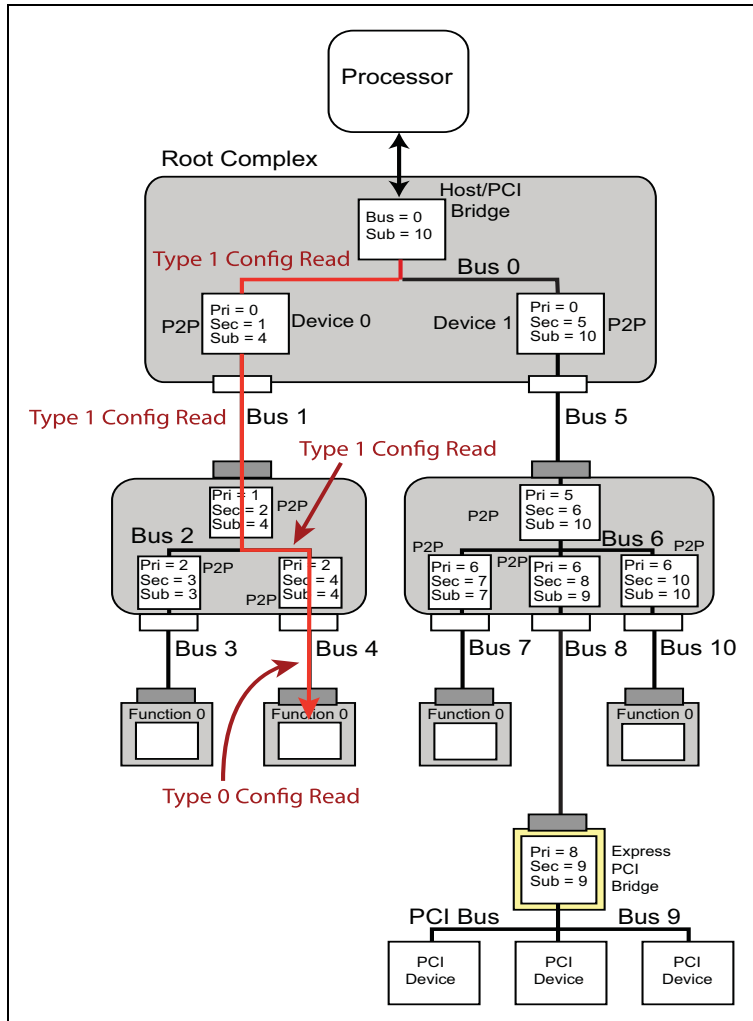
Figure 3-9: Example Configuration Read Access
