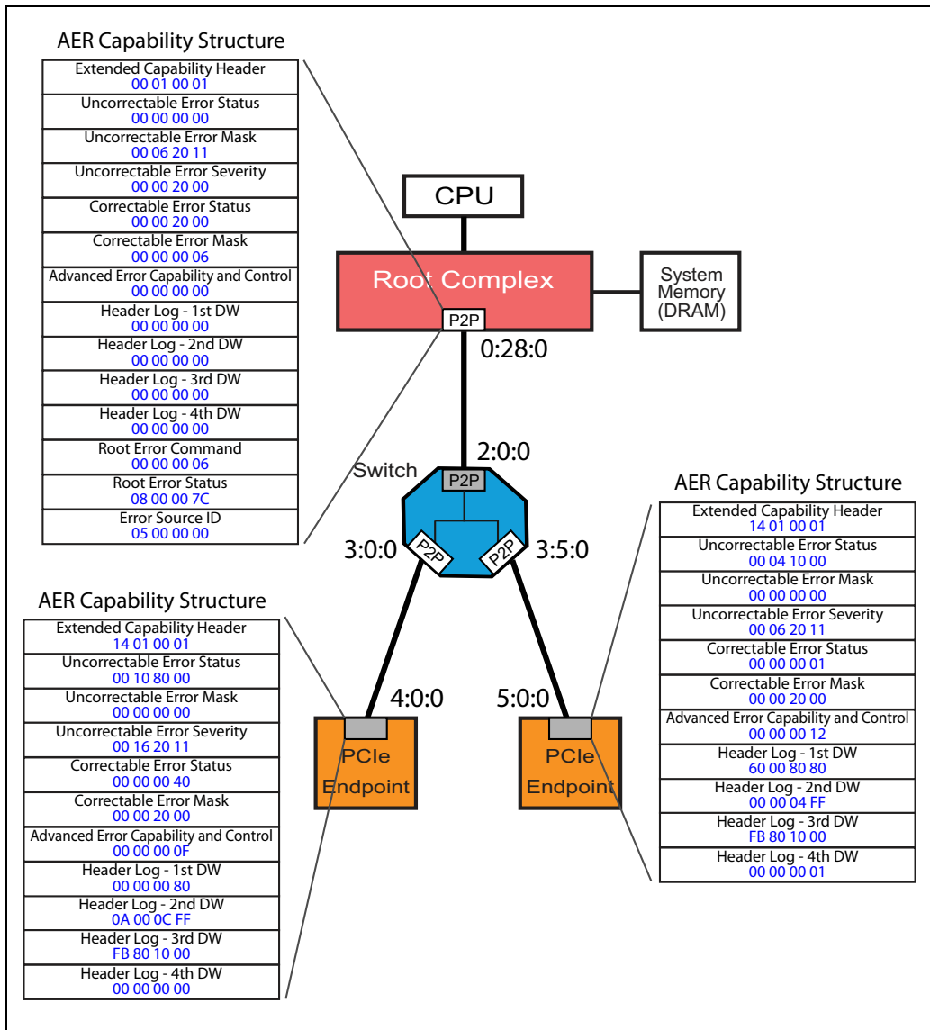
Figure 15-32: Error Investigation Example System
