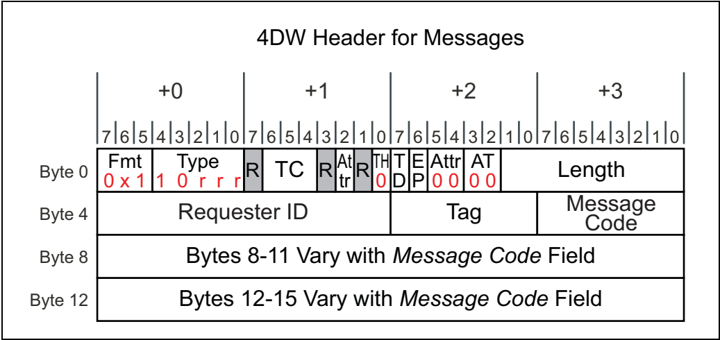
Figure 4-22: 4DW Message TLP Header - Implicit Routing Fields
