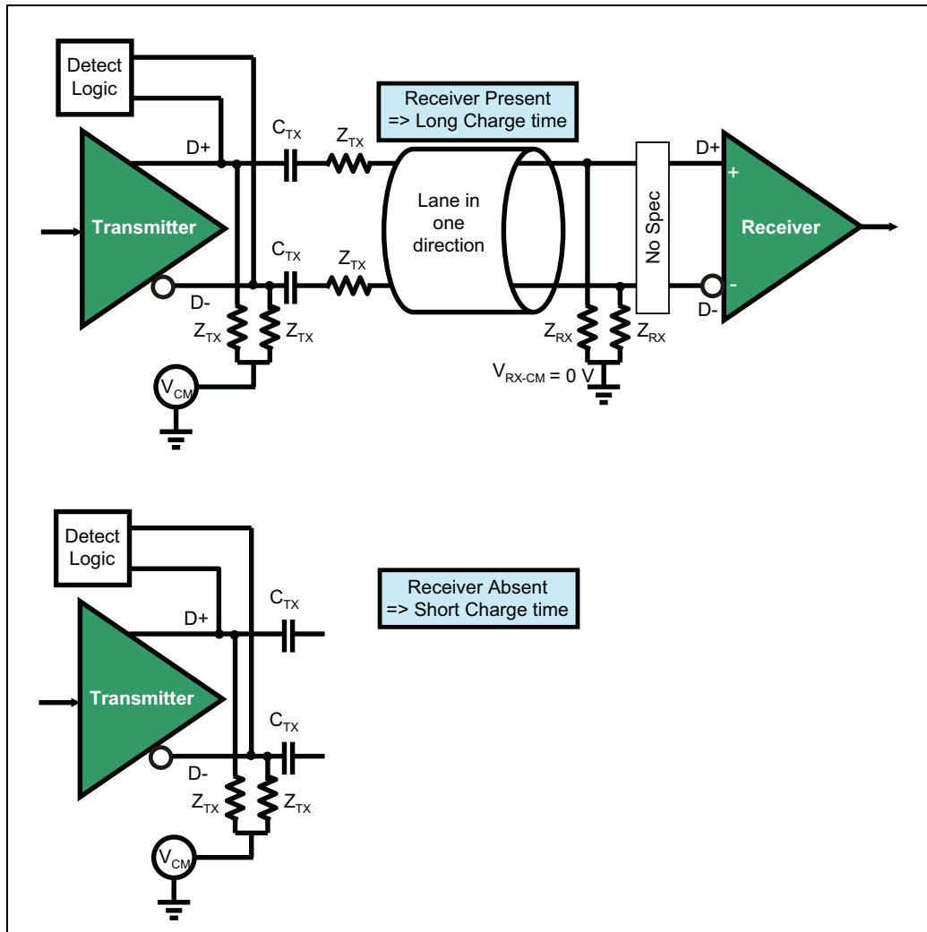
Figure 13-11: Receiver Detection Mechanism
