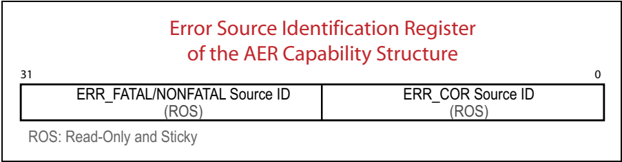
Figure 15-12: Advanced Source ID Register
