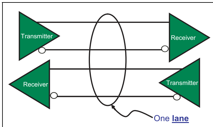
Figure 2-2: One Lane
