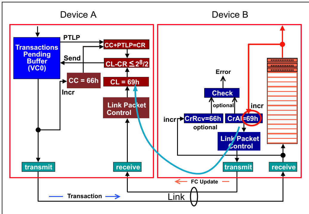
Figure 6-15: Flow Control Update Example
