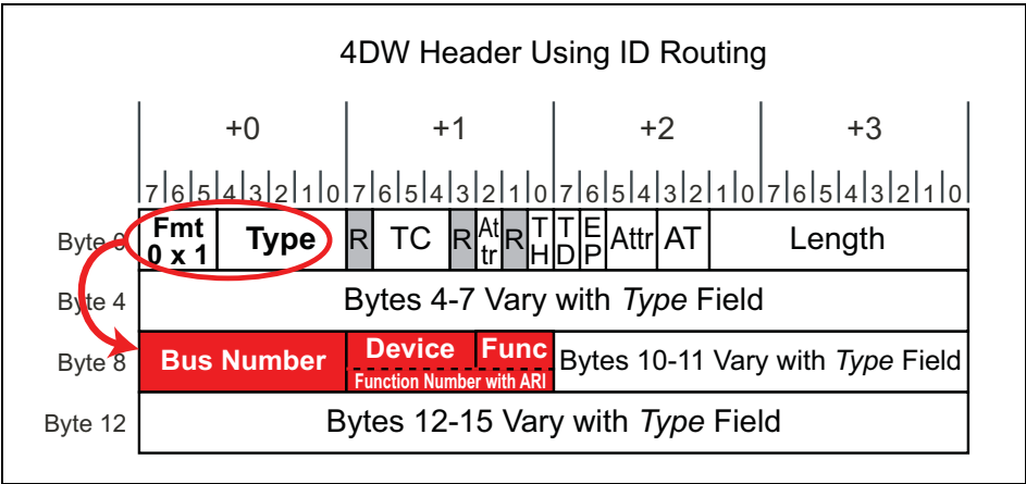
Figure 4-16: 4DW TLP Header - ID Routing Fields
