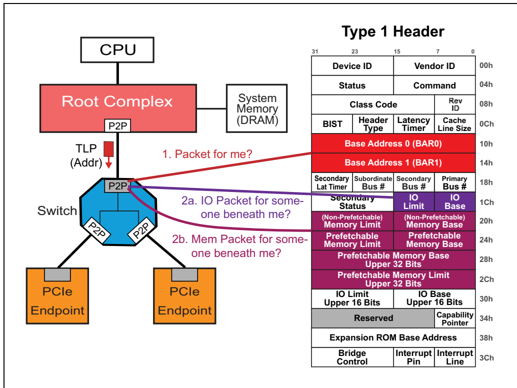
Figure 4-21: Switch Checks Routing Of An Inbound TLP Using Address
