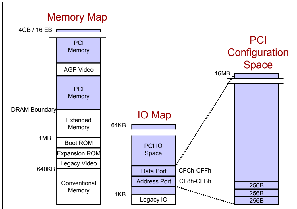
Figure 1-10: Address Space Mapping
