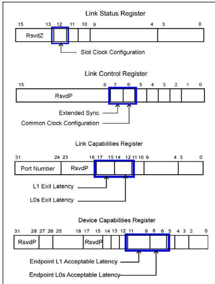
Figure 16-21: Config. Registers for ASPM Exit Latency Management and Reporting
