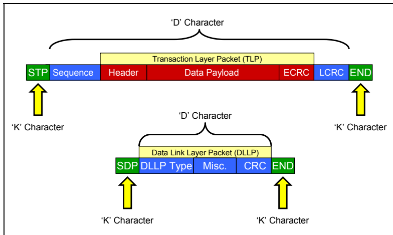
Figure 11-7: TLP and DLLP Packet Framing with Start and End Control Characters
