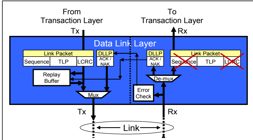
Figure 2-25: Data Link Layer Replay Mechanism
