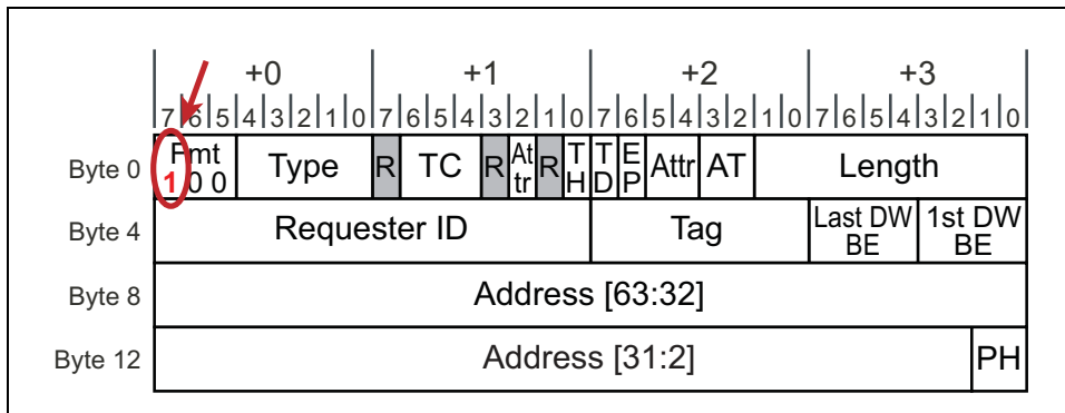
Figure 20-19: TPH Prefix Indication
