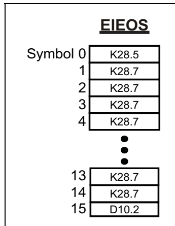
Figure 16-11: Gen1/Gen2 Mode EIEOS Symbol Pattern
