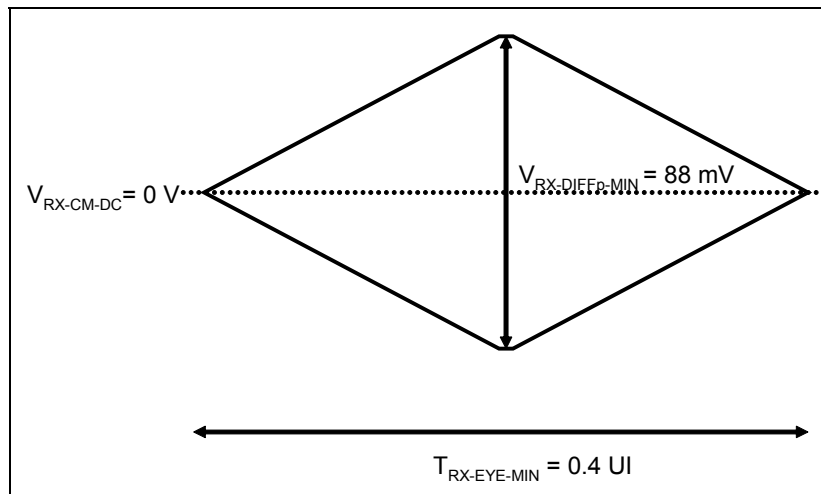
Figure 13-34: 2.5 GT/s Receiver Eye Diagram
