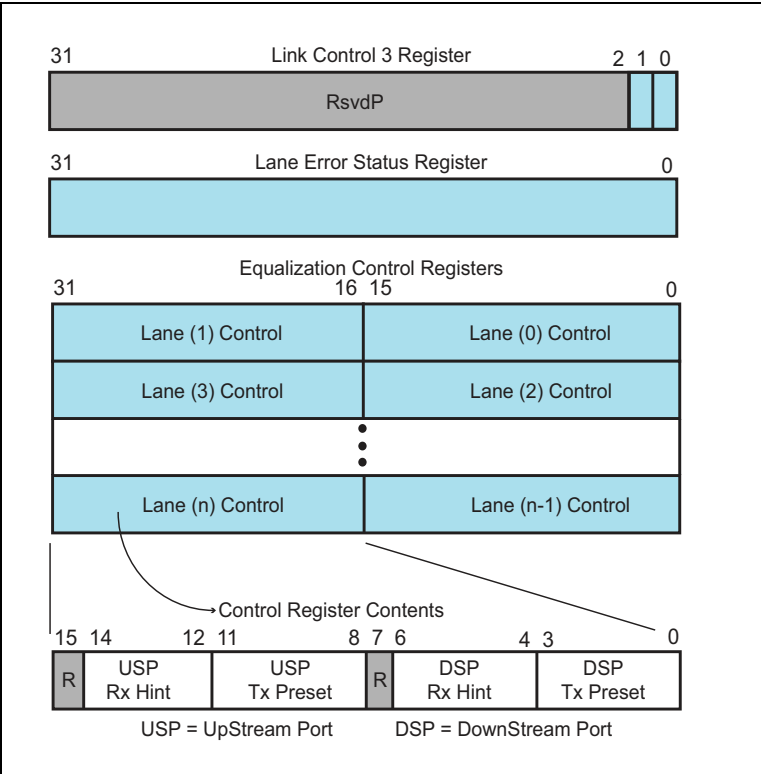
Figure 14-29: Equalization Control Registers
