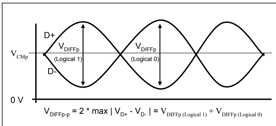
Figure 13-13: Differential Peak-to-Peak ( V_{\text{DIFFP-P}} ) and Peak ( V_{\text{DIFFP}} ) Voltages
