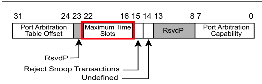
Figure 7-18: Maximum Time Slots Register
