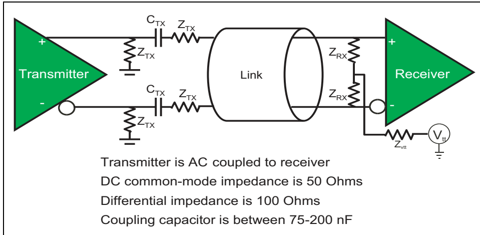
Figure 2-29: Physical Layer Electrical
