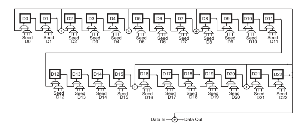
Figure 12-16: Gen3 Per-Lane LFSR Scrambling Logic
