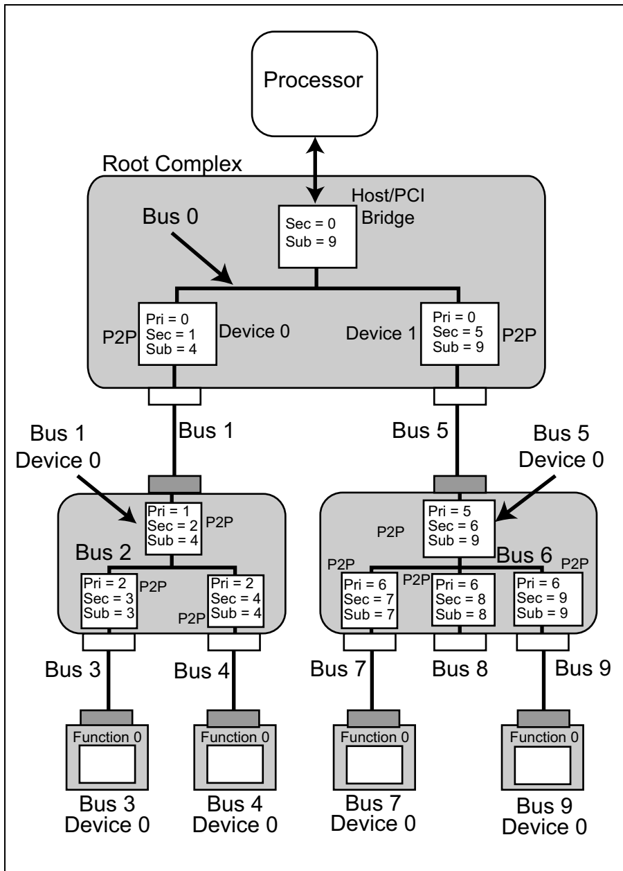
Figure 3-5: Single-Root System
