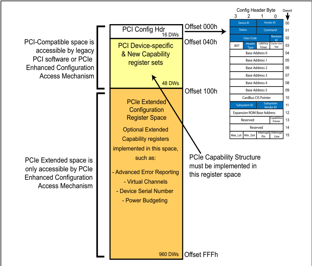
Figure 3-3: 4KB Configuration Space per PCI Express Function
