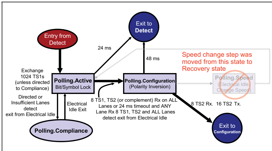
Figure 14-10: Polling State Machine with Legacy Speed Change
