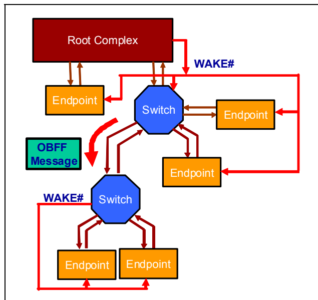
Figure 16-33: OBFF Signaling Example
