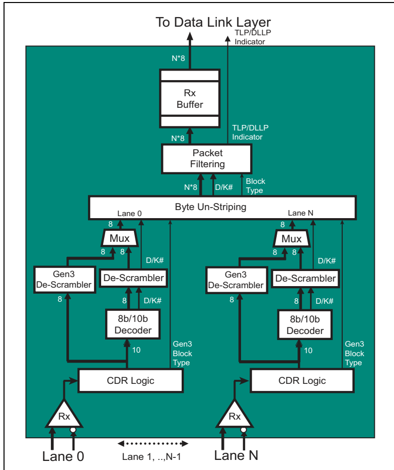
Figure 11-4: Physical Layer Receive Logic Details
