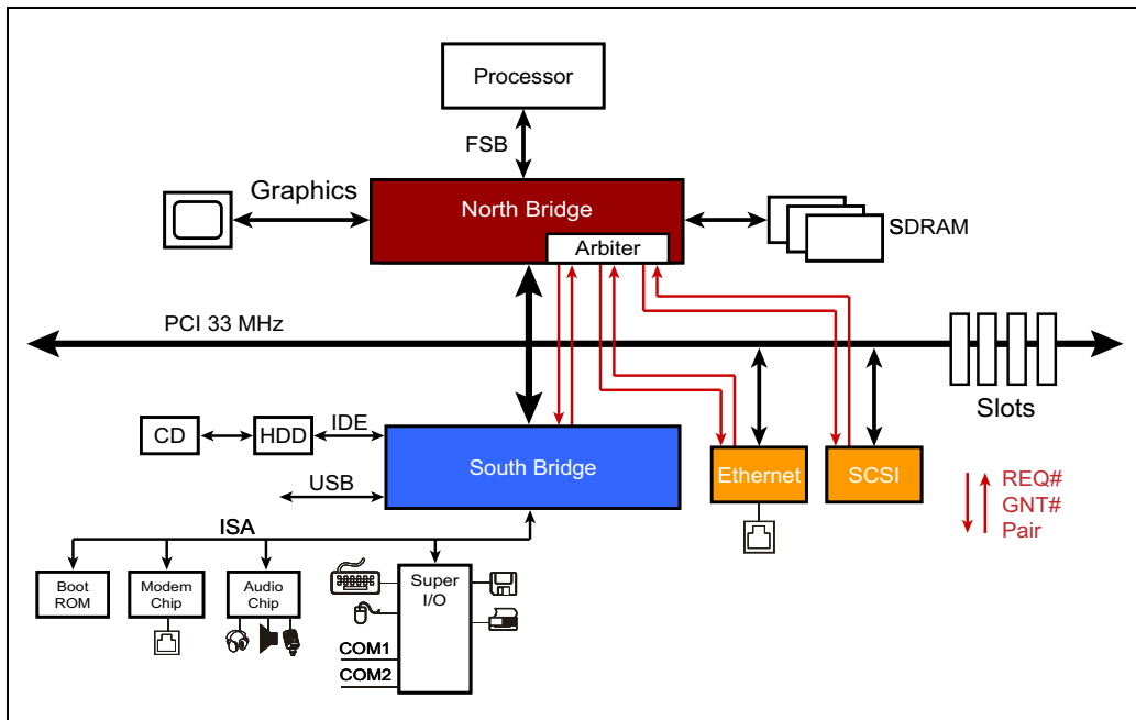
Figure 1-2: PCI Bus Arbitration
