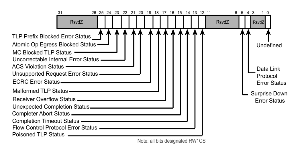
Figure 15-25: Advanced Uncorrectable Error Status Register
