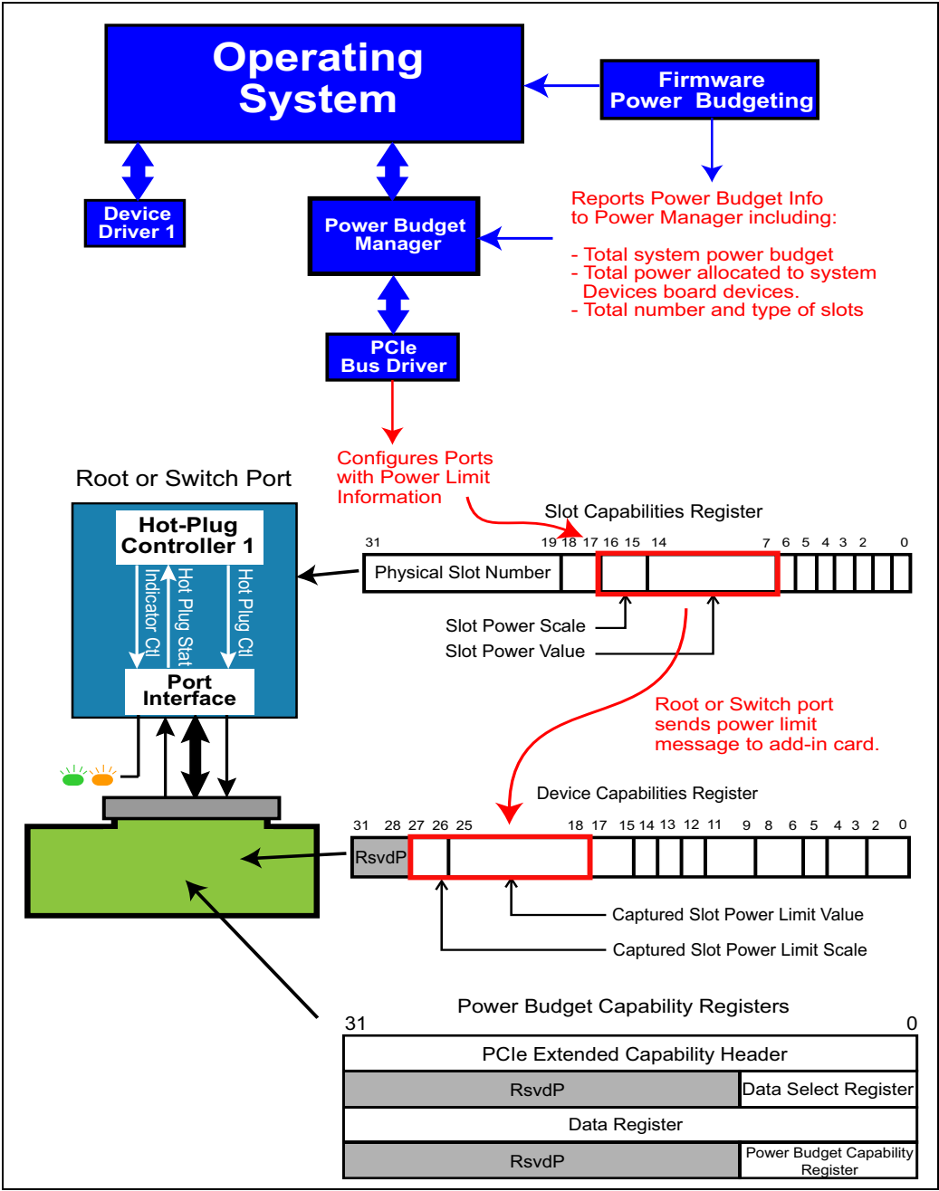
Figure 19-10: Elements Involved in Power Budget
