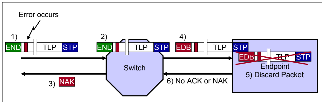
Figure 10-16: Switch Cut-Through Mode Showing Error Handling
