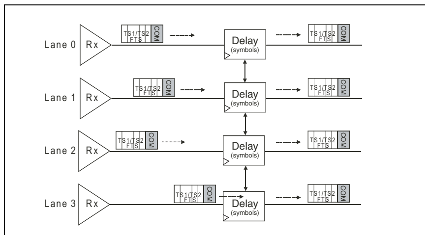
Figure 11-23: Receiver's Link De-Skew Logic
