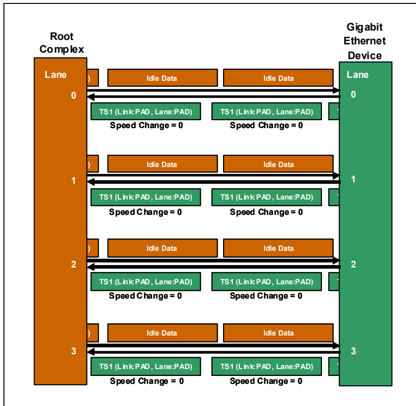
Figure 14-63: Link Width Change - Recovery.Idle
