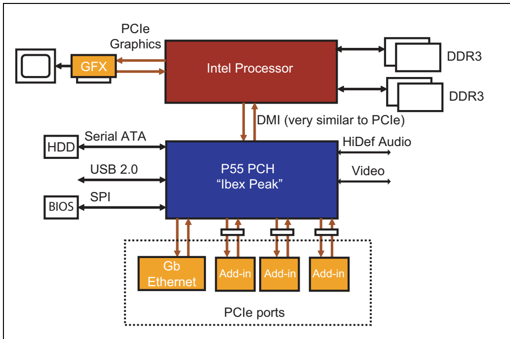
Figure 2-10: Low-Cost PCIe System
