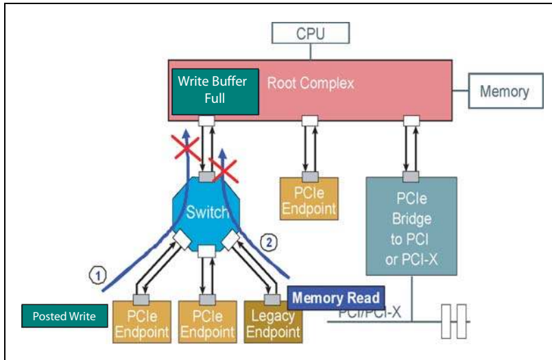
Figure 8-7: Different Sources are Unlikely to Have Dependencies
