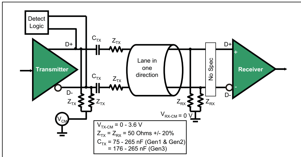
Figure 13-2: Differential Transmitter/Receiver
