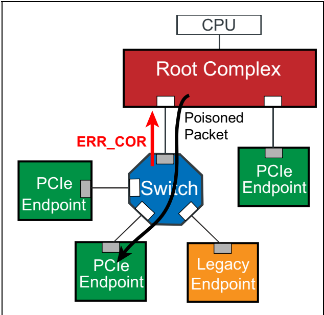
Figure 15-11: Role-Based Error Reporting Example
