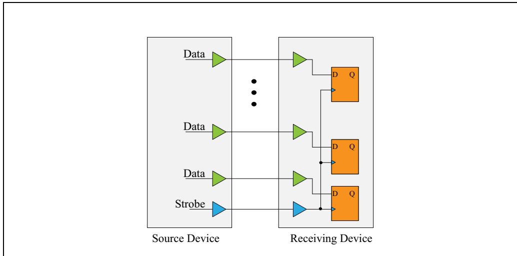
Figure 1-19: Source-Synchronous Clocking Model
