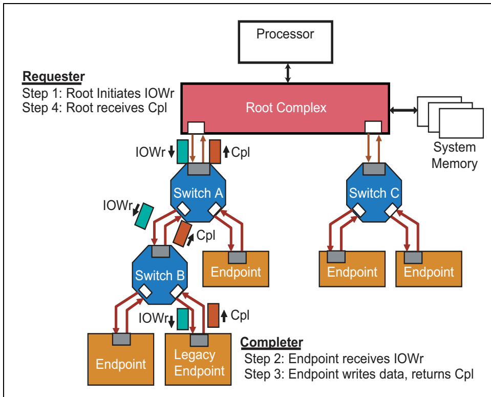
Figure 2-20: Non-Posted Write Transaction Protocol
