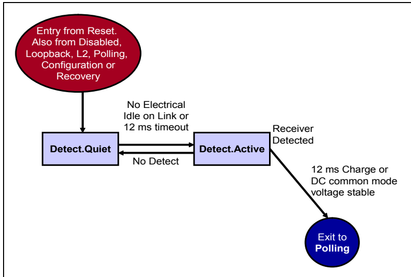
Figure 14-8: Detect State Machine
