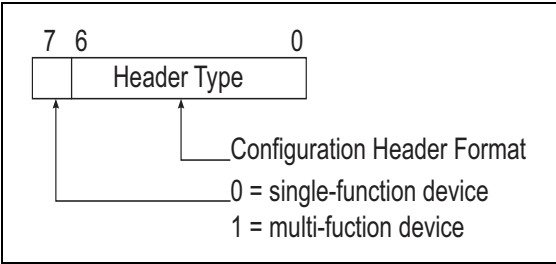
Figure 3-12: Header Type Register
