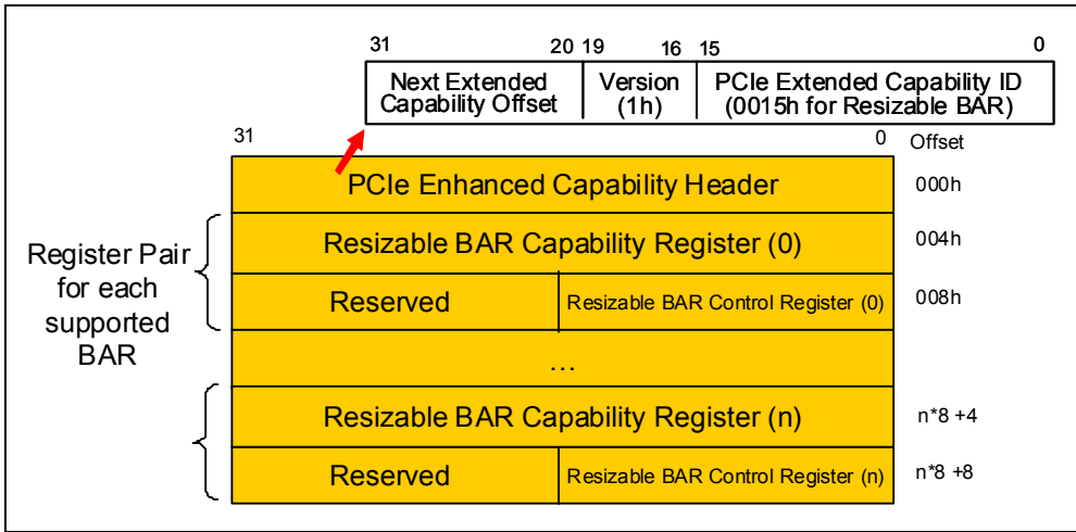
Figure 20-20: Resizable BAR Registers
