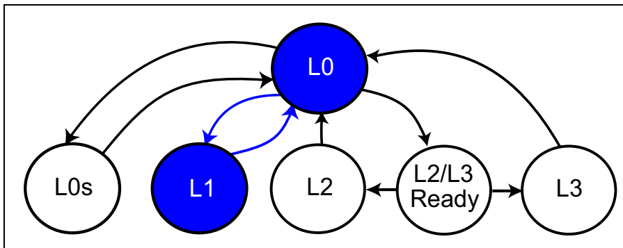
Figure 16-23: Devices Transition to L1 When Software Changes their Power Level from D0
