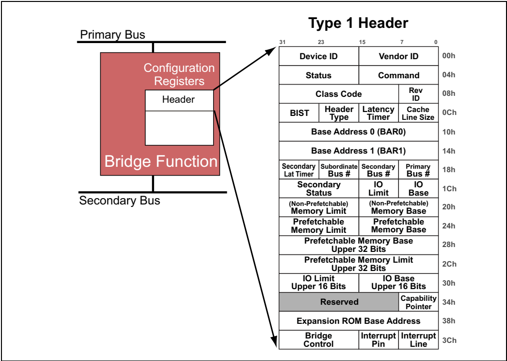
Figure 1-12: PCI Configuration Header Type 1 (Bridge)
