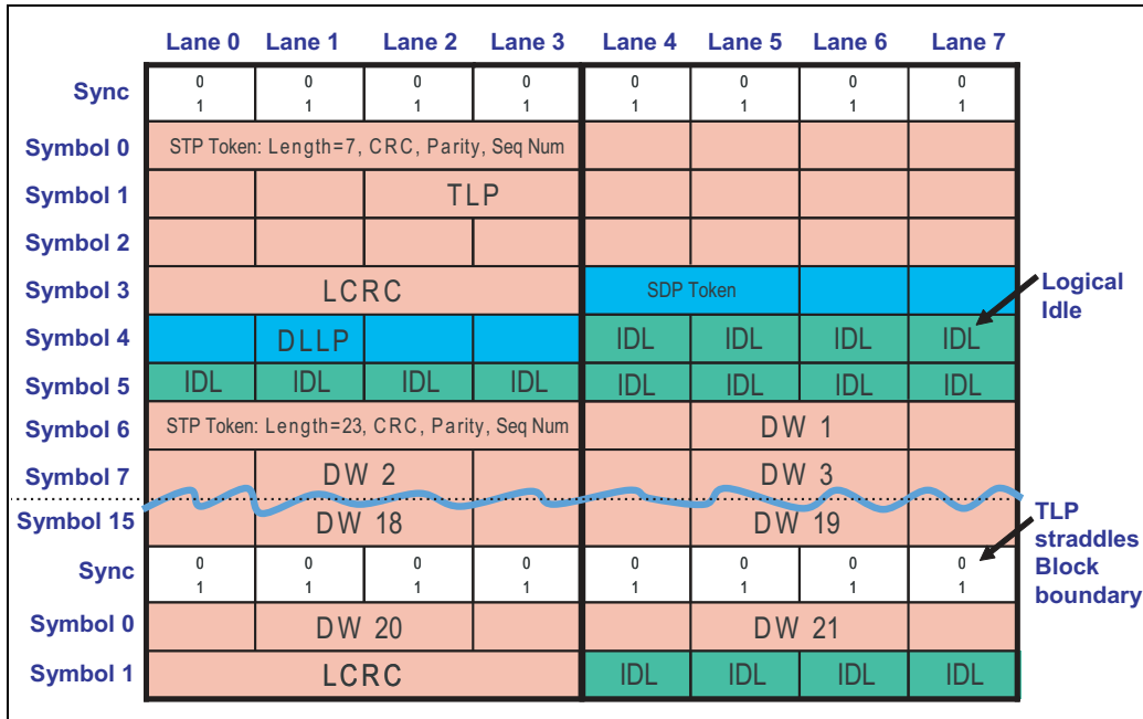
Figure 12-12: Gen3 x8 Example: TLP Straddles Block Boundary
