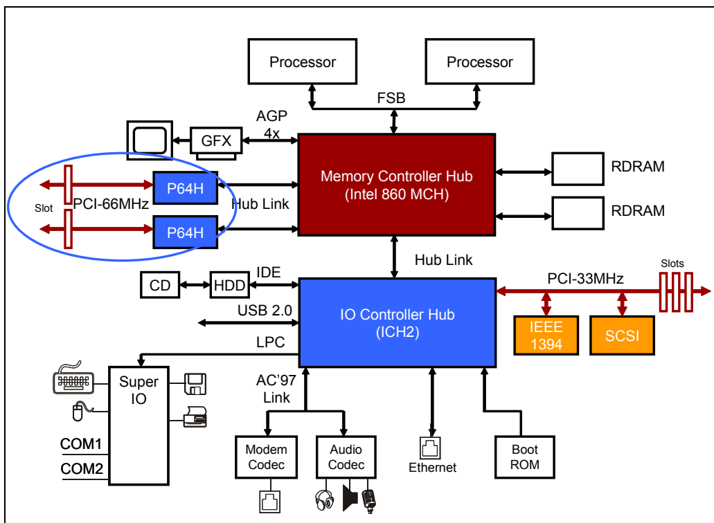
Figure 1-14: 66 MHz PCI Bus Based Platform
