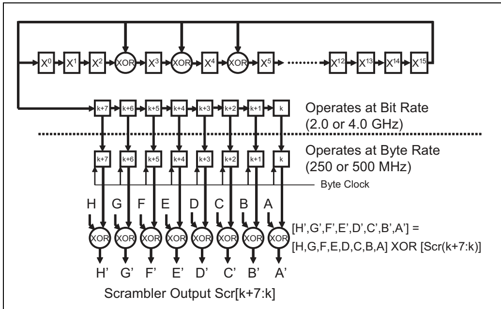
Figure 11-14: Scrambler
