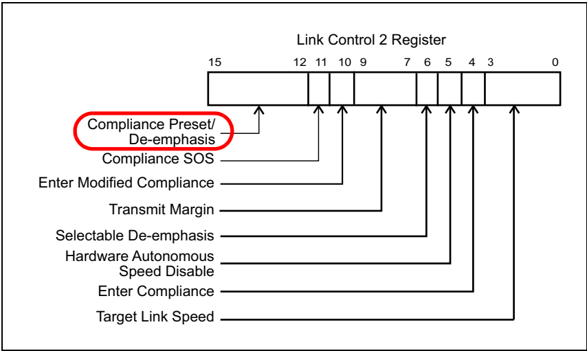
Figure 14-11: Link Control 2 Register
