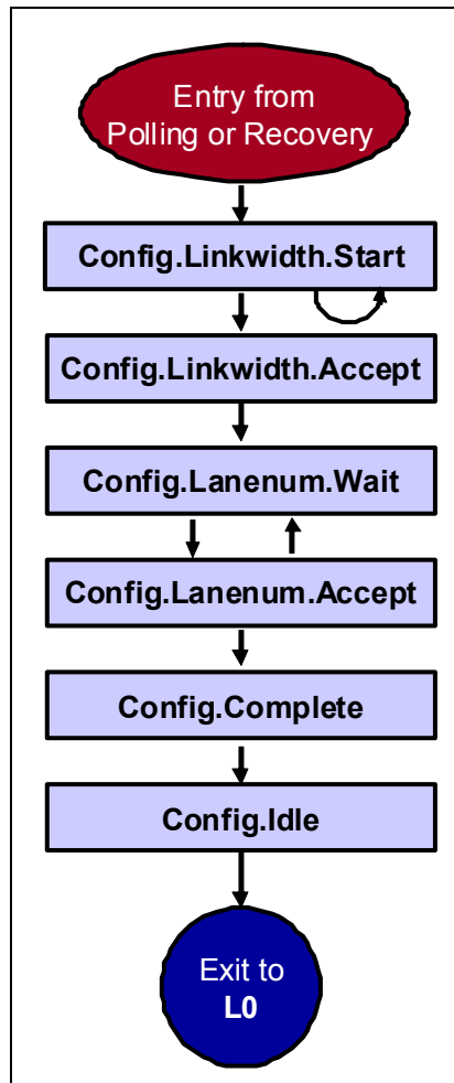
Figure 14-61: Simplified Configuration Substates
