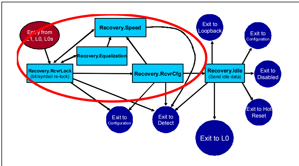
Figure 14-48: Recovery Sub-States
