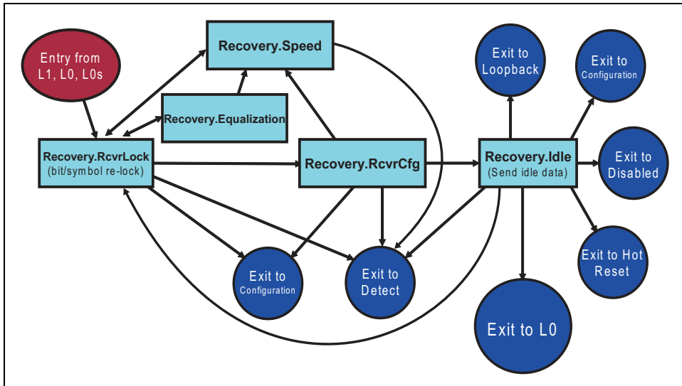
Figure 14-27: Recovery State Machine
