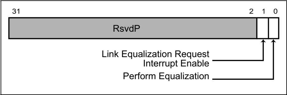
Figure 14-37: Link Control 3 Register
