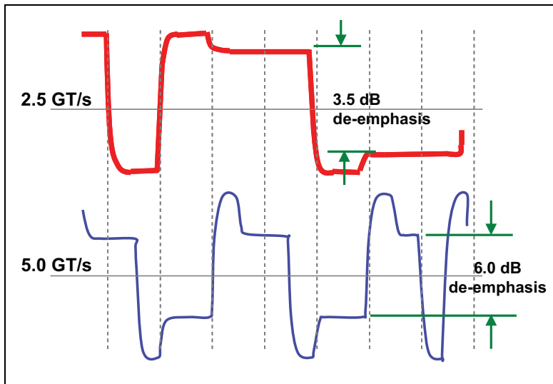
Figure 13-19: De-emphasis Options for 5.0 GT/s
