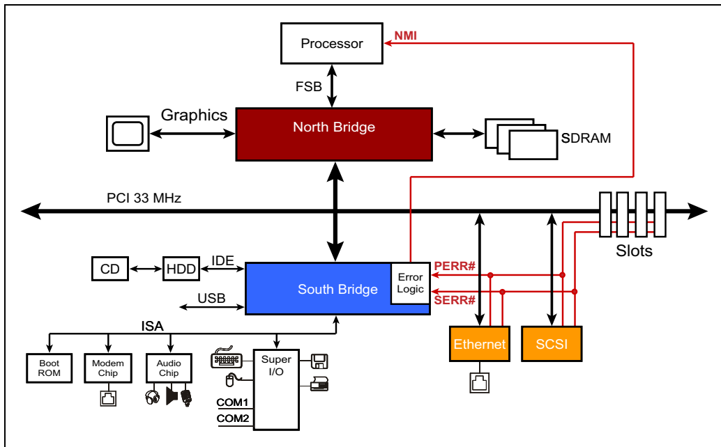
Figure 1-9: PCI Error Handling
