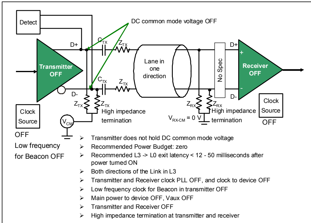
Figure 13-39: L3 Link Off State
