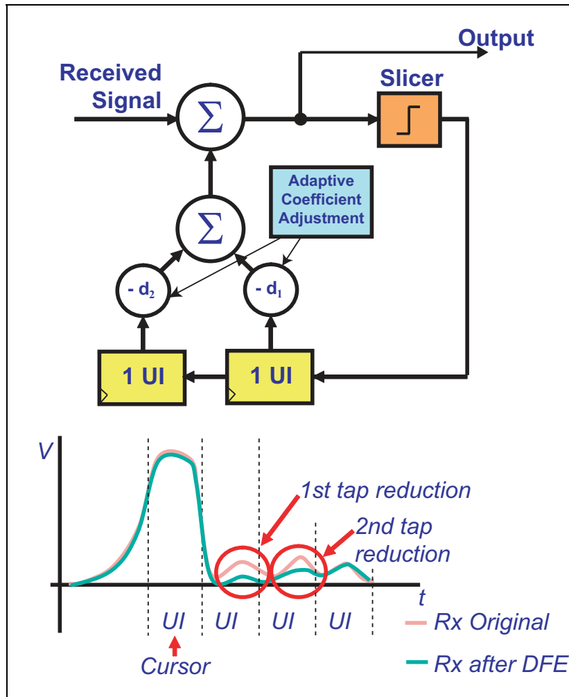
Figure 13-33: Rx 2-Tap DFE
