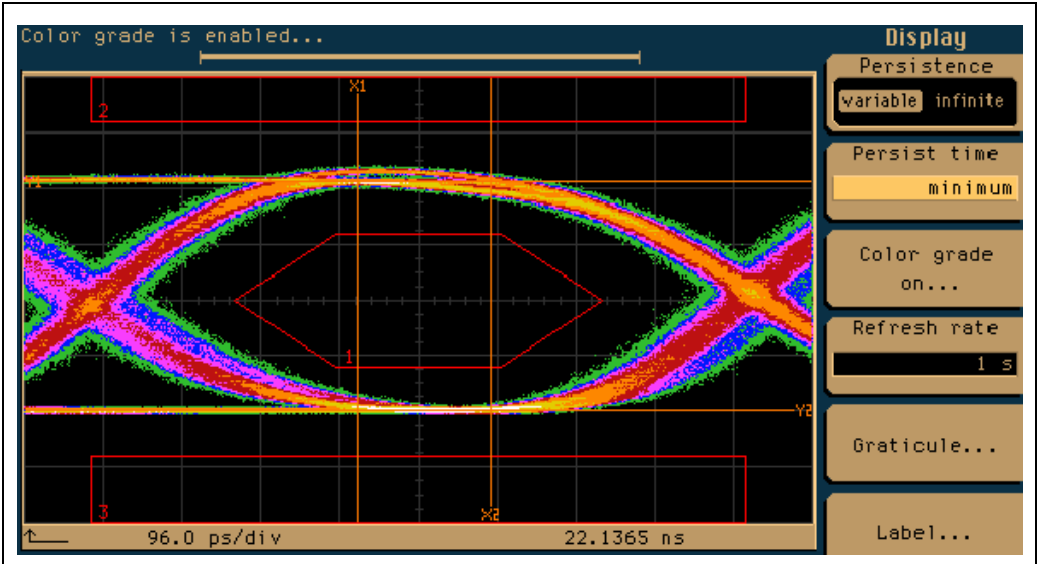
Figure 13-28: Rx Bad Eye (No De-emphasis)
