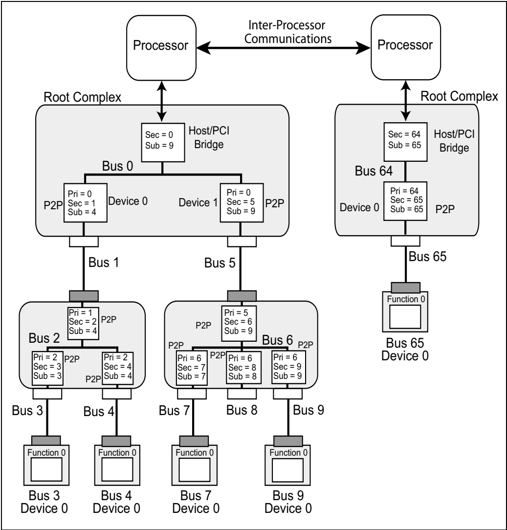
Figure 3-14: Multi-Root System
