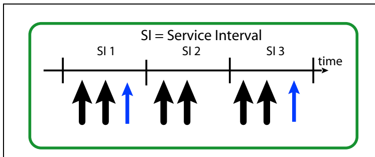
Figure 7-25: Injection of Isochronous Packets
