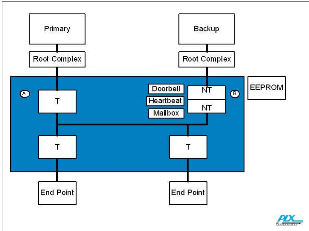
Figure 0-5: Host Failover in PCI and PCI Express Systems
