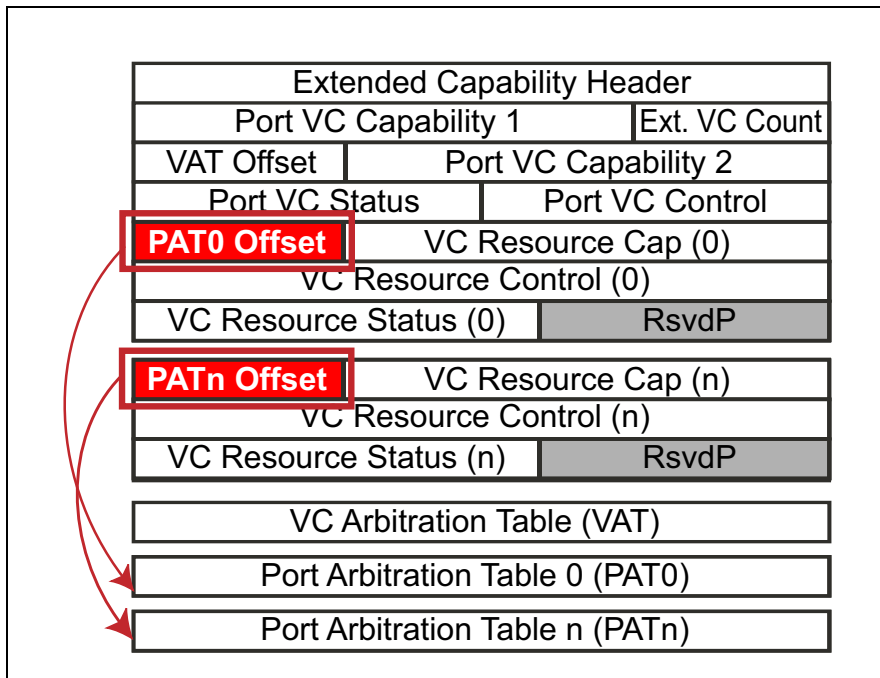
Figure 7-15: Port Arbitration Tables for Each VC
