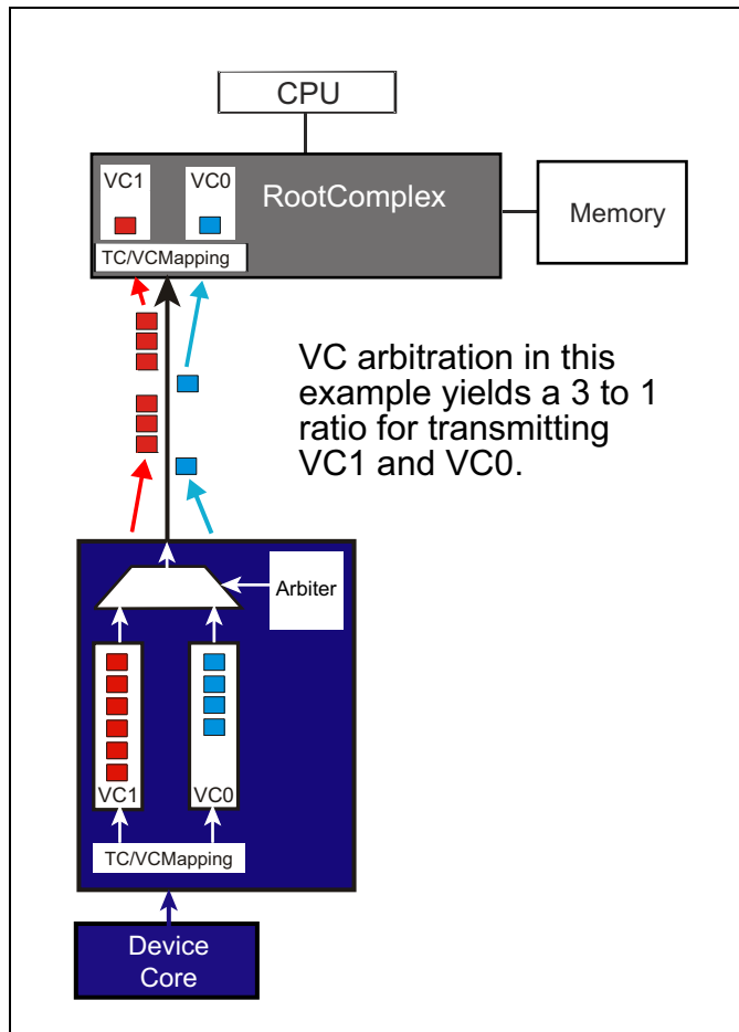
Figure 7-6: VC Arbitration Example
