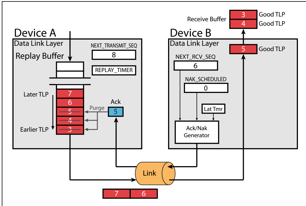
Figure 10-8: Example 1 - Example of Ack
