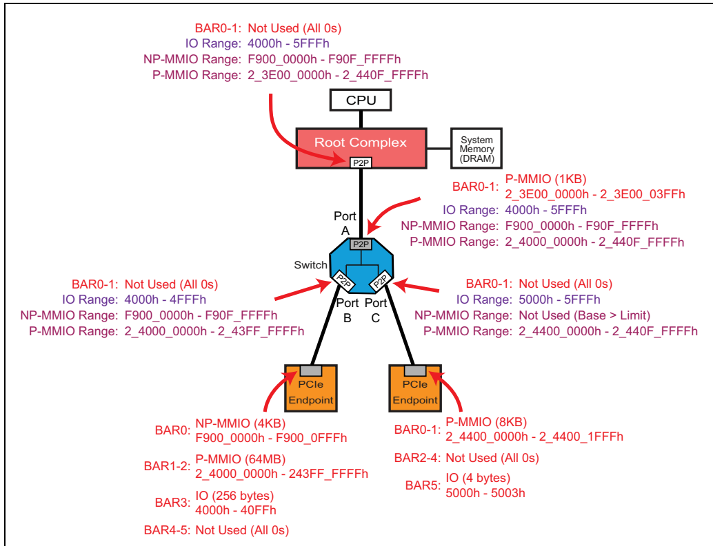
Figure 4-11: Final Example Address Routing Setup
