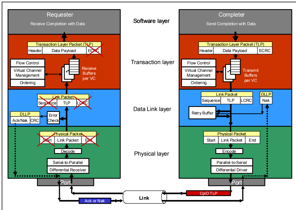
Figure 2-33: Completion with Data Phase
