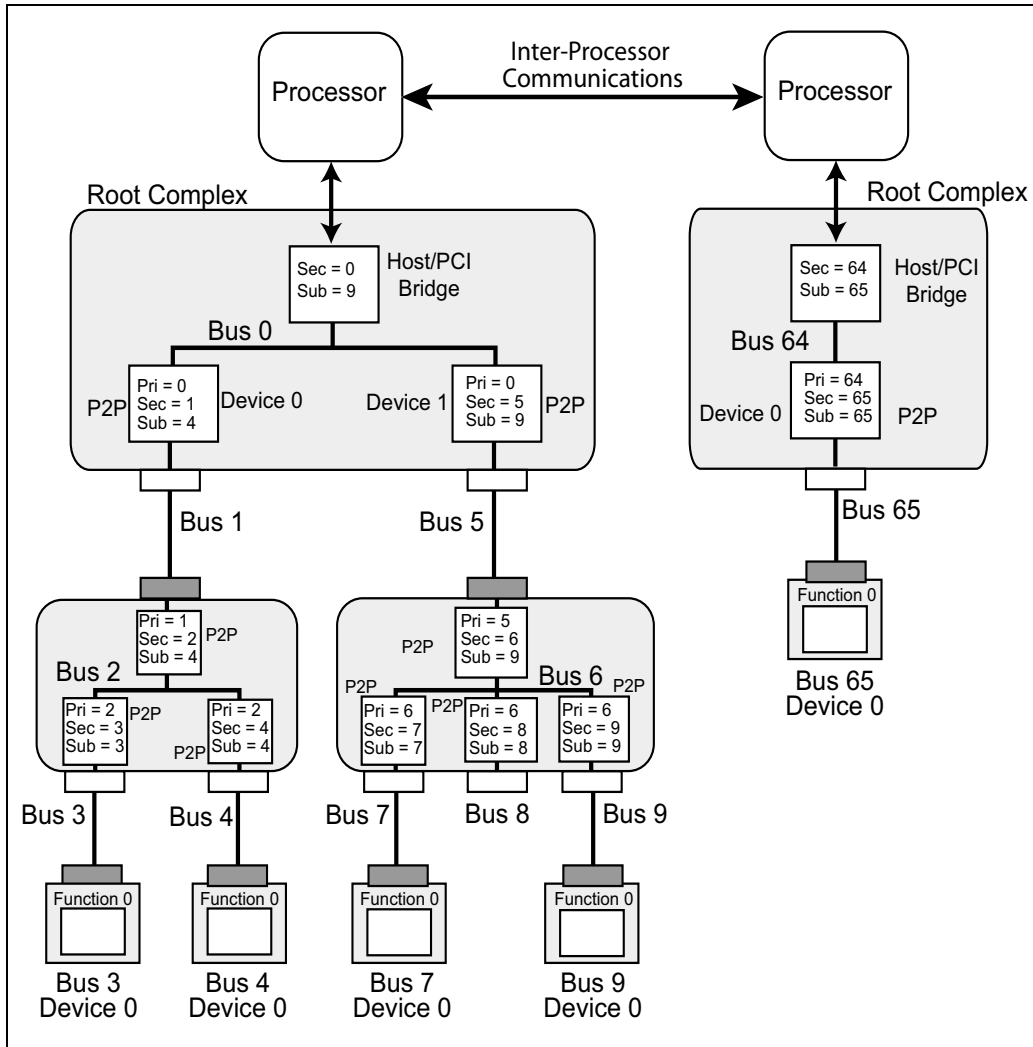
Figure 3-6: Multi-Root System
