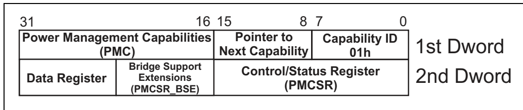
Figure 16-2: PCI Power Management Capability Register Set
