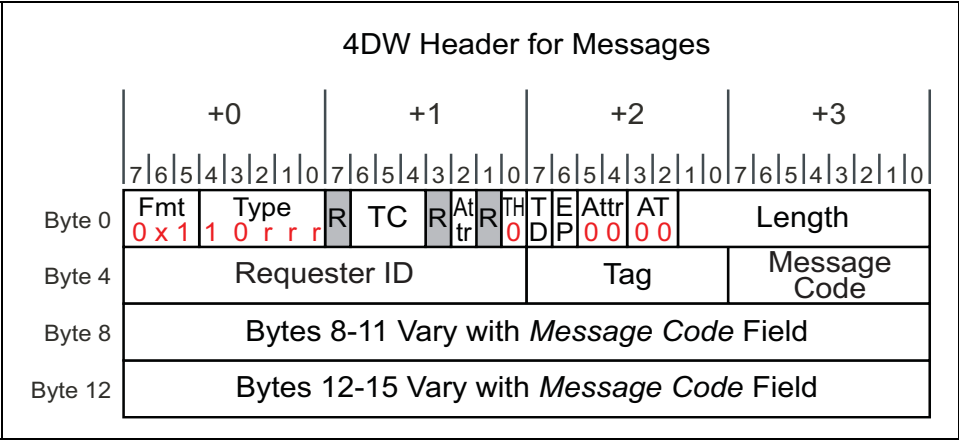
Figure 5-11: 4DW Message Request Header Format
