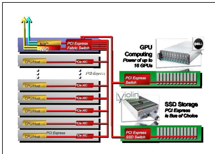
Figure 0-3: PCIe in a Data Center for HPC Applications
