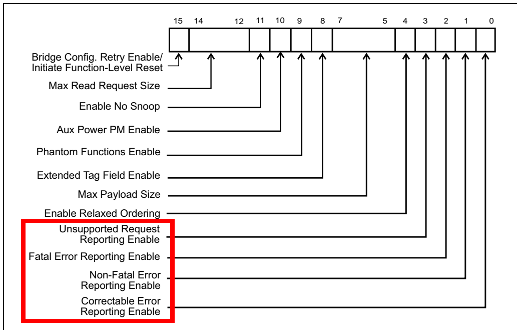
Figure 15-16: Device Control Register Fields Related to Error Handling
