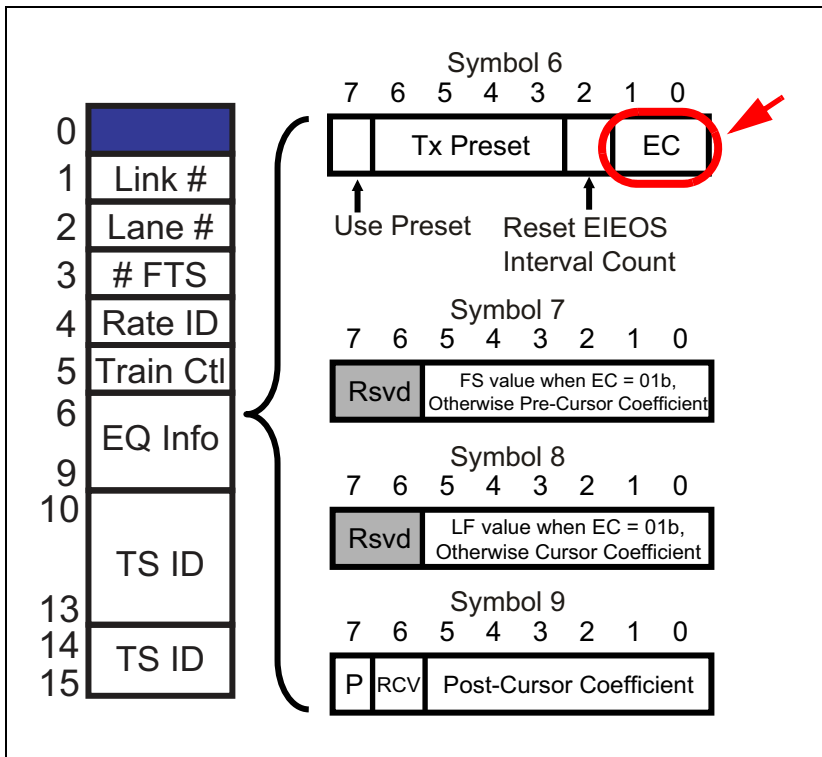
Figure 14-28: EC Field in TS1s and TS2s for 8.0 GT/s
