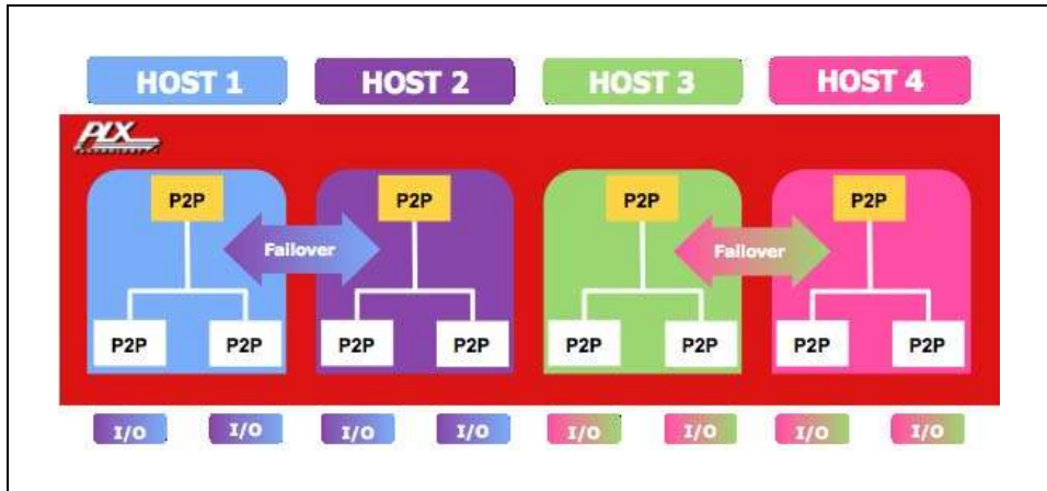
Figure 0-2: MR-IOV Switch Internal Architecture
