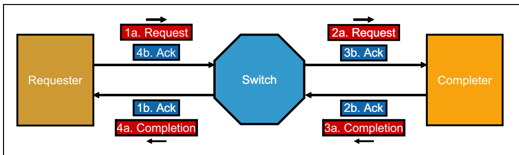
Figure 2-27: Non-Posted Transaction with Ack/Nak Protocol
