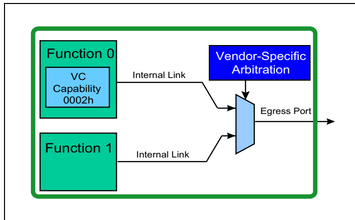
Figure 7-21: Simple Multi-Function Arbitration
