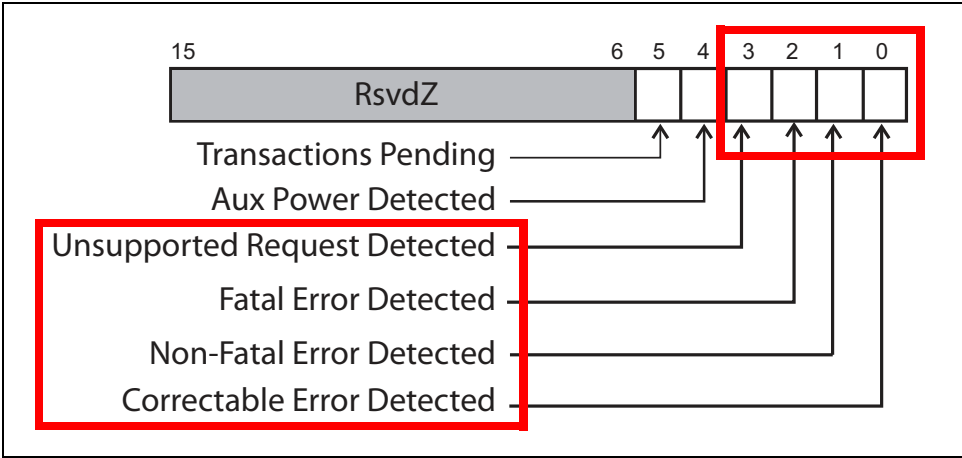
Figure 15-17: Device Status Register Bit Fields Related to Error Handling
