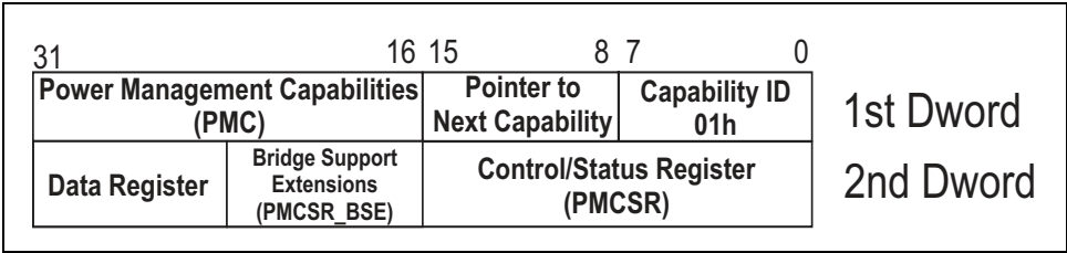
Figure 16-7: PCI Function’s PM Registers
