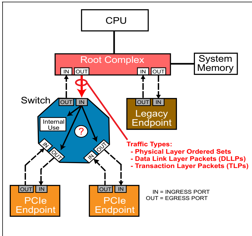
Figure 4-12: Multi-Port PCIe Devices Have Routing Responsibilities
