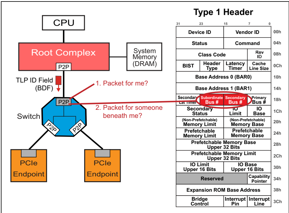
Figure 4-17: Switch Checks Routing Of An Inbound TLP Using ID Routing
