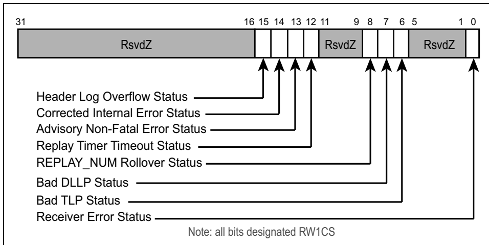
Figure 15-23: Advanced Correctable Error Status Register
