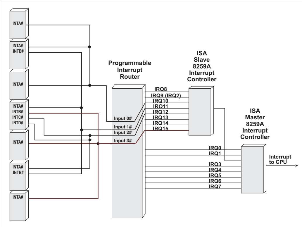
Figure 17-6: INTx Signal Routing is Platform Specific
