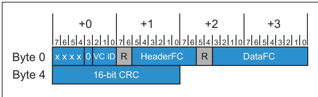
Figure 9-5: Flow Control DLLP Format
