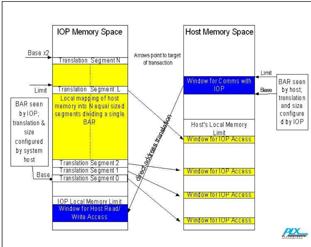
Figure 0-3: Look Up Table Translation Creates Multiple Windows
