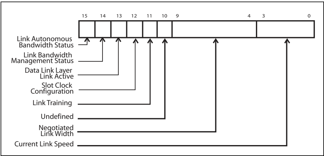
Figure 14-70: Link Status Register
