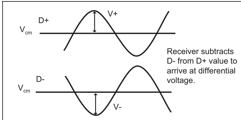
Figure 13-12: Differential Signaling
