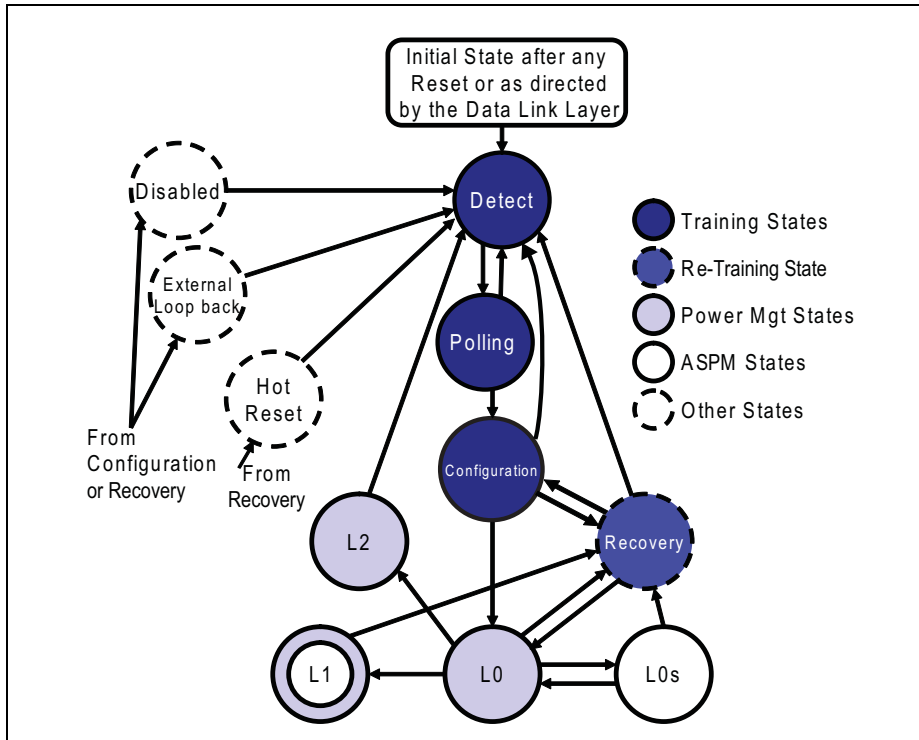
Figure 14-6: Link Training and Status State Machine (LTSSM)
