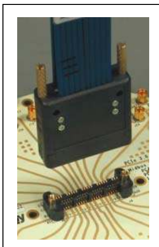
Figure A-4: LeCroy PCI Express Gen3 Mid-Bus Probe
