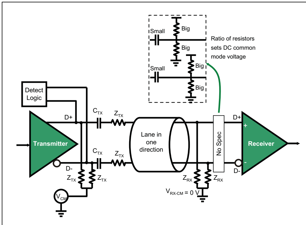
Figure 13-15: Receiver DC Common-Mode Voltage Adjustment
