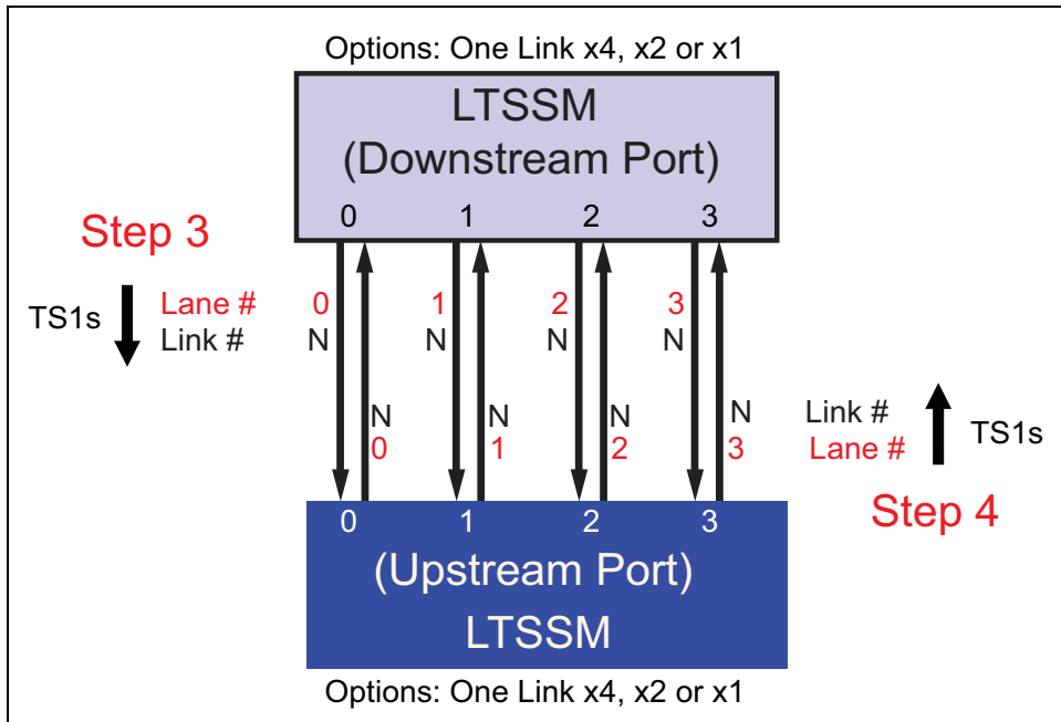
Figure 14-16: Example 1 - Steps 3 and 4
