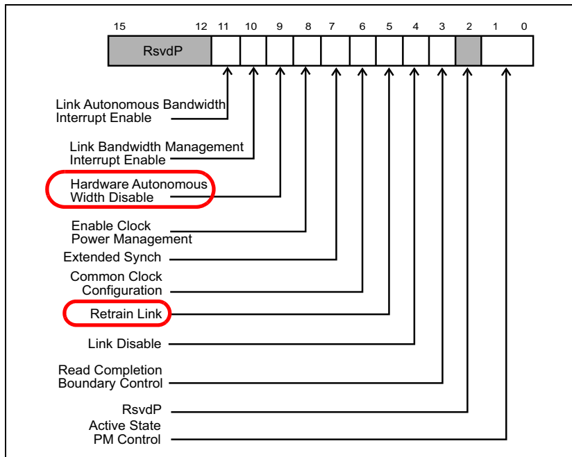
Figure 14-25: Link Control Register
