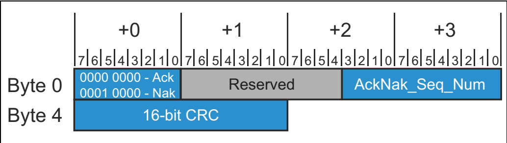
Figure 10-7: Ack Or Nak DLLP Format
