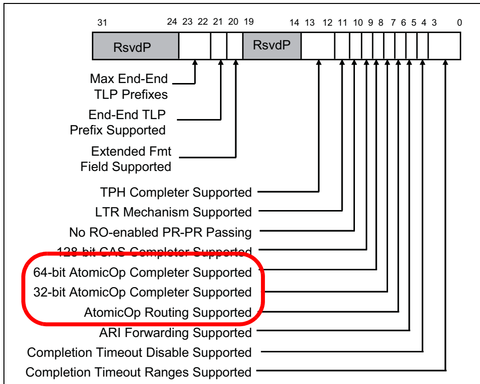
Figure 20-10: Device Capabilities 2 Register
