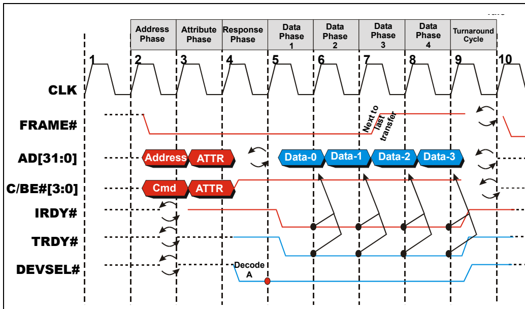
Figure 1-16: Example PCI-X Burst Memory Read Bus Cycle
