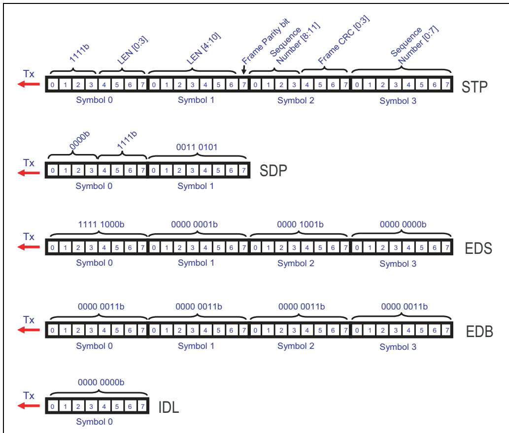
Figure 12-8: Gen3 Frame Token Examples
