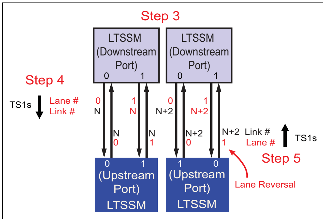
Figure 14-20: Example 2 - Steps 3, 4 and 5
