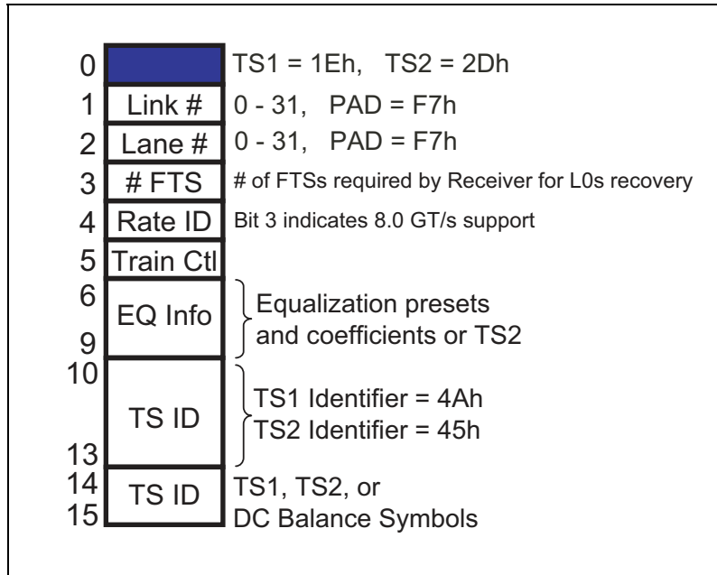
Figure 14-5: TS1 and TS2 Ordered Set Block When In Gen3 Mode of Operation
