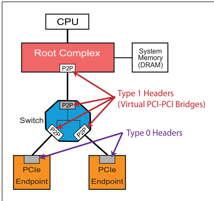
Figure 4-3: PCI Express Devices And Type 0 And Type 1 Header Use
