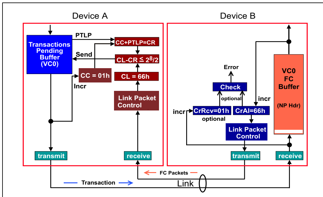
Figure 6-11: Flow Control Elements After First TLP Sent
