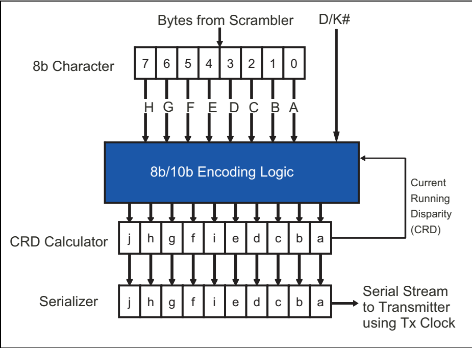
Figure 11-17: 8-bit to 10-bit (8b/10b) Encoder
