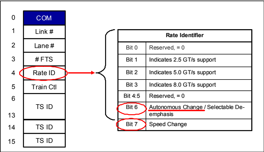
Figure 14-47: TS2 Contents
