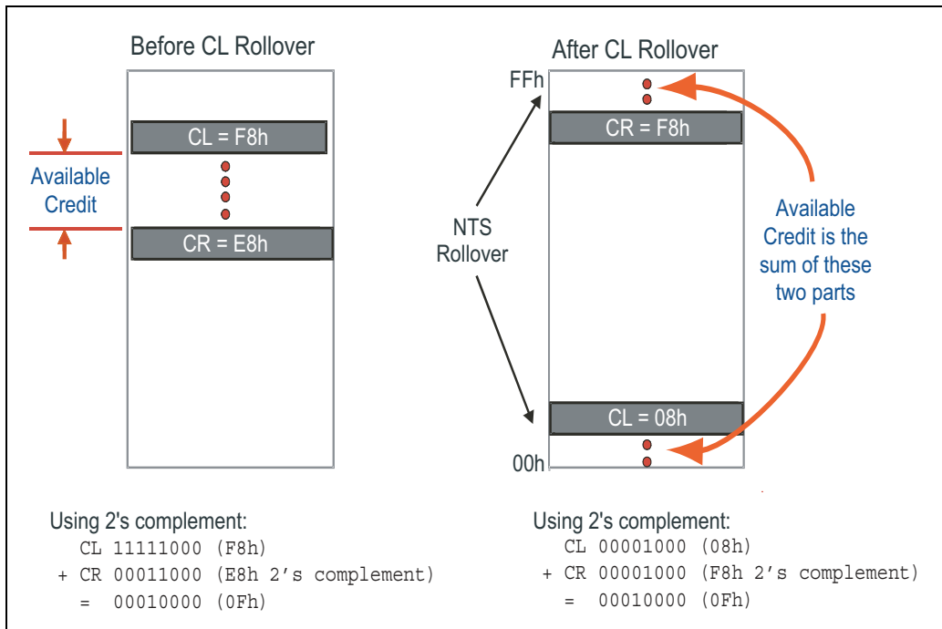
Figure 6-13: Flow Control Rollover Problem
