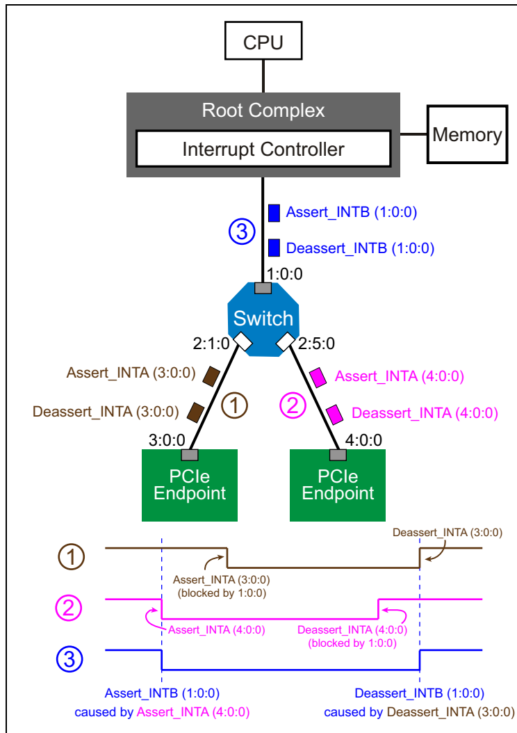
Figure 17-12: Switch Uses Bridge Mapping of INTx Messages
