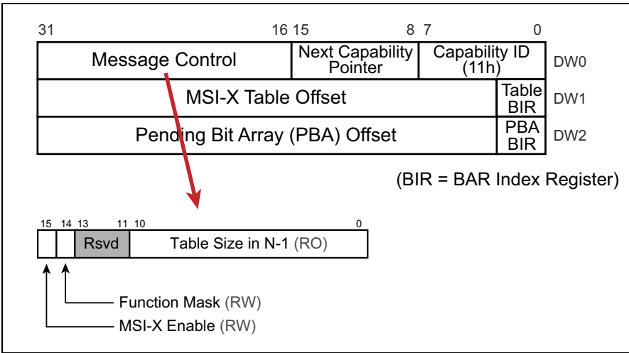
Figure 17-17: MSI-X Capability Structure
