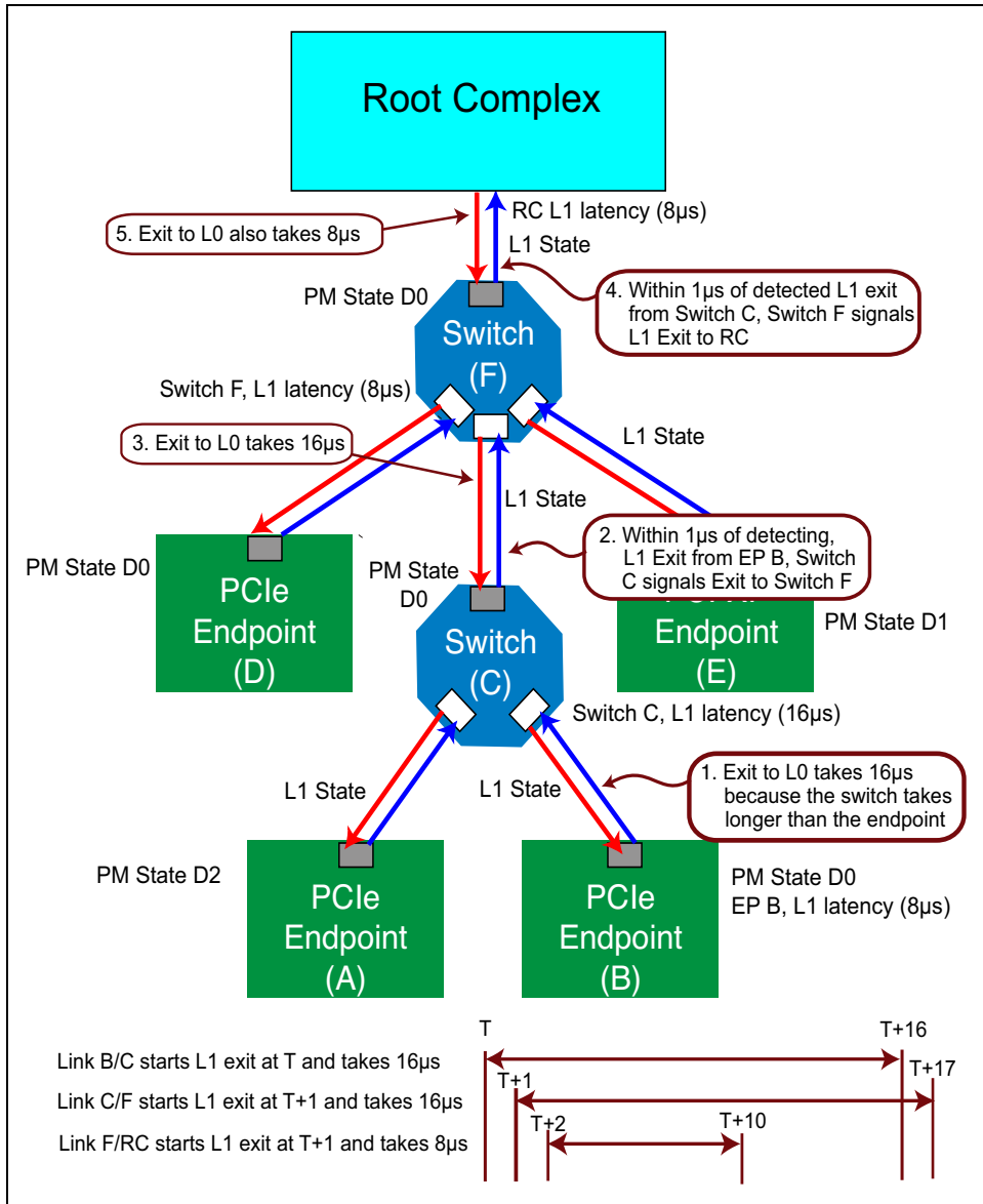
Figure 16-22: Example of Total L1 Latency
