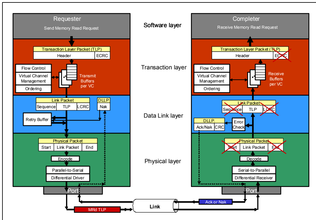
Figure 2-32: Memory Read Request Phase
