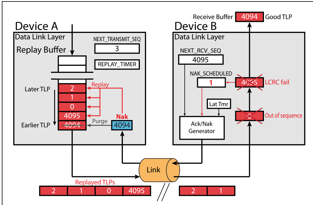
Figure 10-10: Example of a Nak
