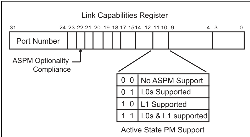
Figure 16-14: ASPM Support
