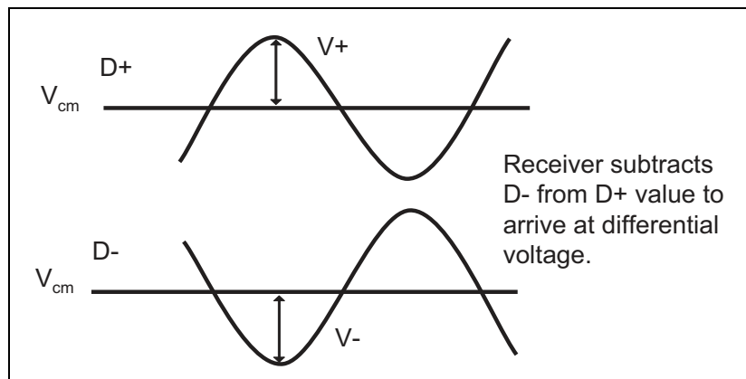
Figure 2-4: Differential Signaling
