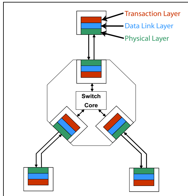
Figure 2-13: Switch Port Layers
