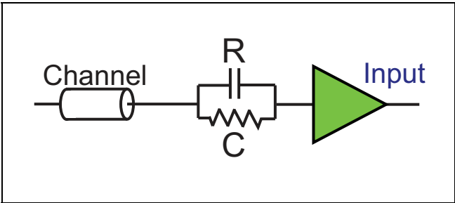
Figure 13-30: Rx Continuous-Time Linear Equalizer (CTLE)
