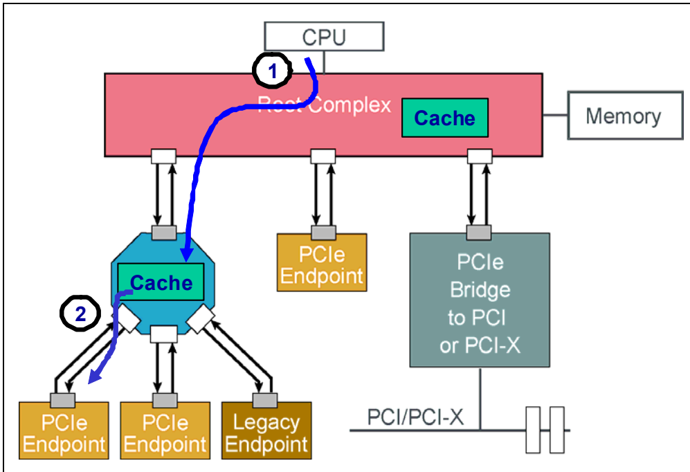
Figure 20-13: TPH Usage for TLPs to Endpoint
