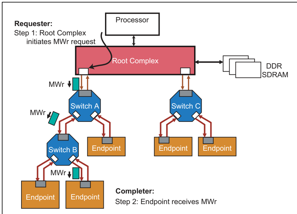
Figure 2-21: Posted Memory Write Transaction Protocol
