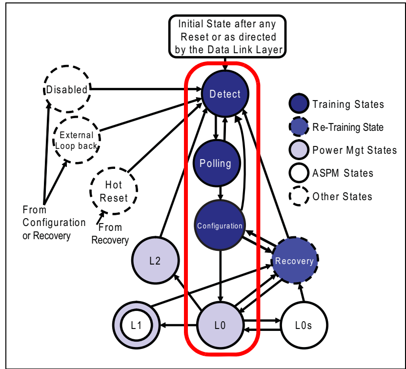
Figure 14-7: States Involved in Initial Link Training at 2.5 Gb/s
