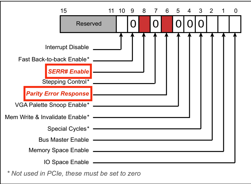
Figure 15-13: Command Register in Configuration Header
