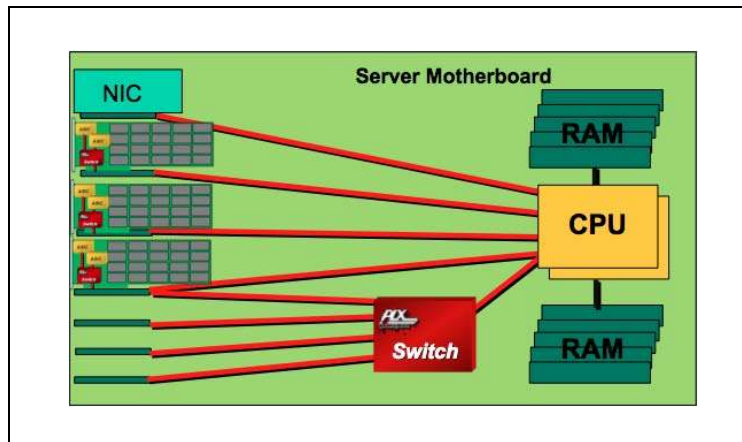
Figure 0-5: Server Motherboard Use PCIe Switches
