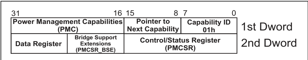
Figure 16-8: PM Registers
