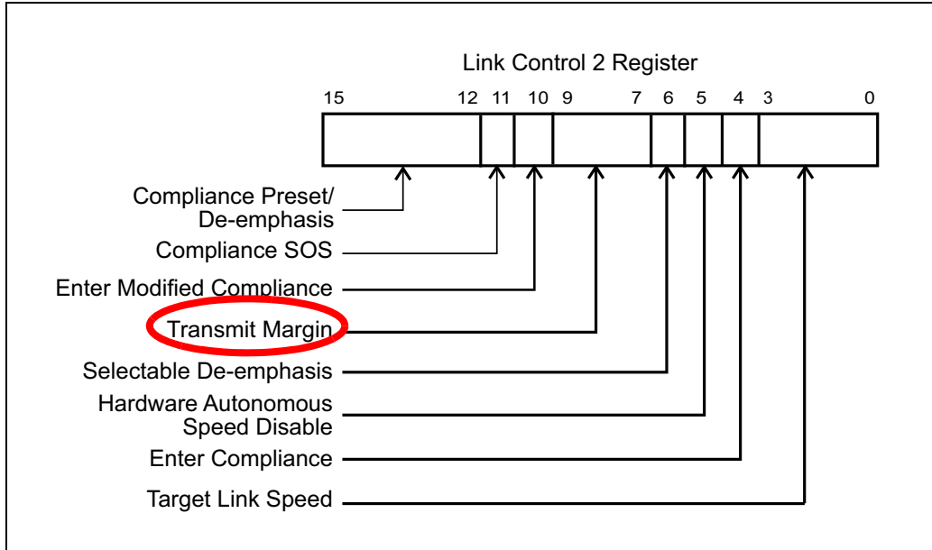
Figure 13-14: Transmit Margin Field in Link Control 2 Register
