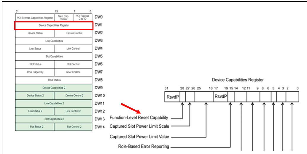
Figure 18-8: Function-Level Reset Capability
