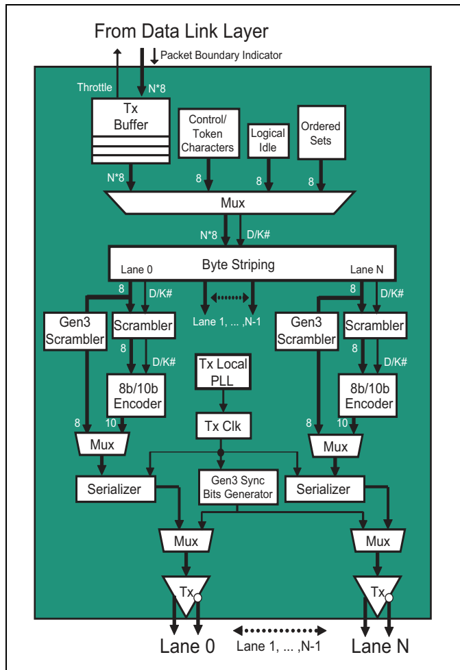
Figure 11-3: Physical Layer Transmit Details
