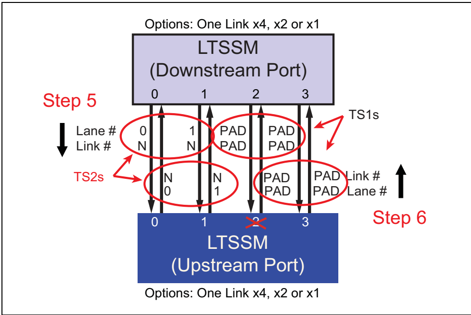
Figure 14-23: Example 3 - Steps 5 and 6
