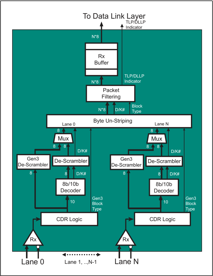
Figure 12-18: Gen3 Physical Layer Receiver Details
