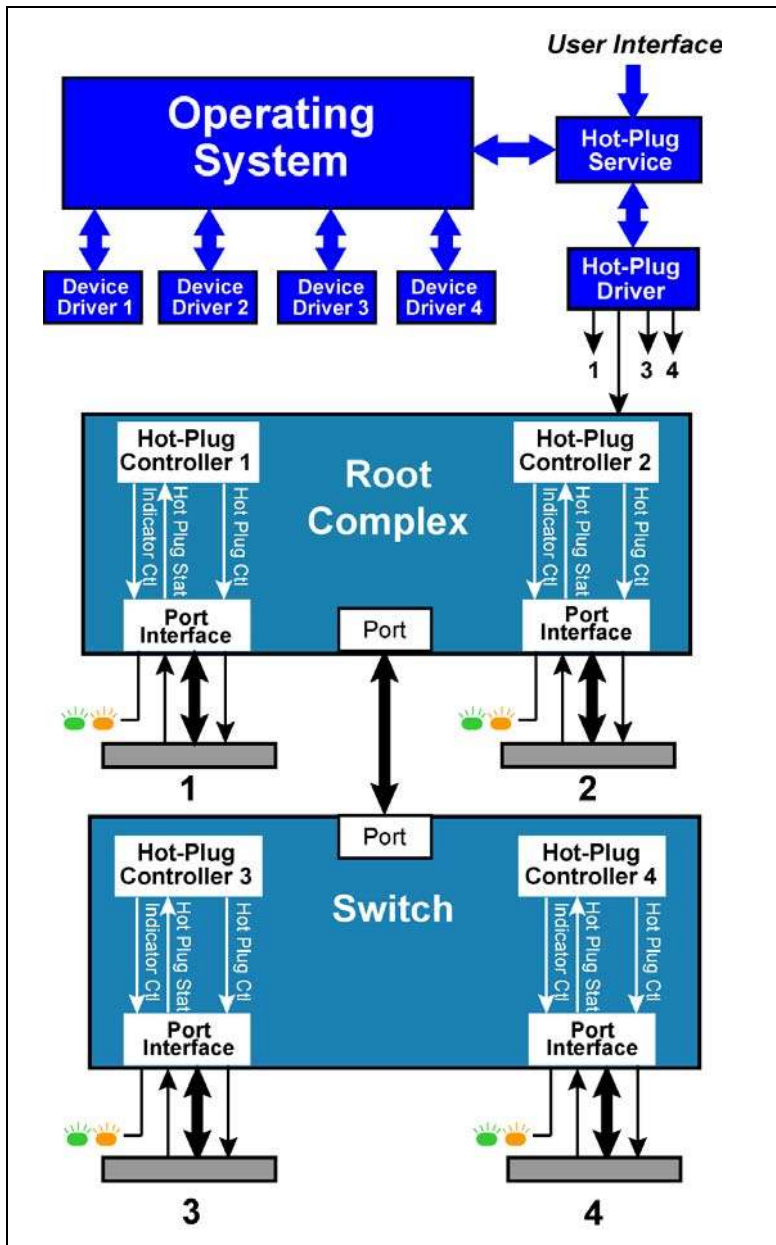
Figure 19-2: PCI Express Hot-Plug Elements
