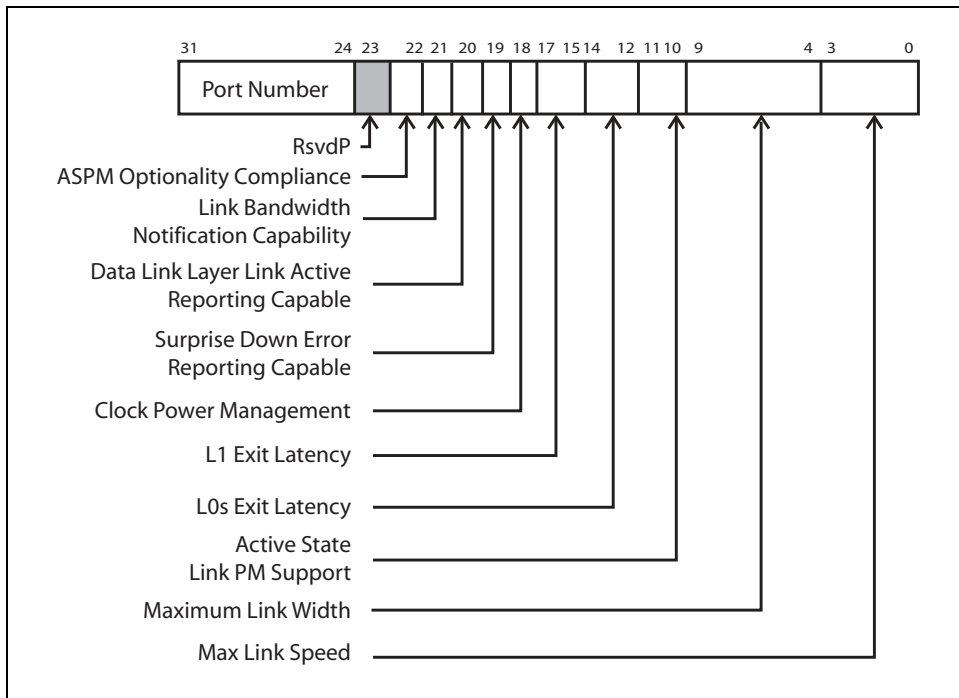
Figure 14-68: Link Capabilities Register
