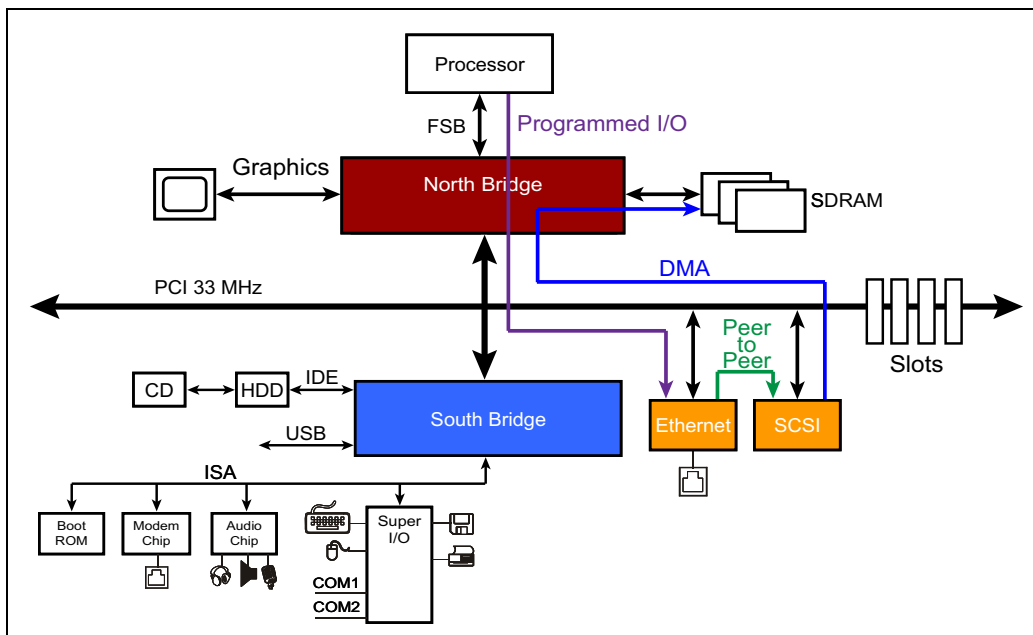
Figure 1-6: PCI Transaction Models
