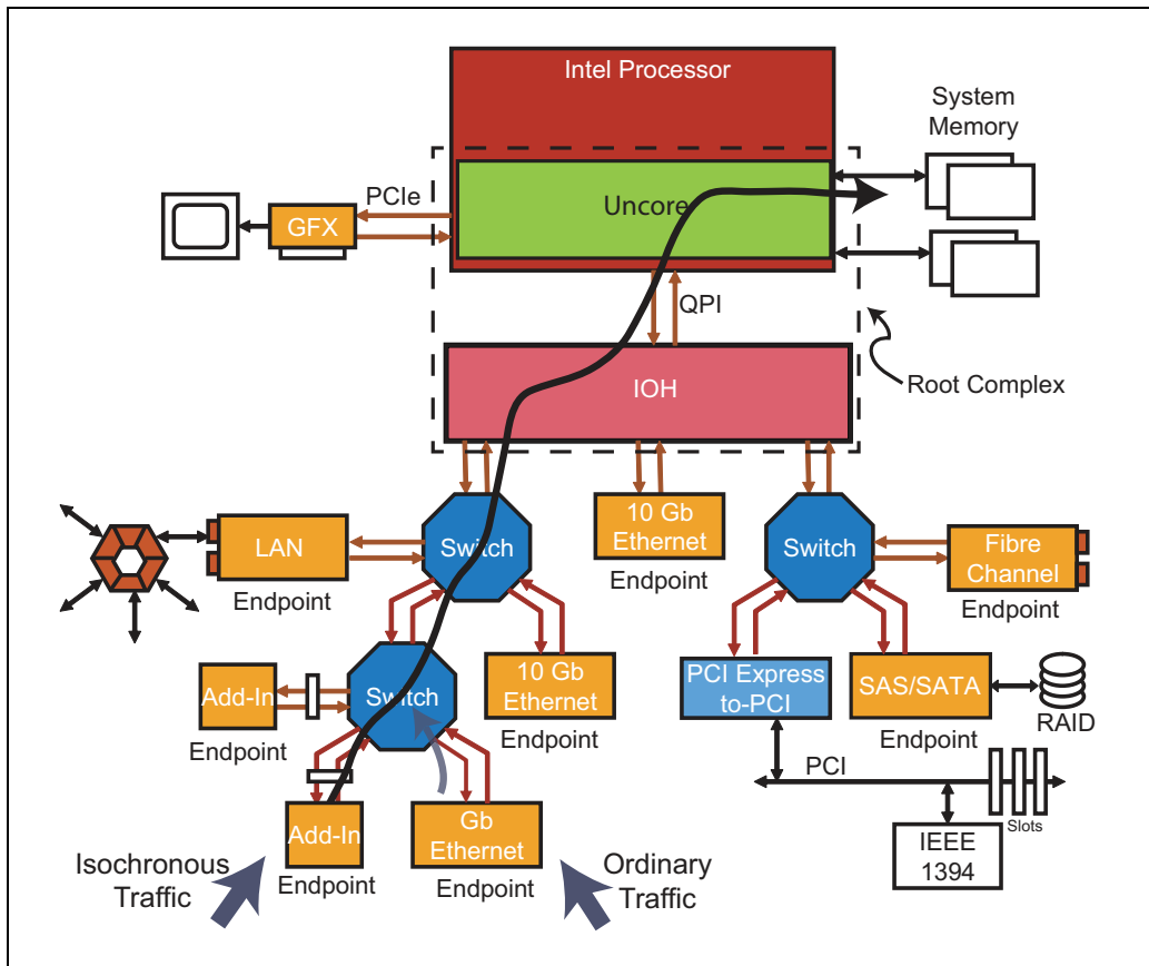
Figure 2-22: QoS Example
