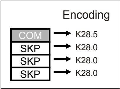
Figure 11-20: SKIP Ordered Set
