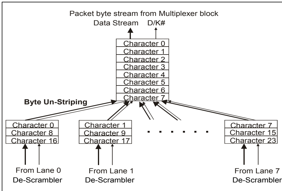
Figure 11-26: Example of x8 Byte Un-Striping
