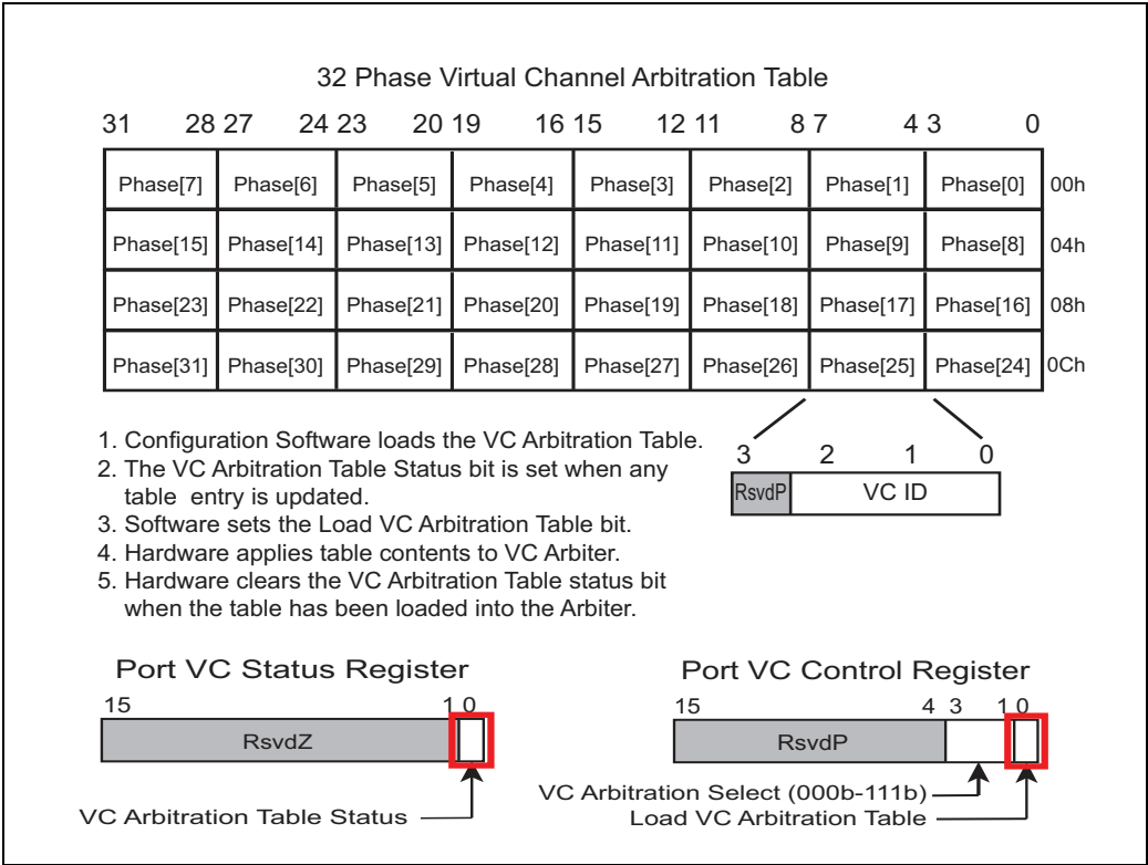
Figure 7-13: Loading the VC Arbitration Table Entries
