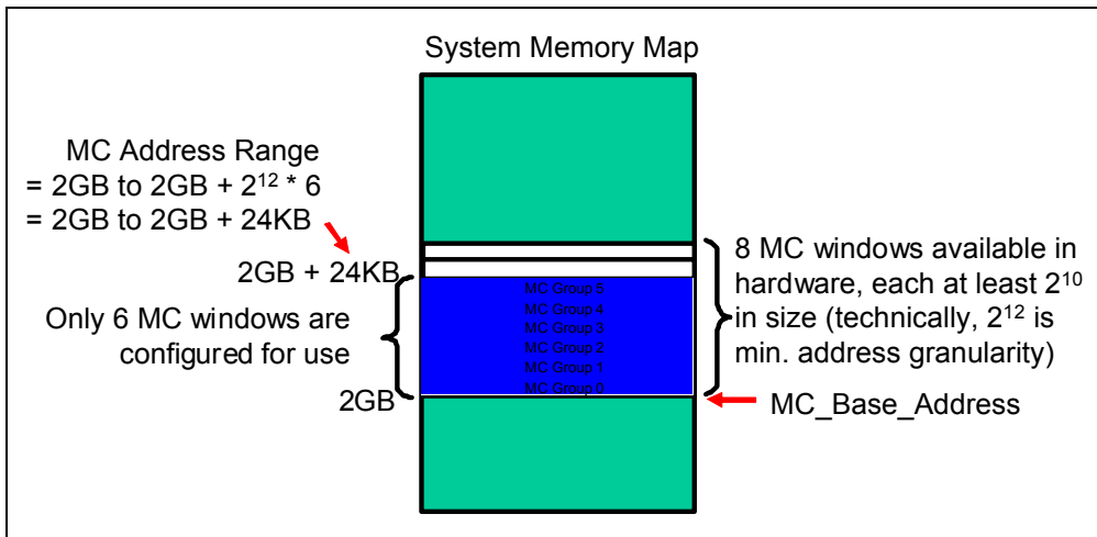
Figure 20-7: Multicast Address Example
