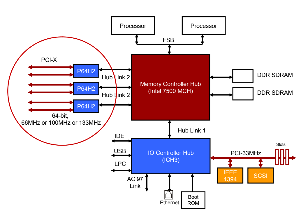
Figure 1-15: 66 MHz/133 MHz PCI-X Bus Based Platform
