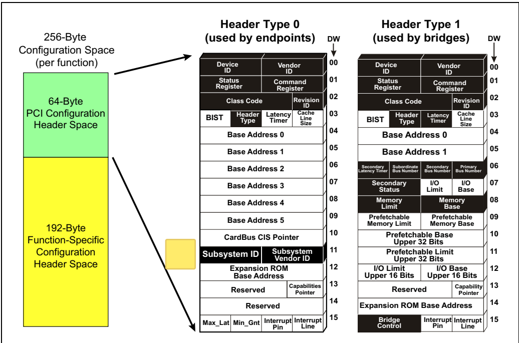
Figure 2-7: Configuration Headers
