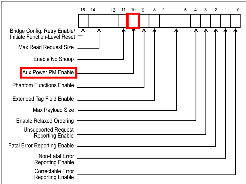
Figure 16-30: Auxiliary Current Enable for Devices Not Supporting PMEs
