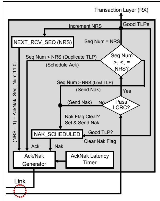
Figure 10-12: Ack/Nak Receiver Elements
