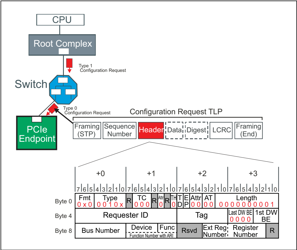
Figure 5-9: 3DW Configuration Request And Header Format
