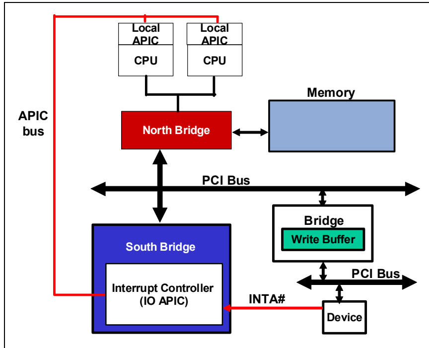
Figure 17-4: APIC Model for Interrupt Delivery
