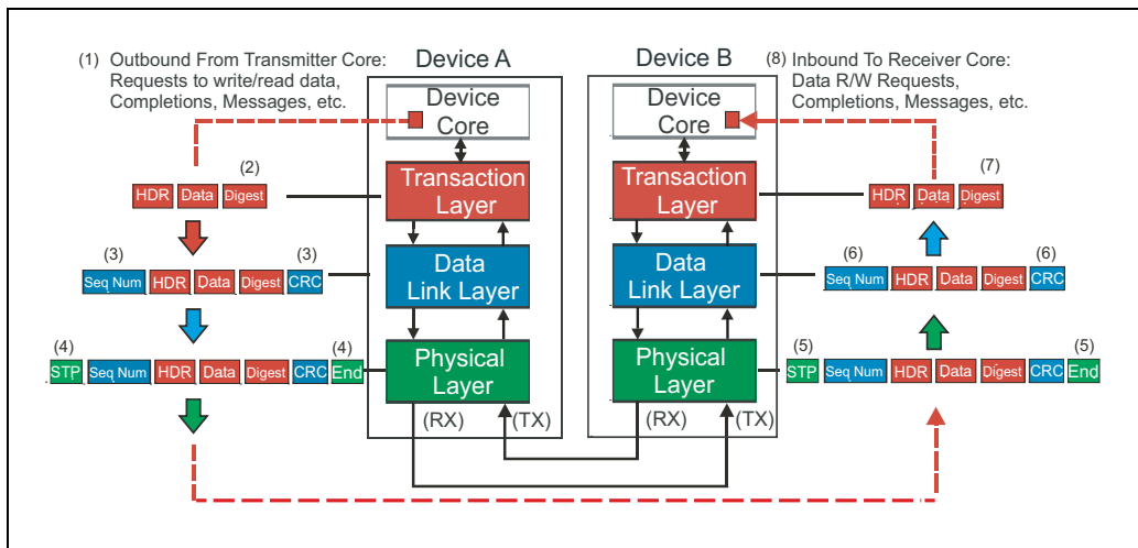
Figure 5-2: PCIe TLP Assembly/Disassembly
