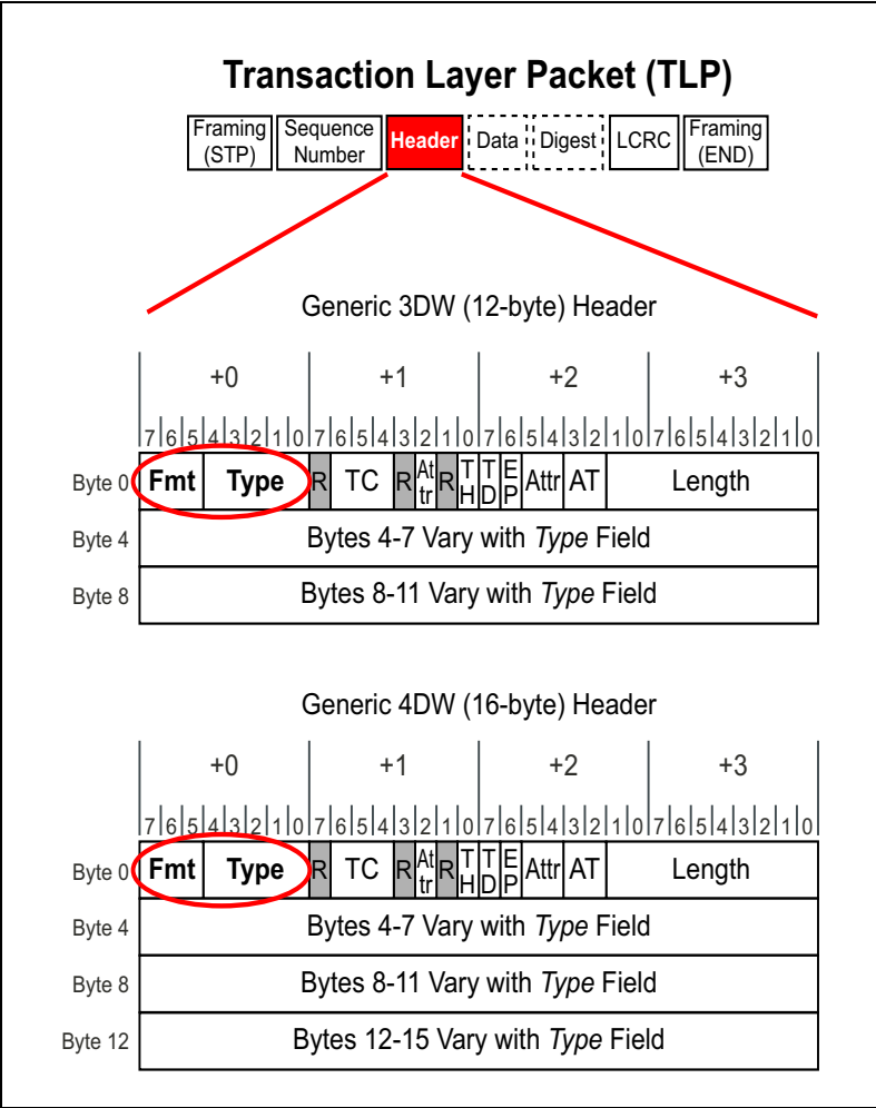
Figure 4-14: Transaction Layer Packet Generic 3DW And 4DW Headers
