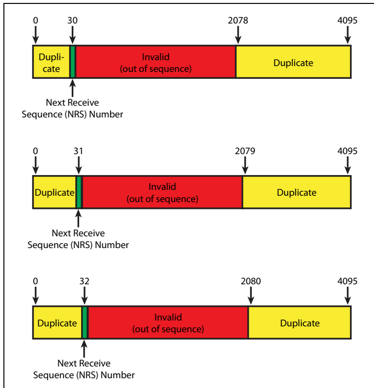
Figure 10-6: Examples of Sequence Number Ranges
