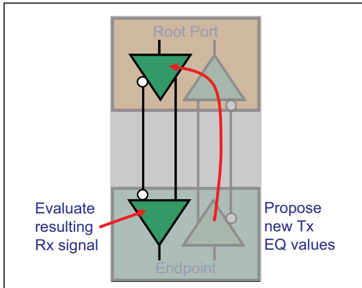
Figure 14-34: Equalization Process: Adjustments During Phase 2
