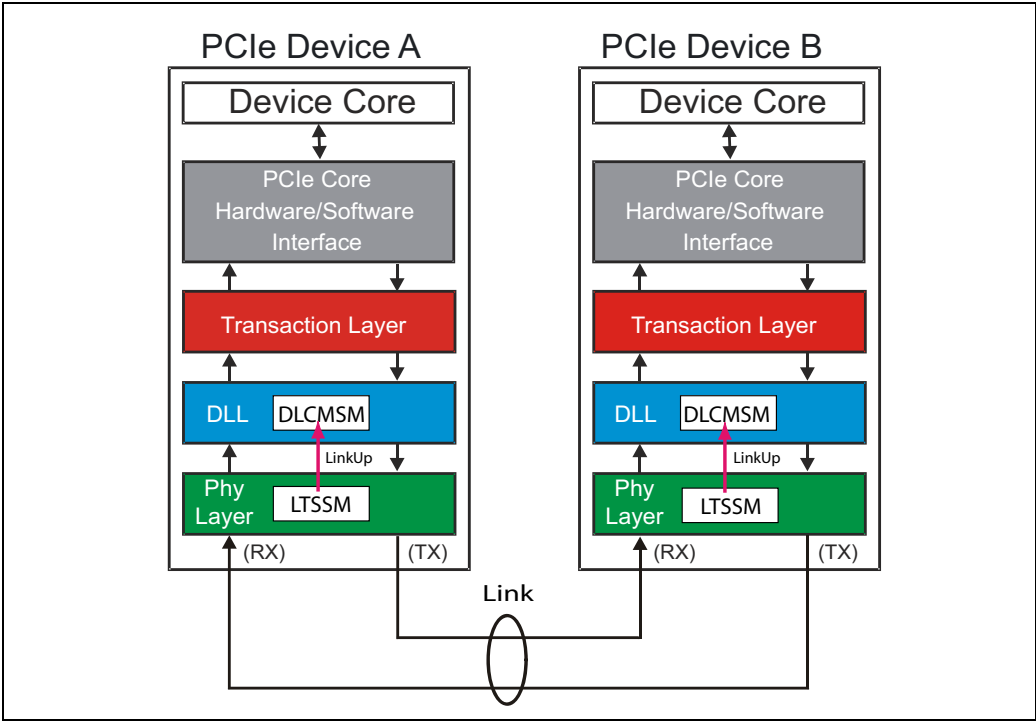
Figure 6-3: Physical Layer Reports That It's Ready
