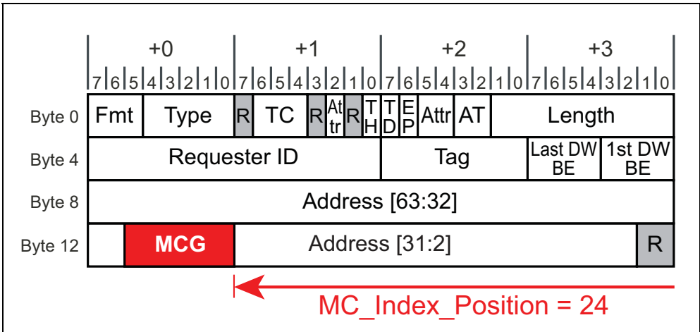
Figure 20-6: Position of Multicast Group Number
