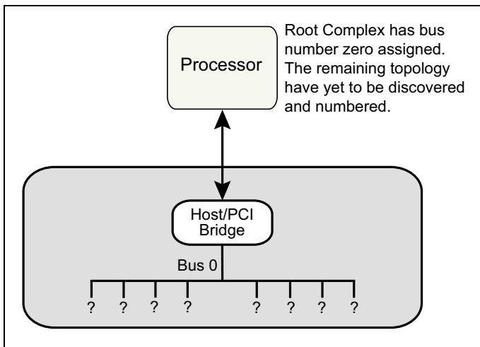
Figure 3-10: Topology View At Startup
