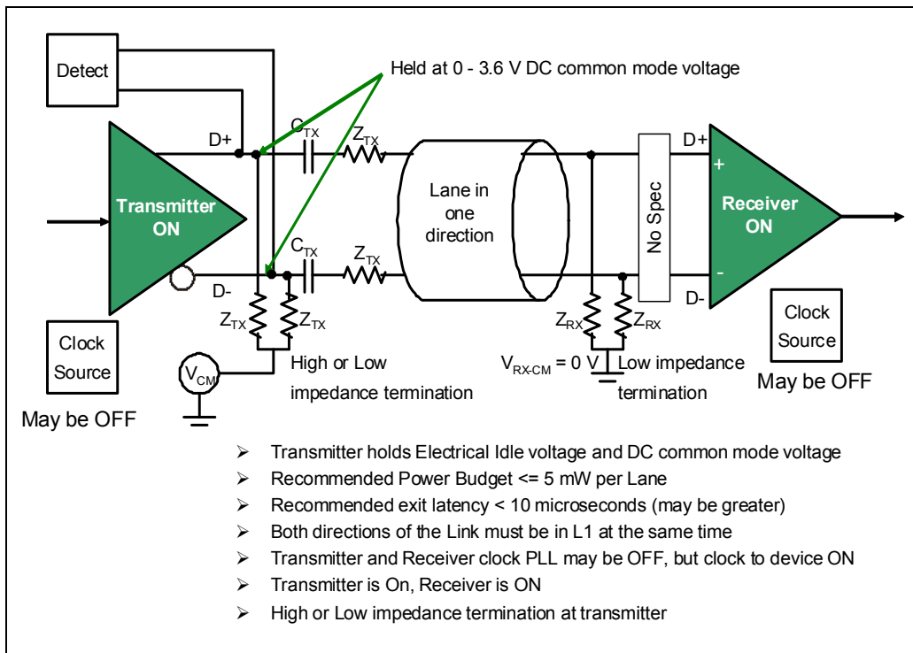
Figure 13-37: L1 Low Power Link State
