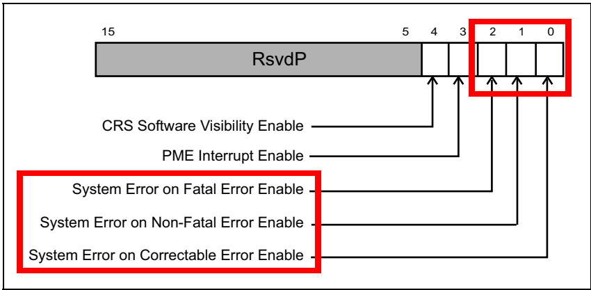
Figure 15-18: Root Control Register
