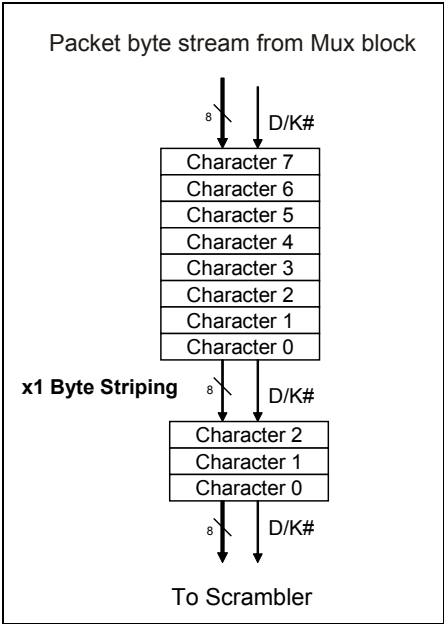
Figure 11-8: x1 Byte Striping
