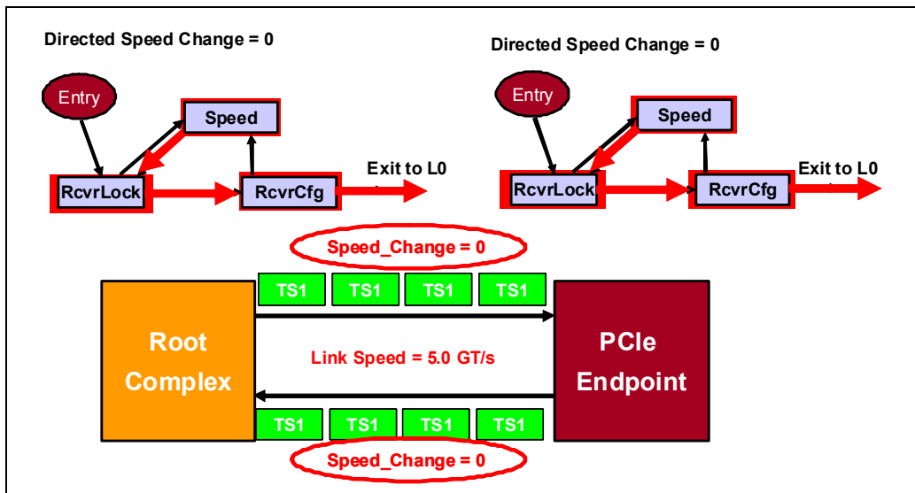
Figure 14-55: Speed Change Finish
