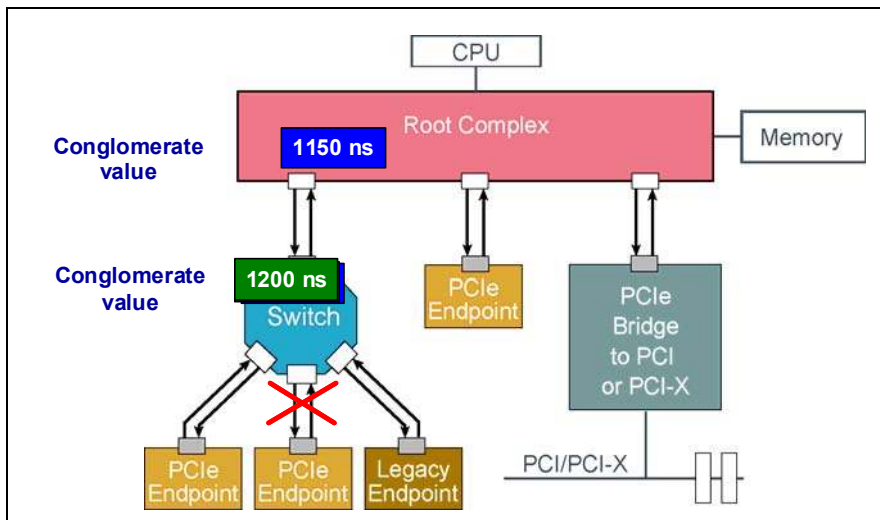
Figure 16-44: LTR - Link Down Case
