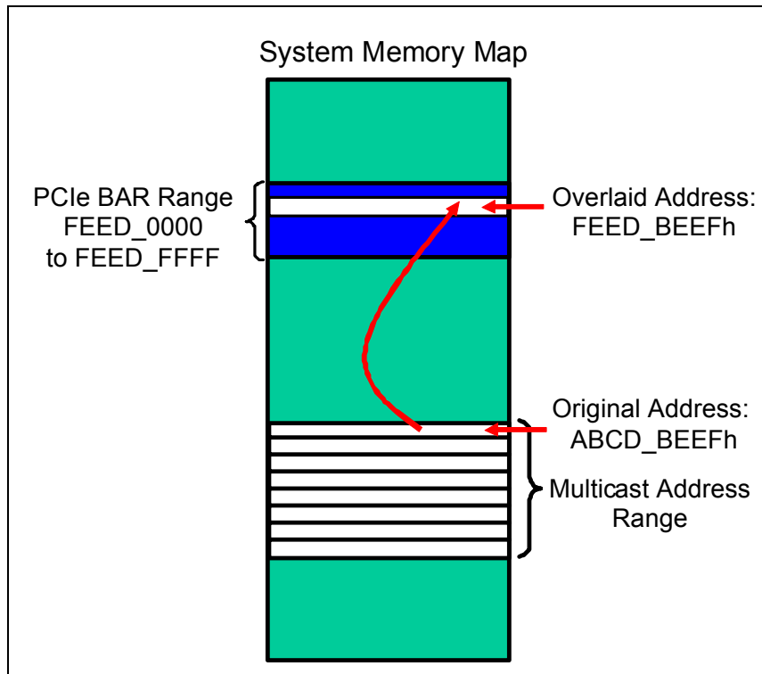
Figure 20-9: Overlay Example
