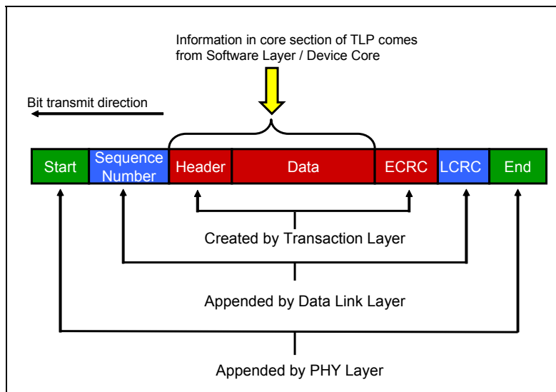
Figure 2-16: TLP Assembly
