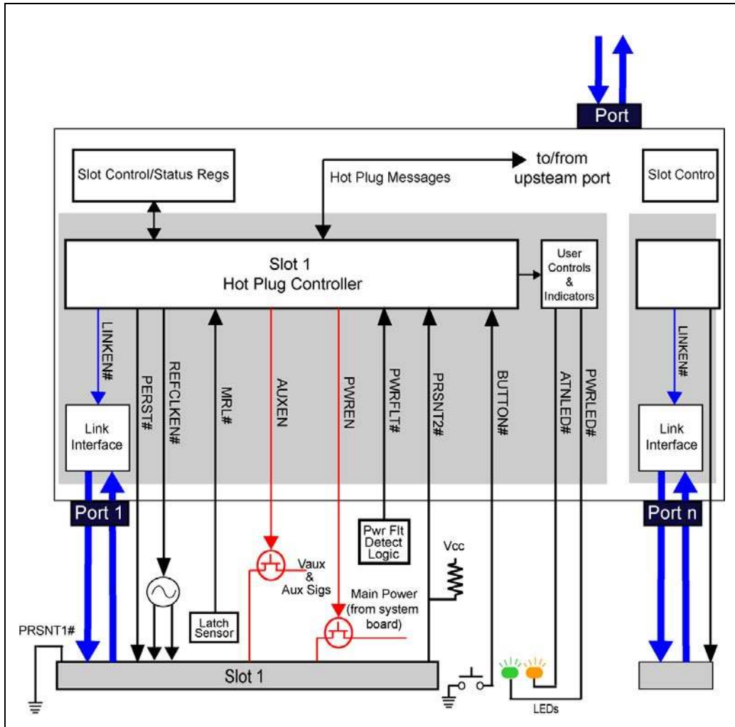
Figure 19-3: Hot Plug Control Functions within a Switch
