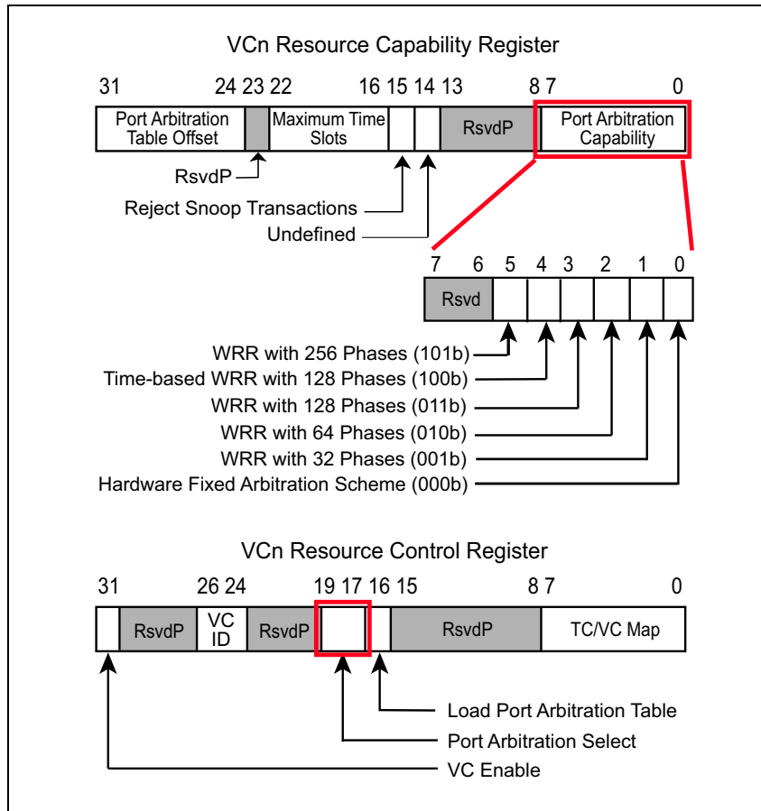
Figure 7-17: Software Selects Port Arbitration Scheme
