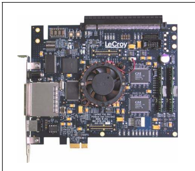
Figure A-14: LeCroy Gen2 Protocol Test Card (PTC)
