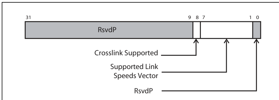
Figure 14-69: Link Capabilities 2 Register
