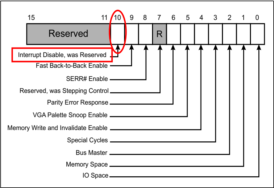
Figure 17-7: Configuration Command Register — Interrupt Disable Field
