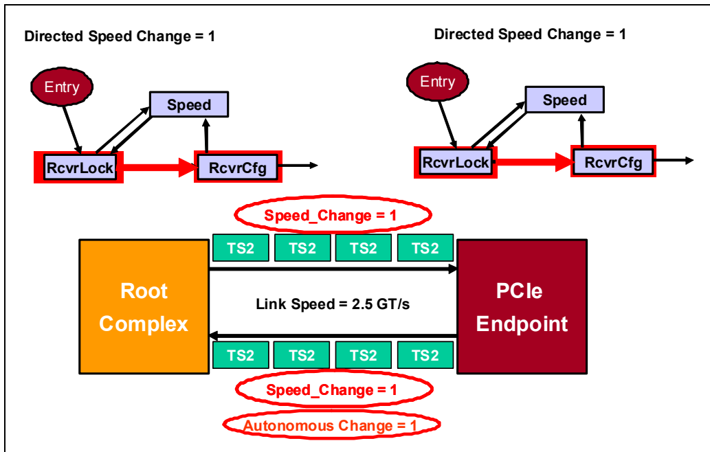
Figure 14-50: Speed Change - Part 2
