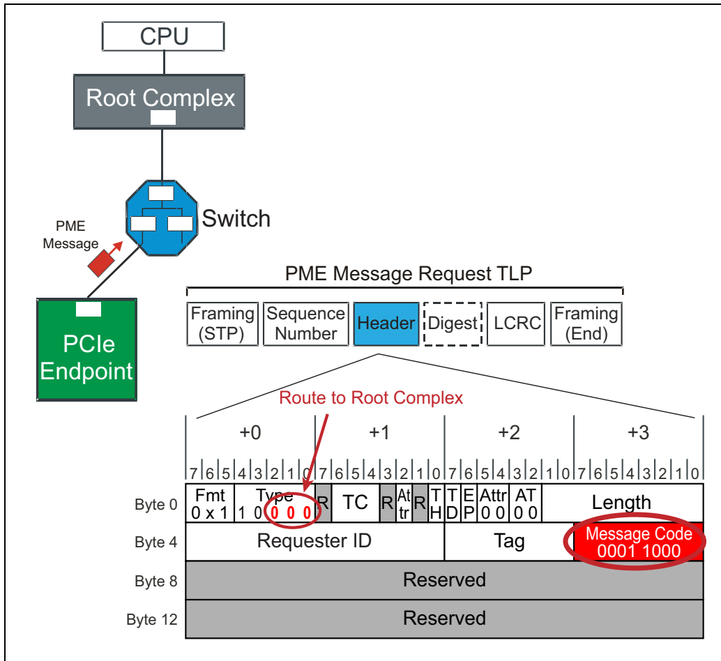
Figure 16-28: PME Message Format
