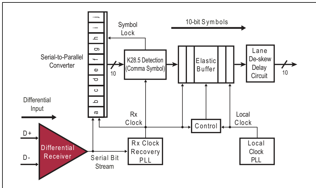
Figure 11-22: Receiver Logic's Front End Per Lane
