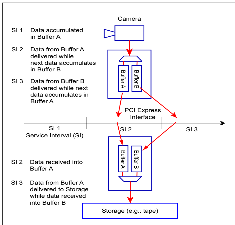
Figure 7-23: Example Application of Isochronous Transaction
