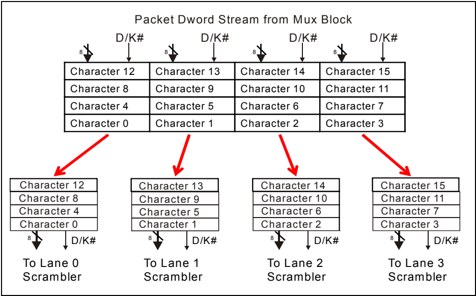
Figure 11-9: x4 Byte Striping
