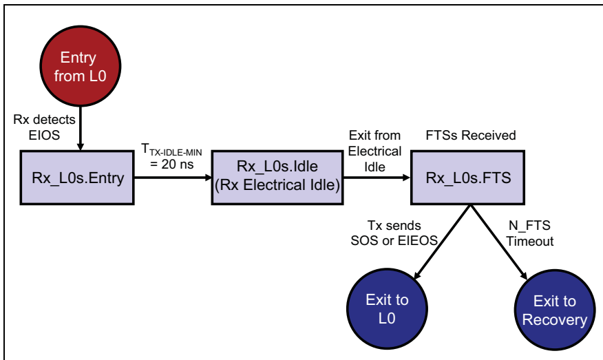
Figure 14-41: L0s Receiver State Machine
