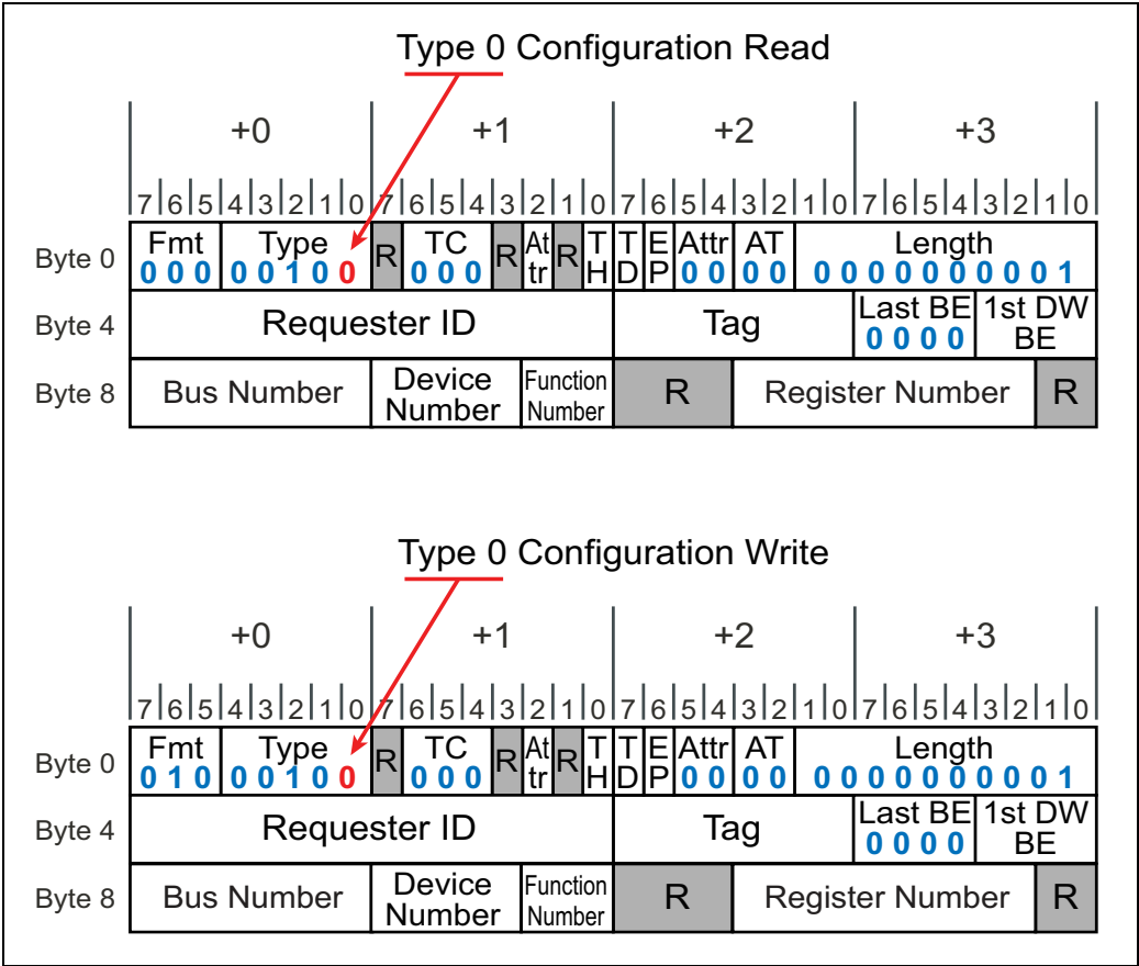
Figure 3-7: Type 0 Configuration Read and Write Request Headers
