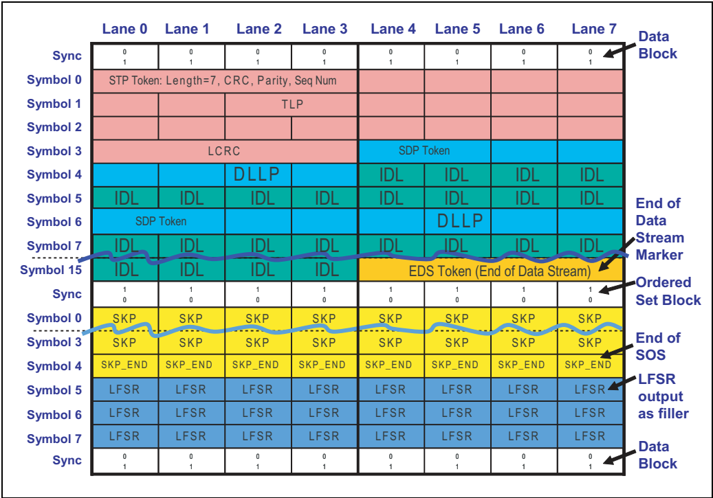
Figure 12-15: Gen3 x8 Skip Ordered Set (SOS) Example
