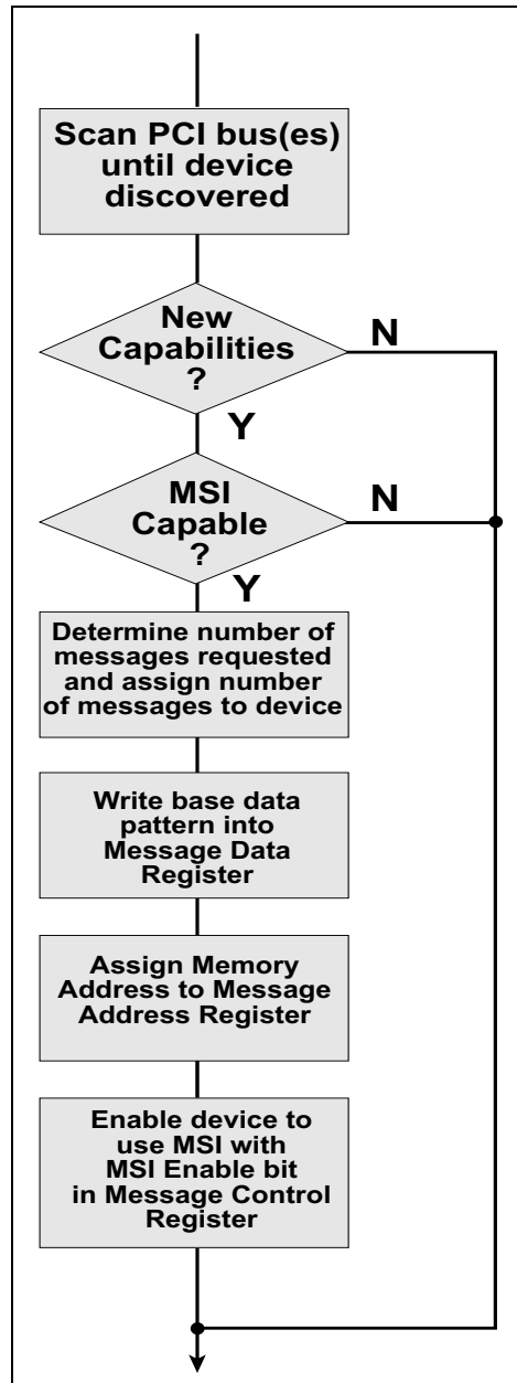
Figure 17-15: Device MSI Configuration Process
