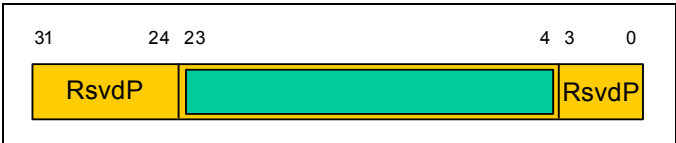
Figure 20-21: Resizable BAR Capability Register
