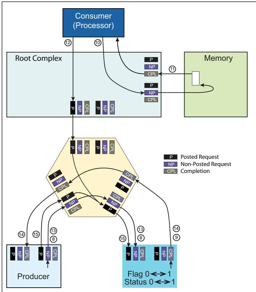
Figure 8-3: Producer/Consumer Sequence Example — Part 2
