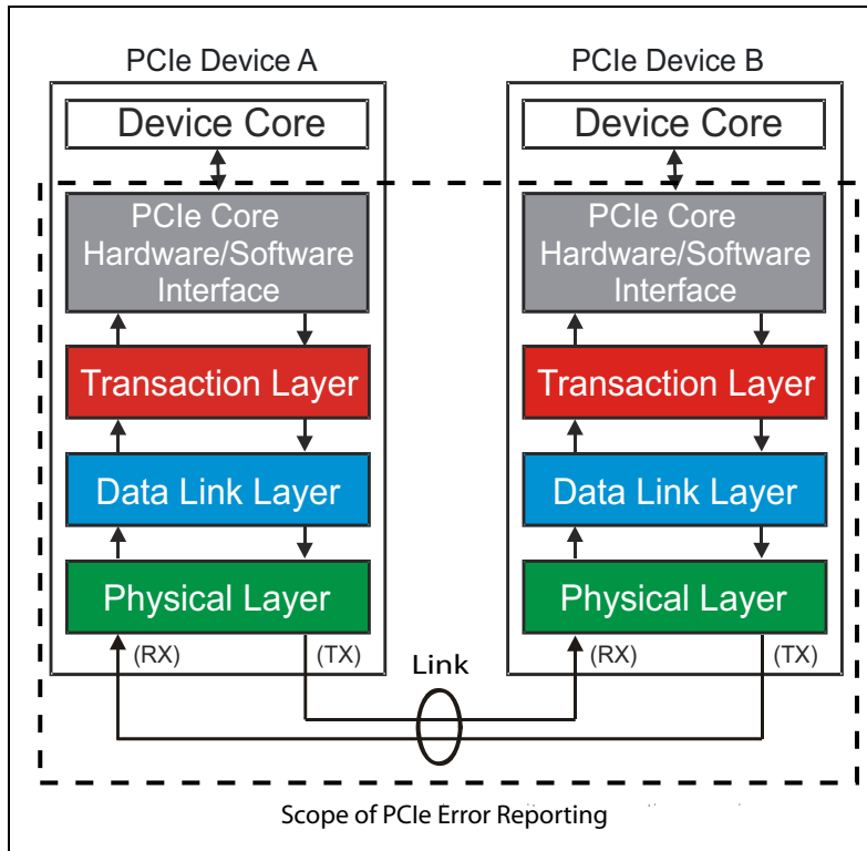
Figure 15-2: Scope of PCI Express Error Checking and Reporting
