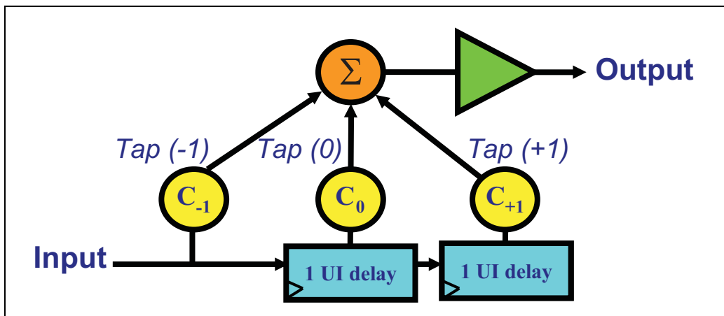
Figure 13-21: 3-Tap Tx Equalizer
