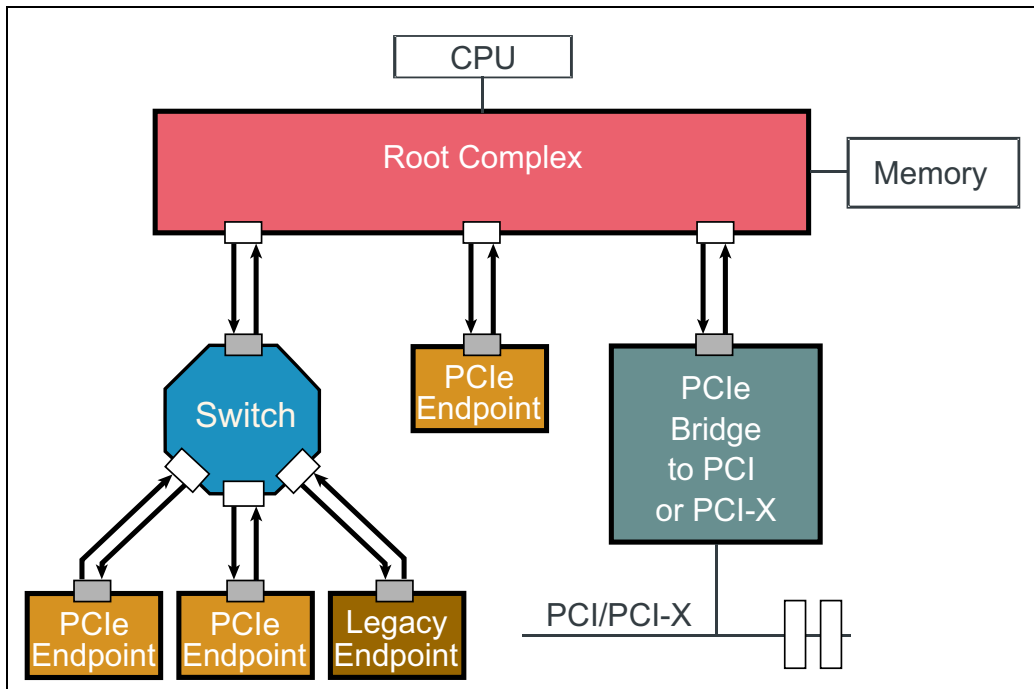
Figure 2-6: Example PCIe Topology
