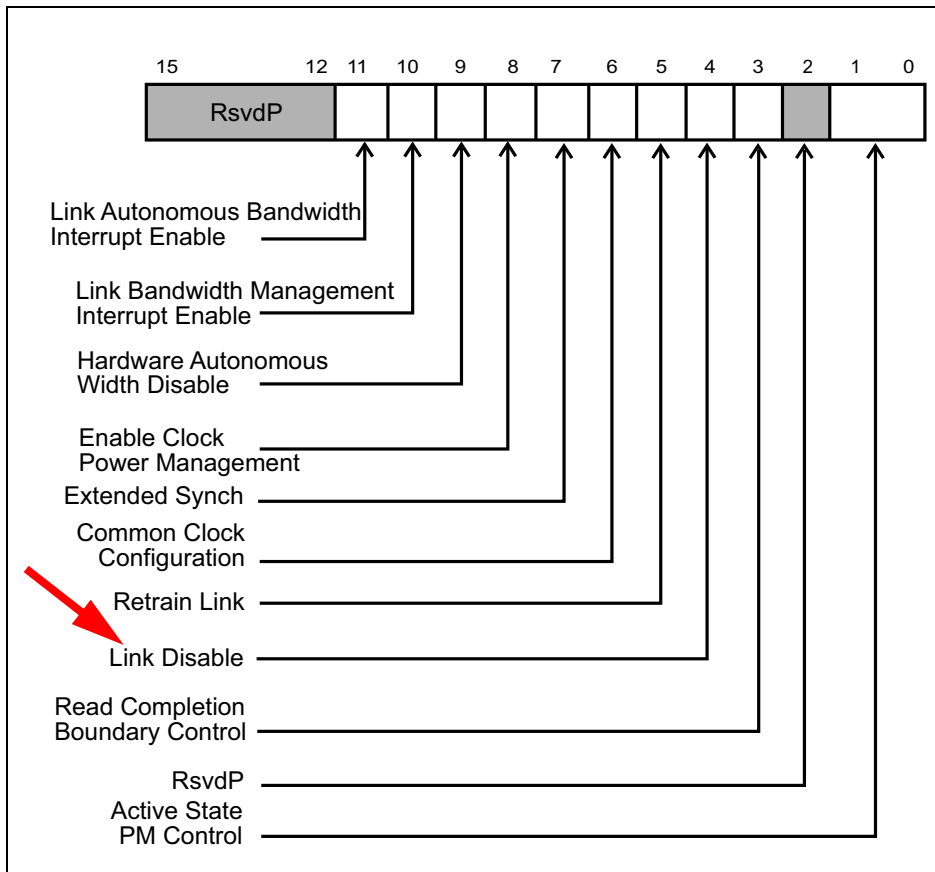
Figure 18-6: Link Control Register
