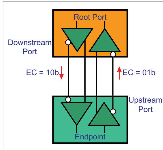
Figure 14-31: Equalization Process: Initiating Phase 2
