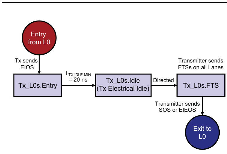
Figure 14-40: L0s Tx State Machine
