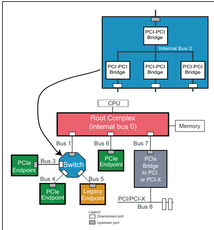
Figure 2-9: Example Results of System Enumeration
