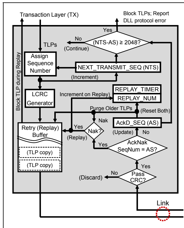
Figure 10-4: Transmitter Elements Associated with the Ack/Nak Protocol
