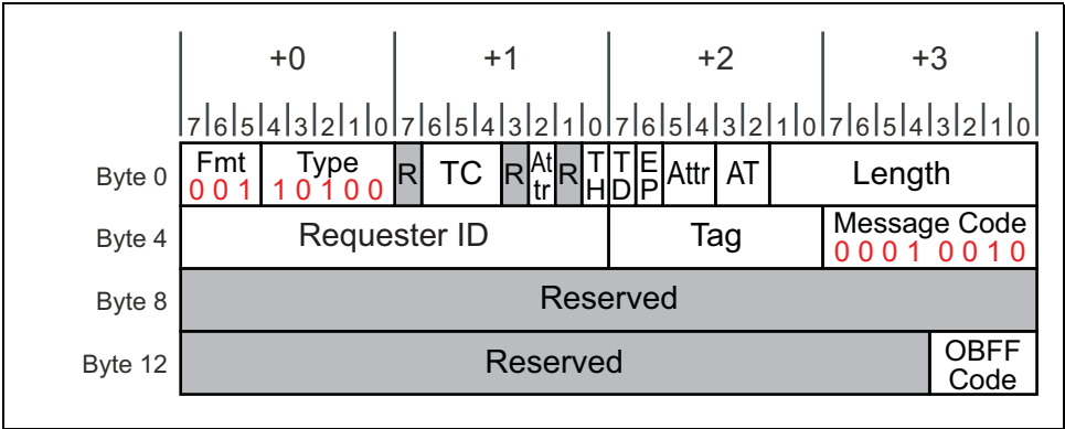
Figure 5-14: OBFF Message Header
