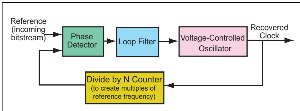
Figure 2-5: Simple PLL Block Diagram
