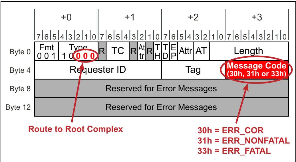
Figure 15-9: Error Message Format
