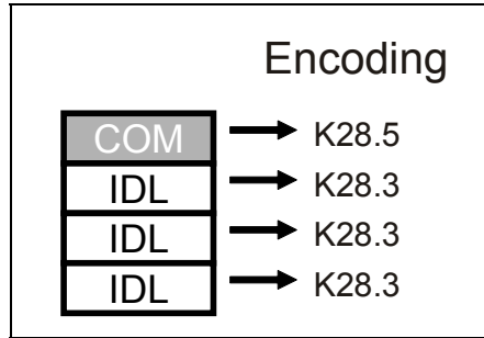
Figure 16-9: Gen1/Gen2 Mode EIOS Pattern
