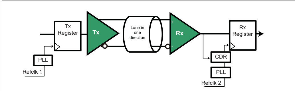
Figure 13-9: Separate Refclk Architecture
