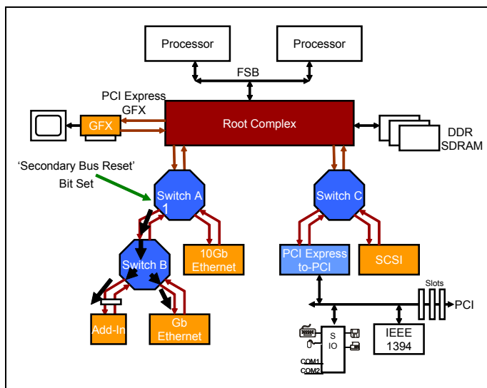
Figure 18-3: Switch Generates Hot Reset on One Downstream Port
