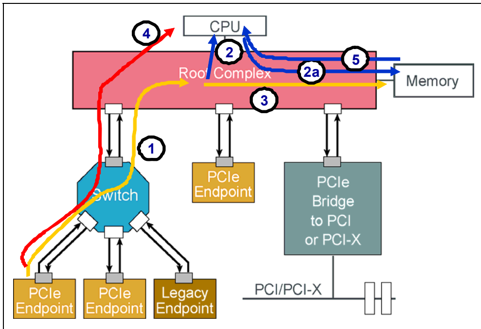
Figure 20-11: TPH Example
