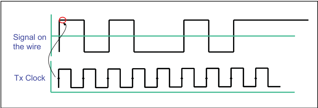
Figure 13-5: Signal Rate Less Than Half the Clock Rate
