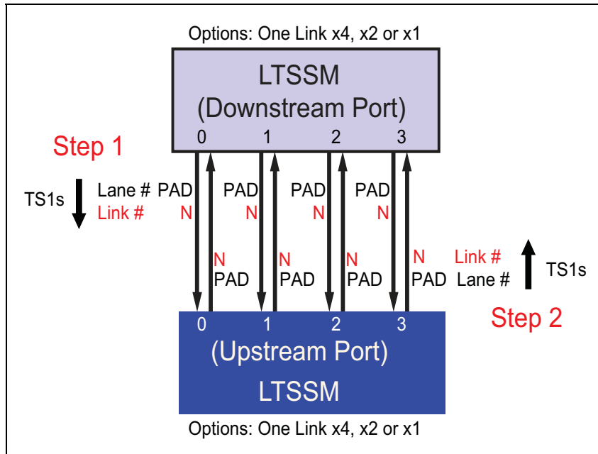
Figure 14-15: Example 1 - Steps 1 and 2
