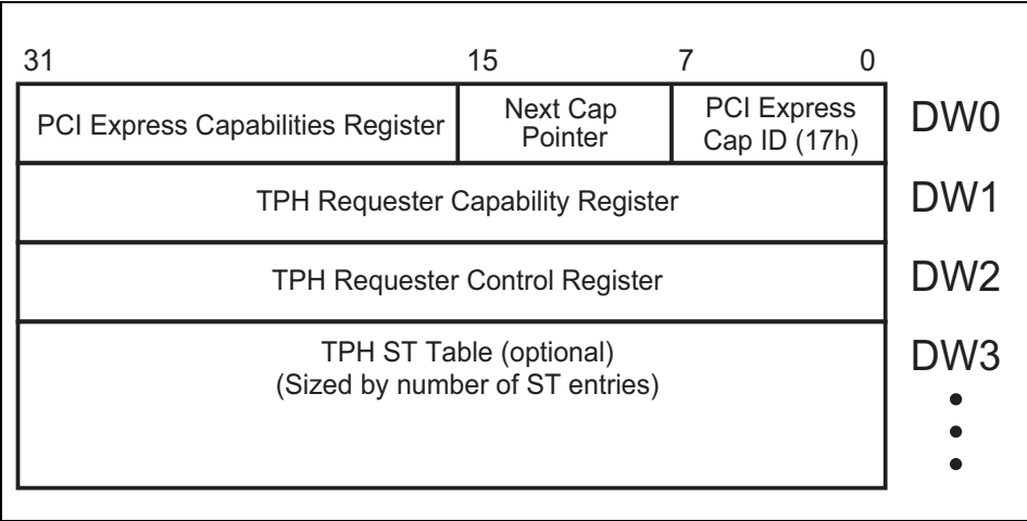
Figure 20-16: TPH Requester Capability Structure
