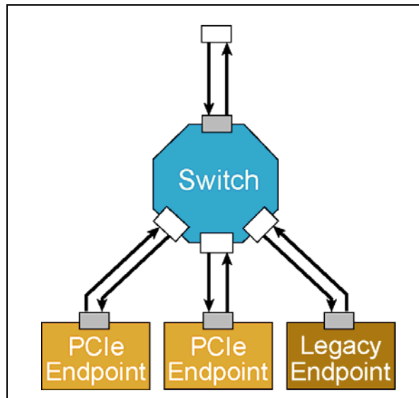
Figure 16-16: Only Upstream Ports Initiate L1 ASPM
