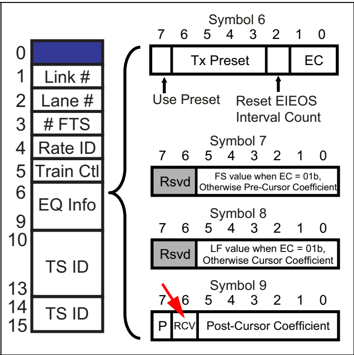
Figure 14-38: TS1s - Rejecting Coefficient Values
