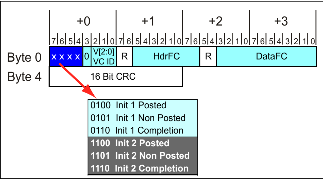
Figure 6-5: INIT1 Flow Control DLLP Format and Contents
