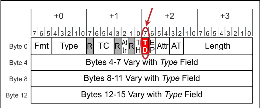
Figure 15-5: TLP Digest Bit in a Completion Header
