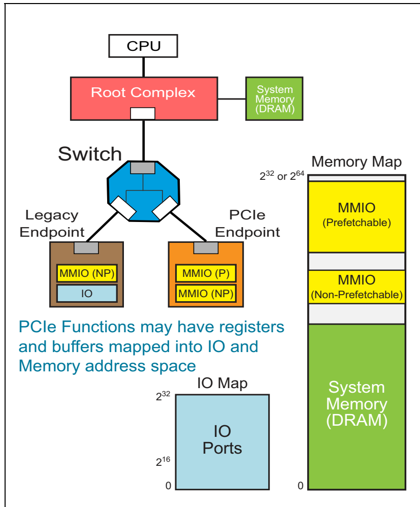
Figure 4-1: Generic Memory And IO Address Maps
