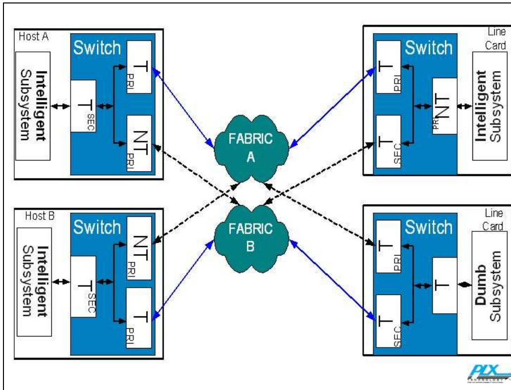
Figure 0-7: Dual-Star Fabric
