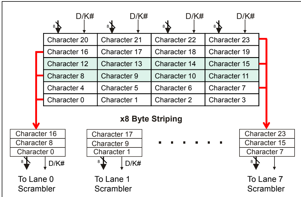
Figure 11-10: x8 Byte Striping with DWord Parallel Data
