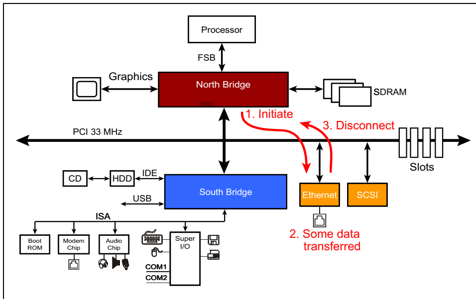
Figure 1-8: PCI Transaction Disconnect Mechanism
